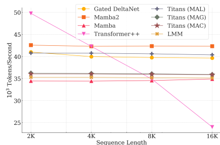
Figure 9: Training throughput comparison of Titans and baselines.
