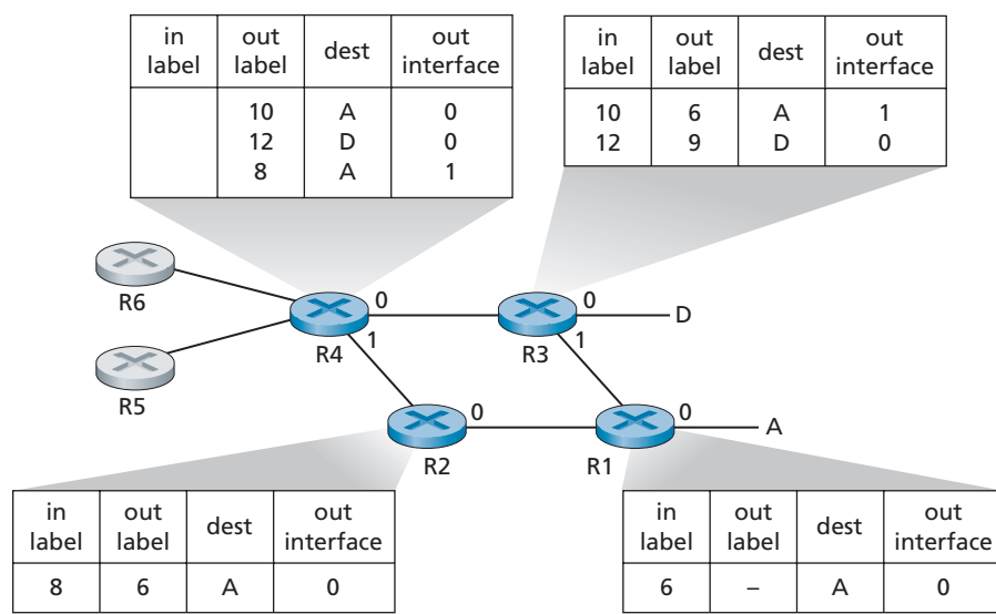
Figure 6.29 ♦ MPLS-enhanced forwarding
