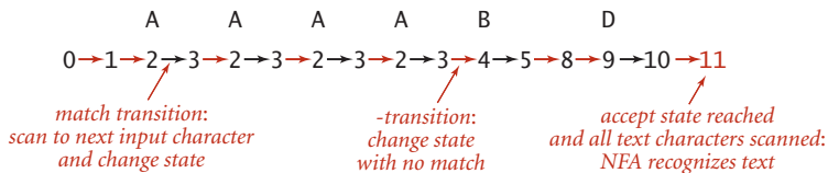
Finding a pattern with ( A | A C ) D ) NFA
