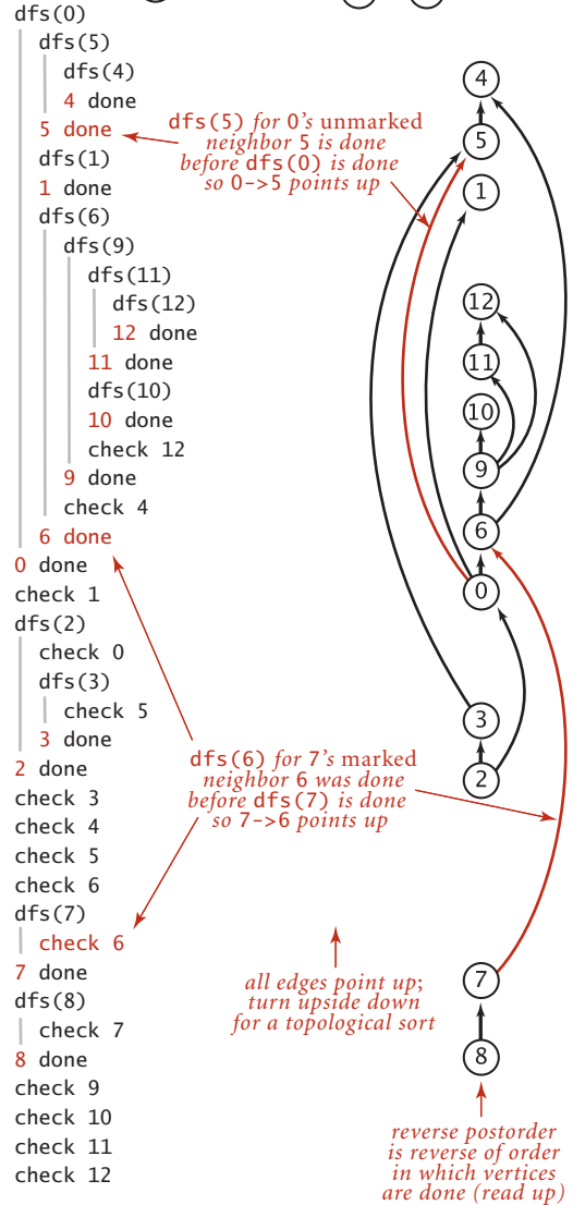
Reverse postorder in a DAG is a topological sort
