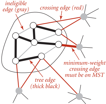
Prim's MST algorithm
