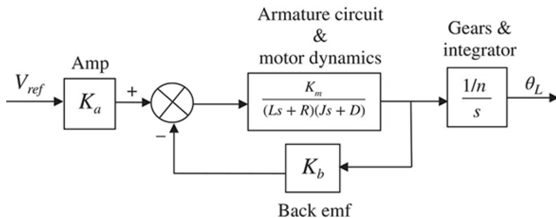
FIGURE P8.35 Open-loop model for ARM II
