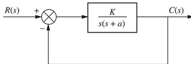
FIGURE 5.14 Second-order feedback control system
