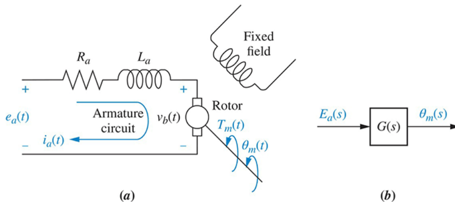
FIGURE 2.35 DC motor: a. schematic; 12 b. block diagram
