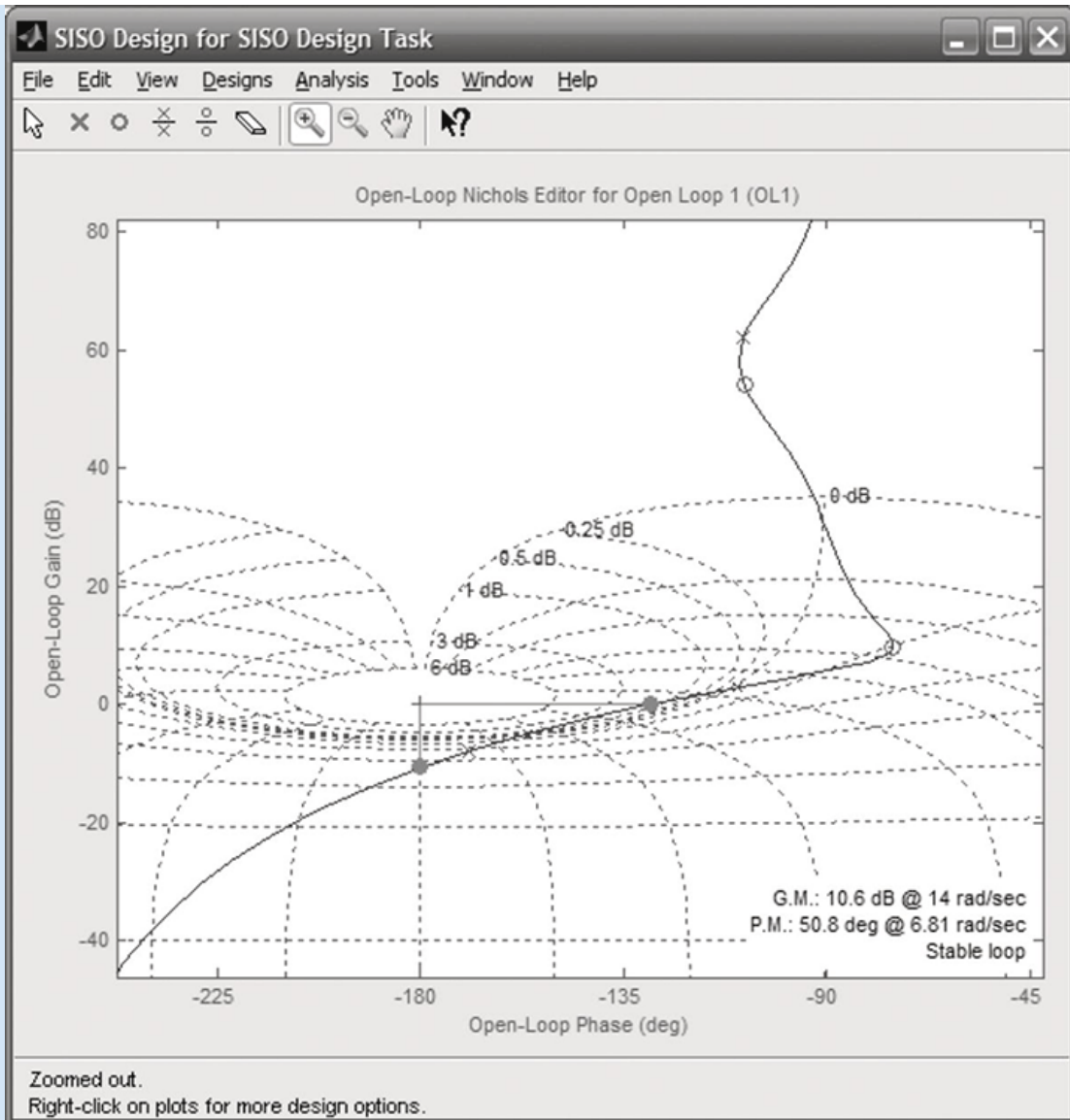
FIGURE 11.15 Nichols chart after lag-lead compensation
