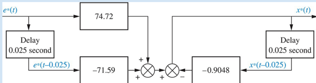
FIGURE 13.36 Flowchart for a digital lead compensator 9
