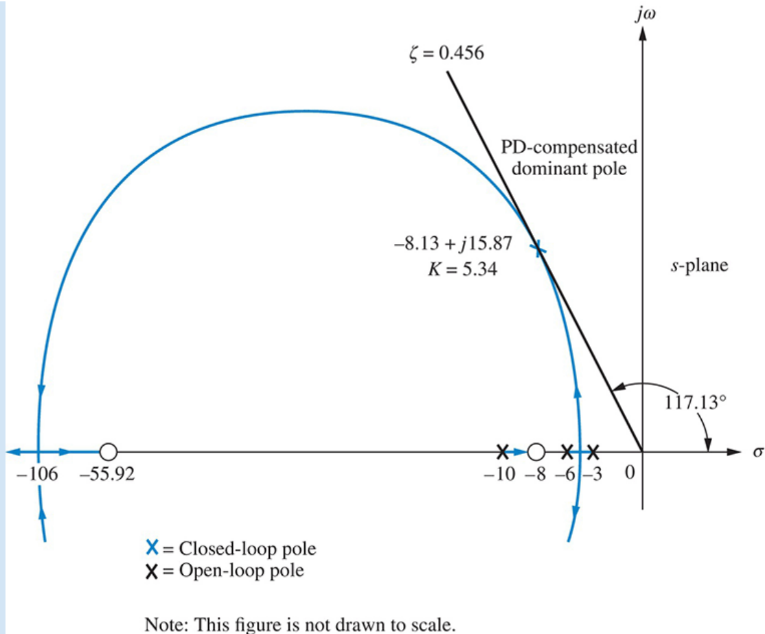
FIGURE 9.34 Root locus for PD-compensated system of Example 9.5
