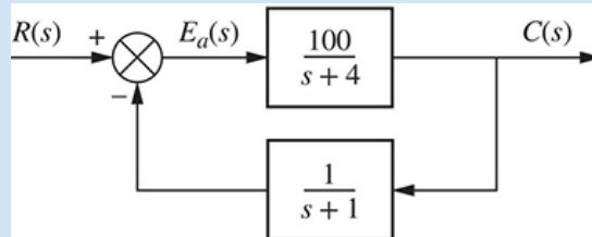
FIGURE 7.18 Nonunity-feedback system for Skill-Assessment Exercise 7.5
