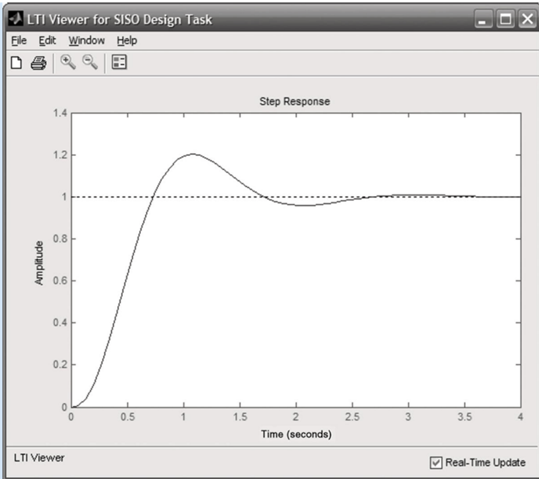
FIGURE 11.14 Gain-adjusted closed-loop step response
