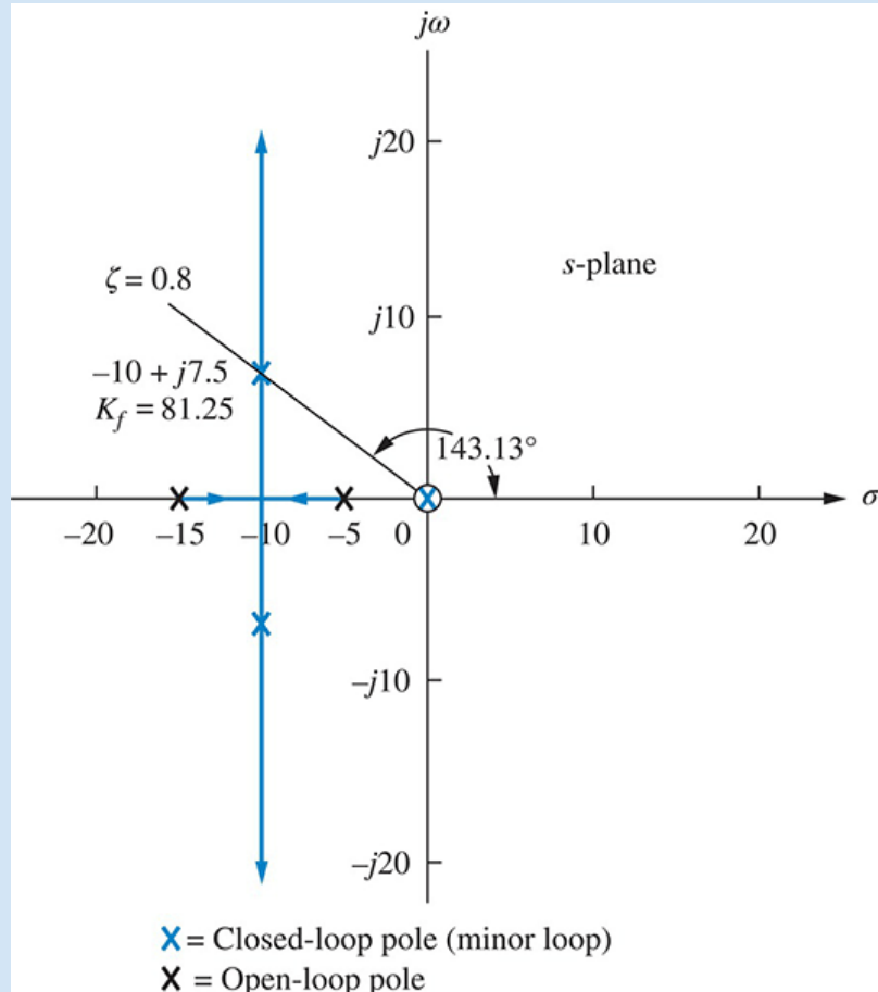
FIGURE 9.56 Root locus for minor loop of Example 9.8
