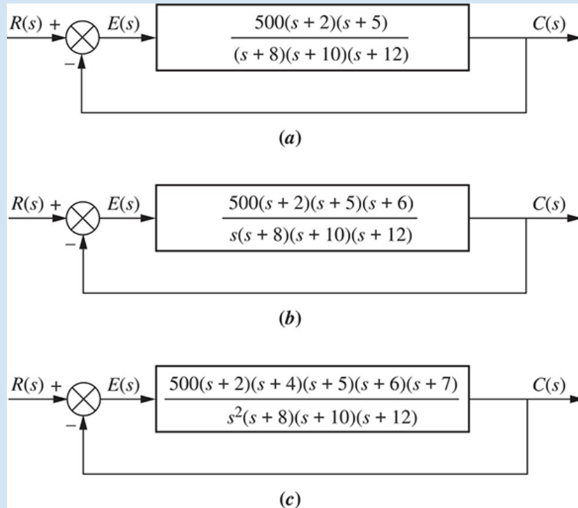
FIGURE 7.7 Feedback control systems for Example 7.4 .
