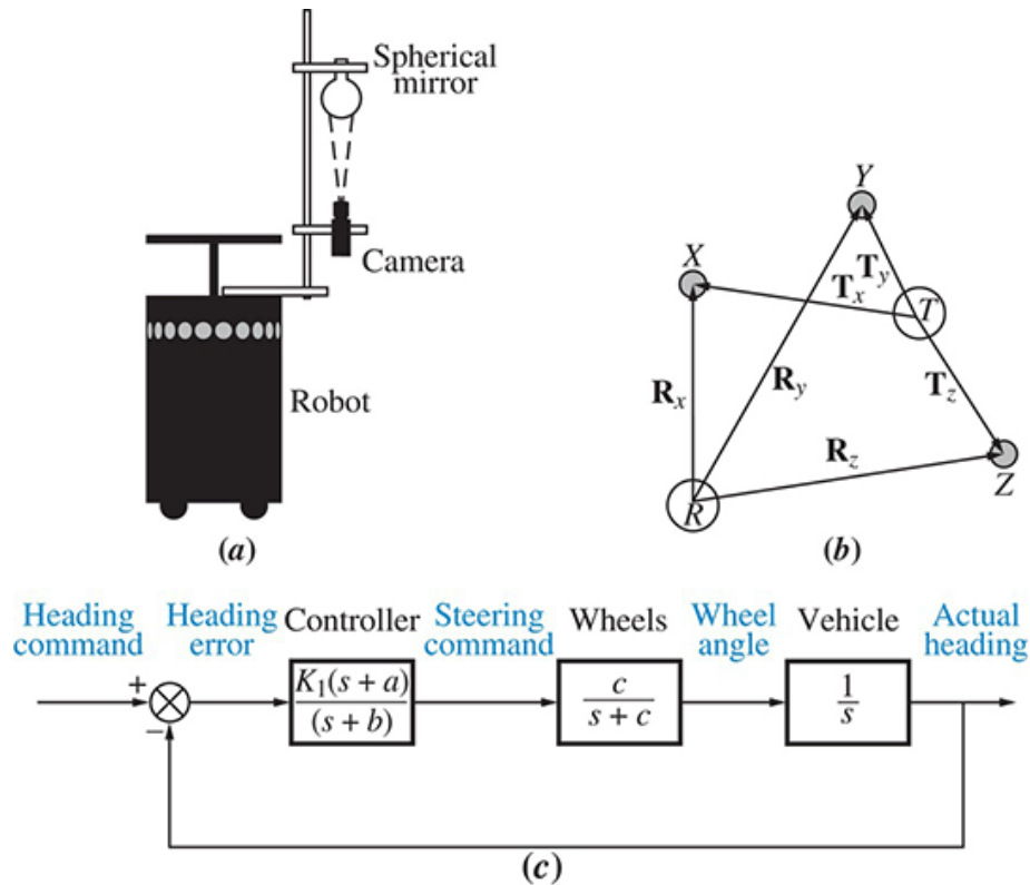
FIGURE P3.11 a. Robot with television imaging system; 1 b. vector diagram showing concept behind image-based homing; 1 c. heading control system
