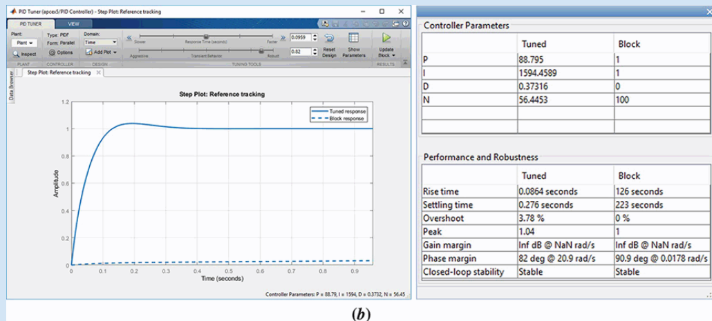
FIGURE C.21 PID Tuner window: a. before additional tuning; b. after additional tuning
