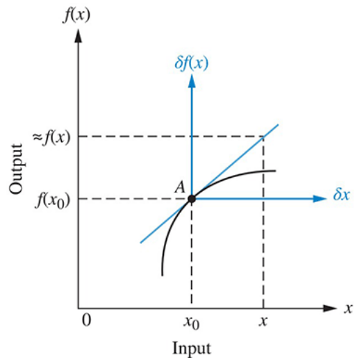
FIGURE 2.47 Linearization about point A
