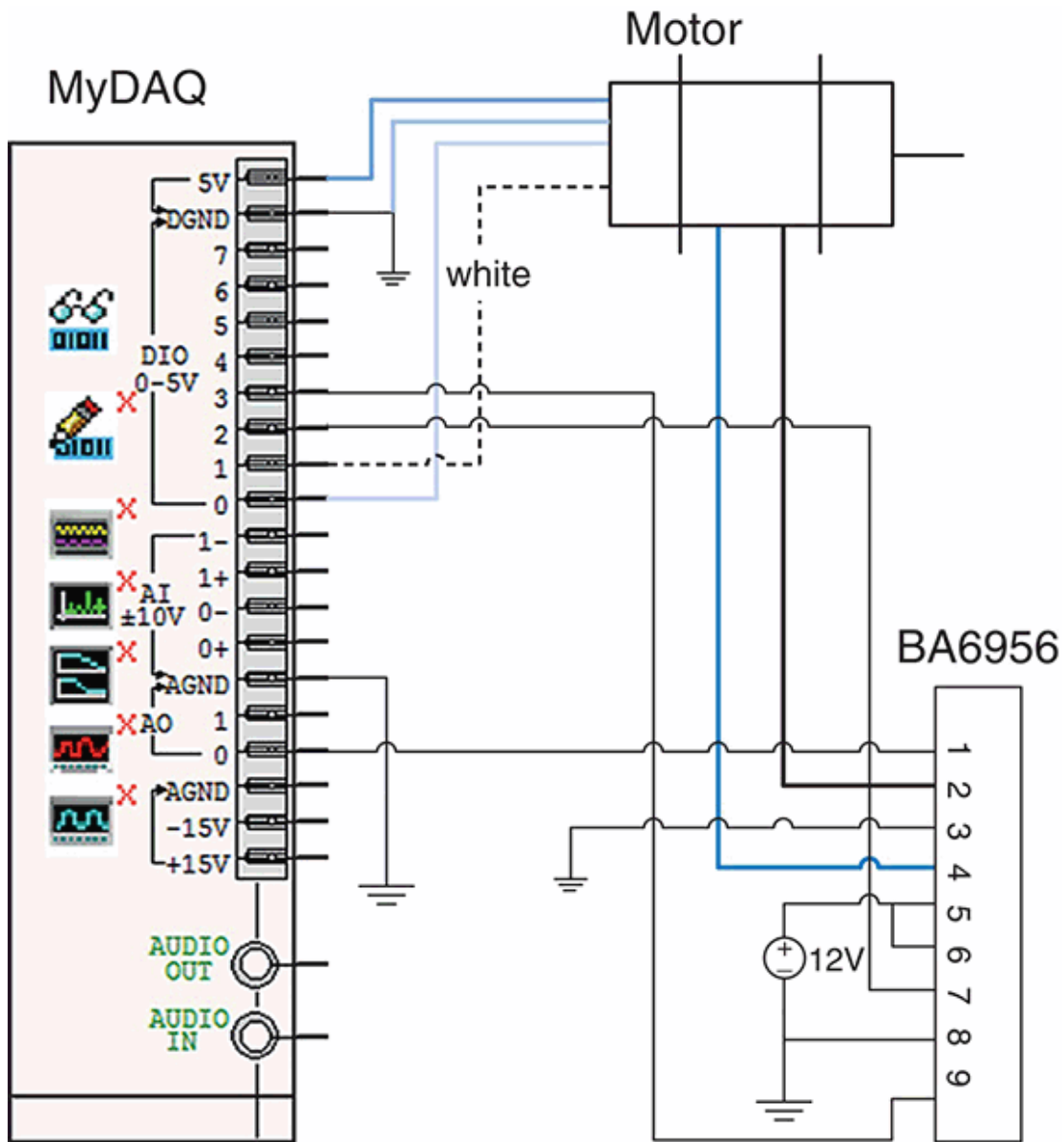
FIGURE P8.39 Wiring diagram 3
