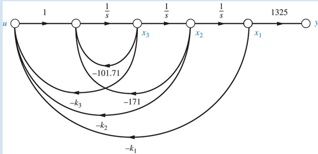
FIGURE 12.25 Plant with state-variable feedback for controller design
