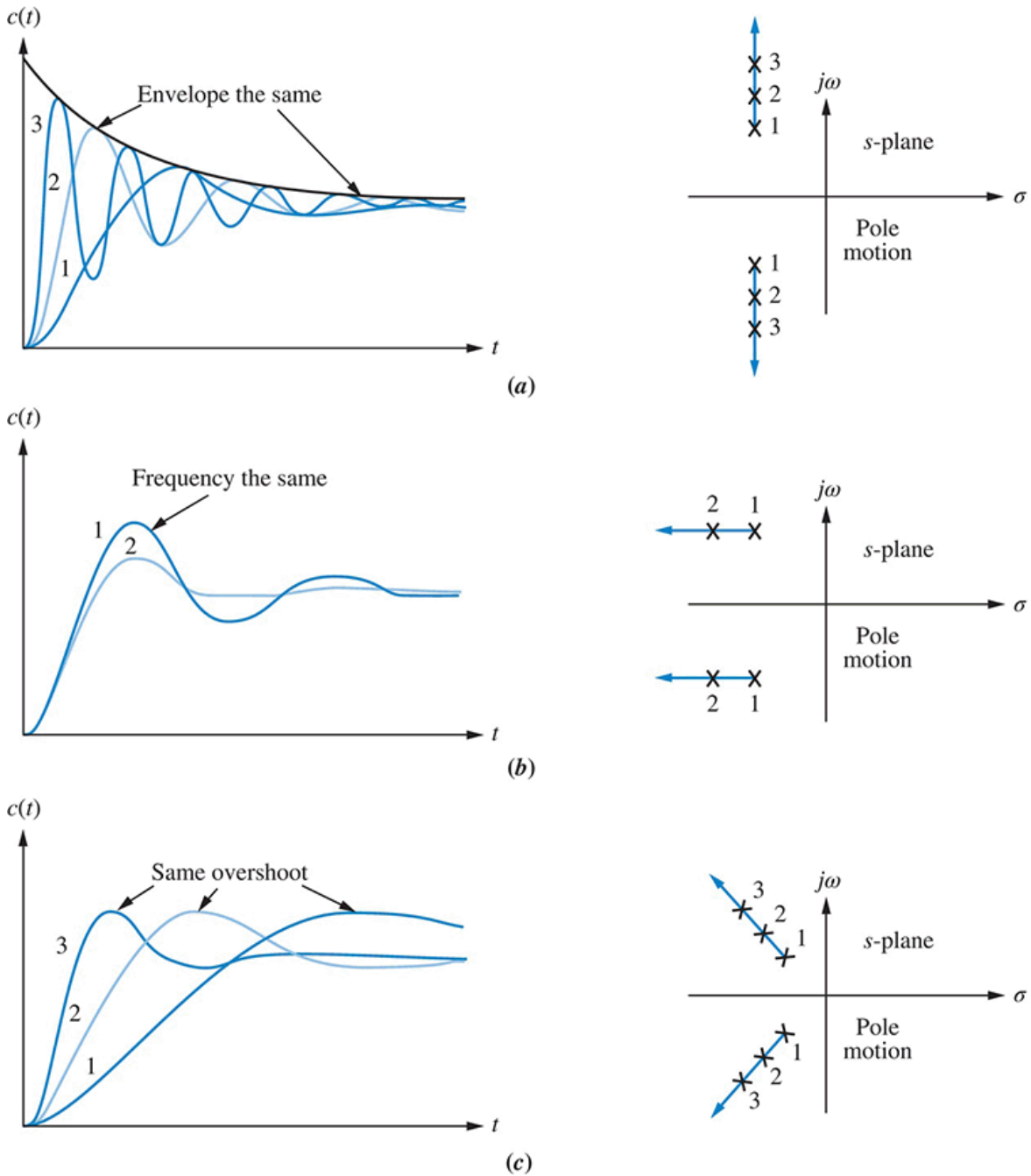
FIGURE 4.19 Step responses of second-order underdamped systems as poles move: a. with constant real part; b. with constant imaginary part; c. with constant damping ratio
