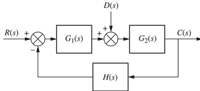
FIGURE 7.17 Nonunity-feedback control system with disturbance
