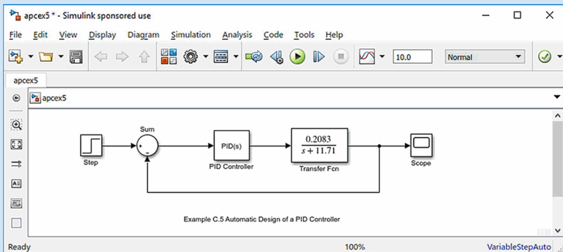
FIGURE C.19 Simulink block diagram for automated design of a PID controller
