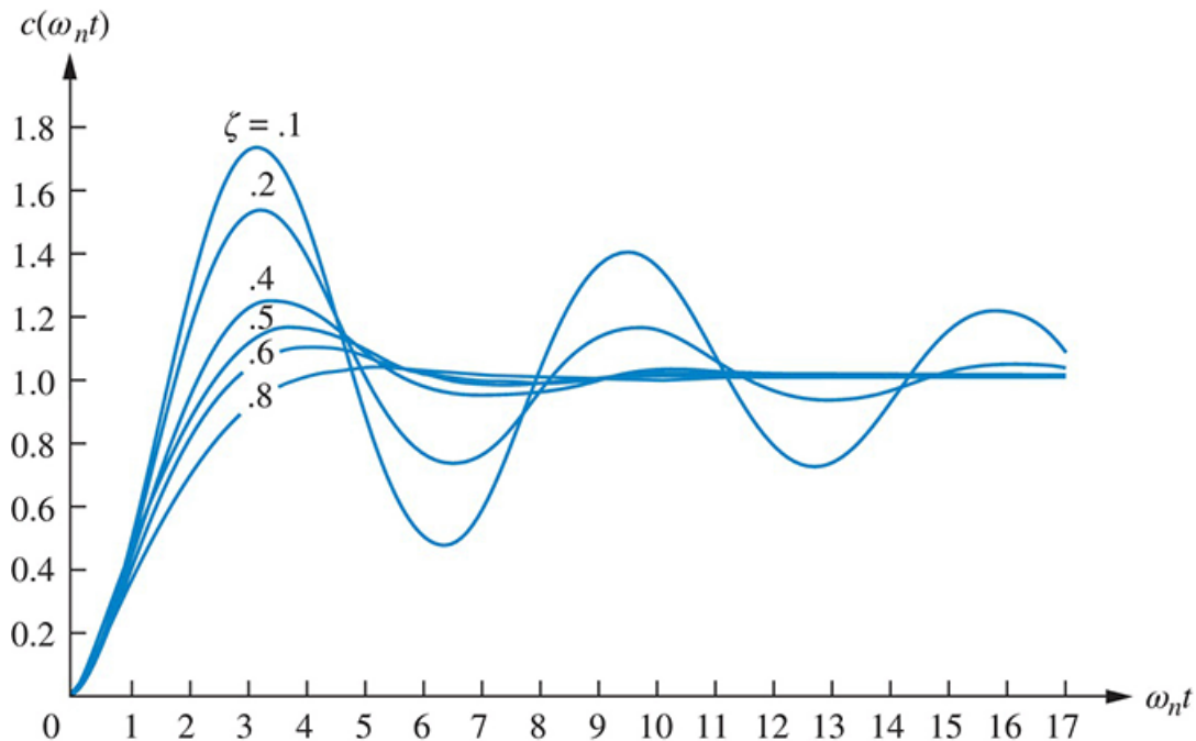
FIGURE 4.13 Second-order underdamped responses for damping ratio values
