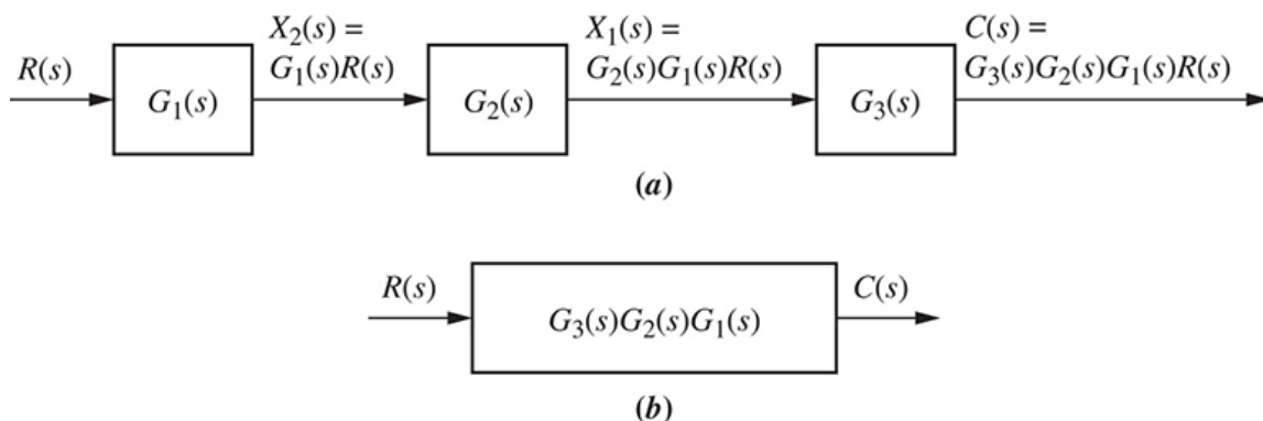
FIGURE 5.3 a. Cascaded subsystems; b. equivalent transfer function
