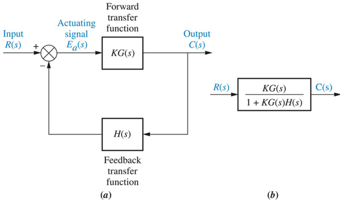
FIGURE 8.1 a. Closed-loop system; b. equivalent transfer function
