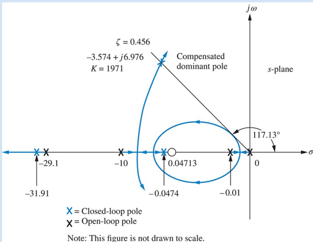
FIGURE 9.41 Root locus for lag-lead-compensated system of Example 9.6
