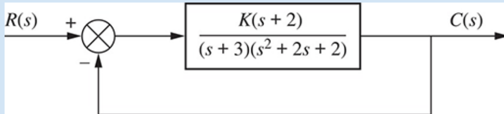
FIGURE 8.16 Unity-feedback system with complex poles
