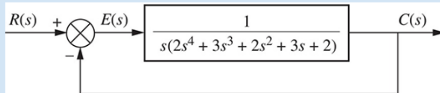
FIGURE 6.7 Feedback control system for Example 6.7
