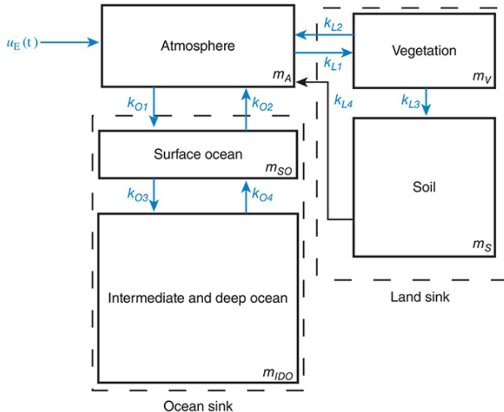
FIGURE P3.14 Global carbon cycle 4
