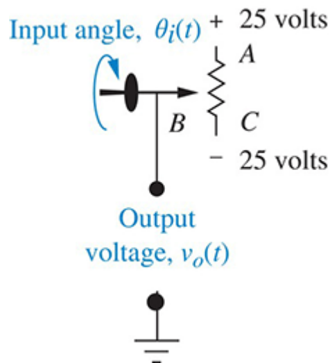
FIGURE P1.1 Potentiometer
