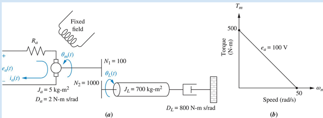
FIGURE 2.39 a. DC motor and load; b. torque–speed curve; c. block diagram
