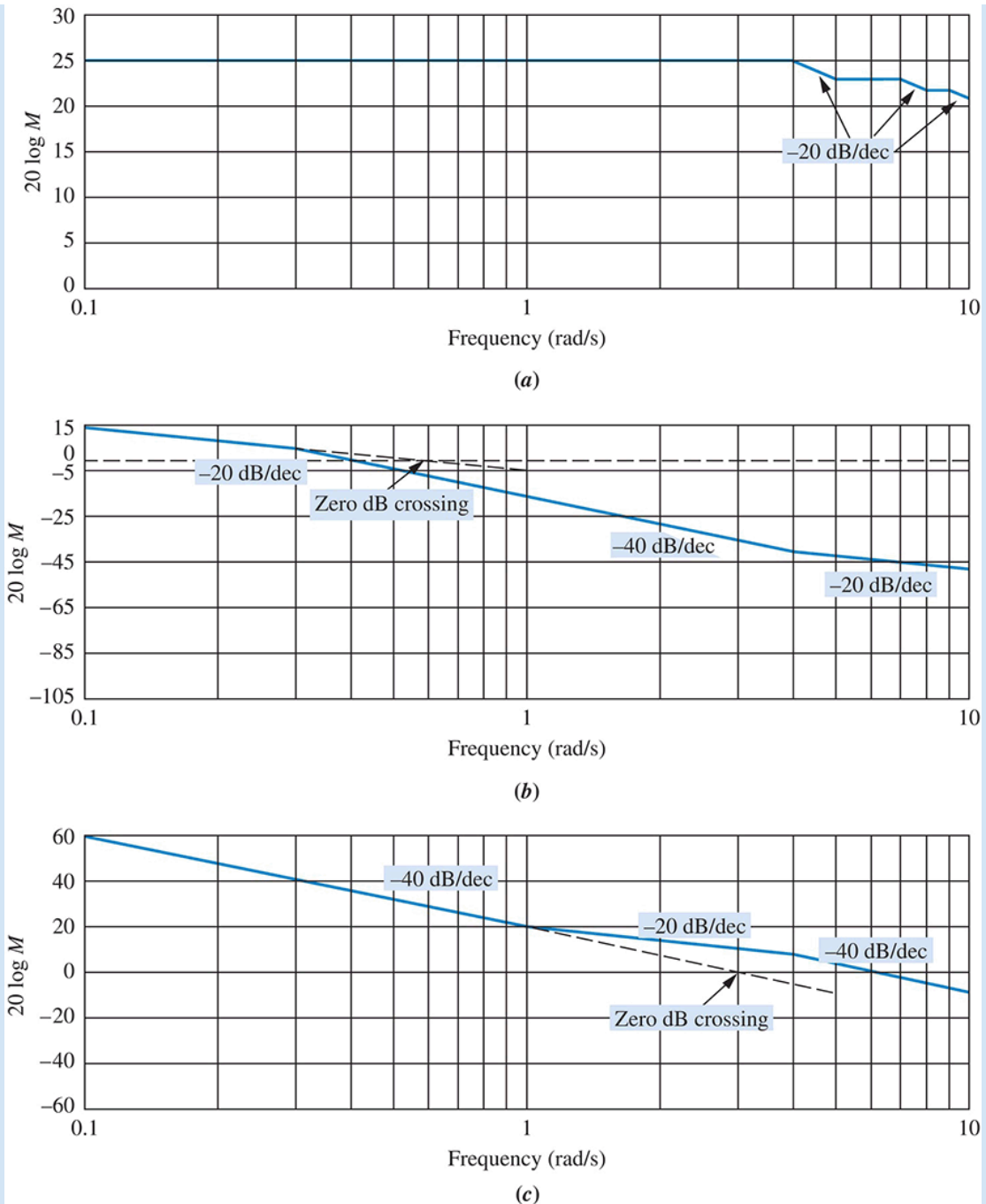
FIGURE 10.52 Bode log-magnitude plots for Example 10.14 .
