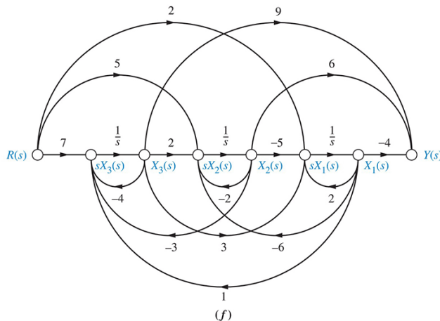
FIGURE 5.22 Stages of development of a signal-flow graph for the system of Eqs. (5.36) : a. place nodes; b. interconnect state variables and derivatives; c. form dx_1/dt ; d. form dx_2/dt ; e. form dx_3/dt ; f. form output
