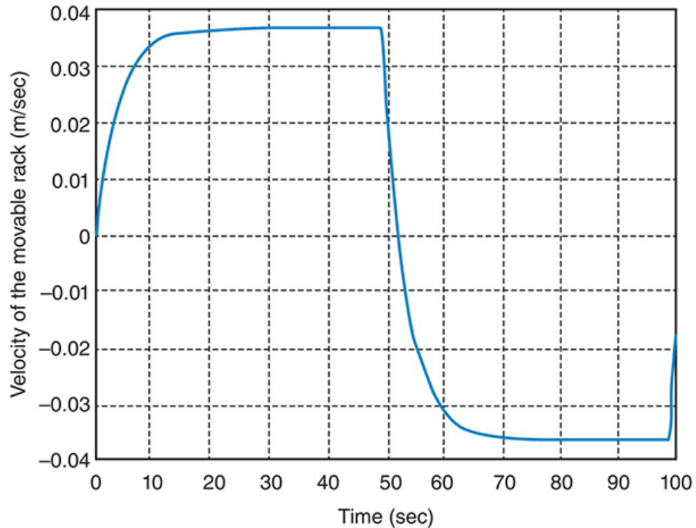
FIGURE P7.21 Velocity output response 2
