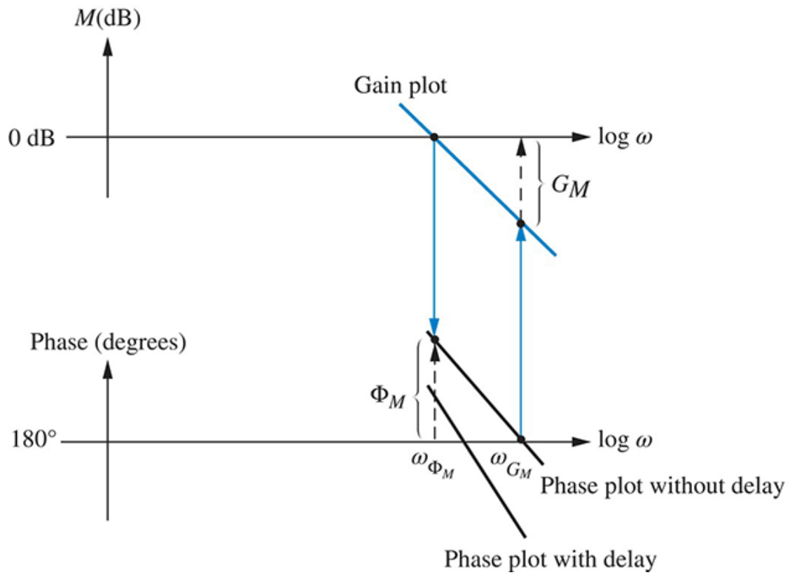
FIGURE 10.54 Effect of delay upon frequency response
