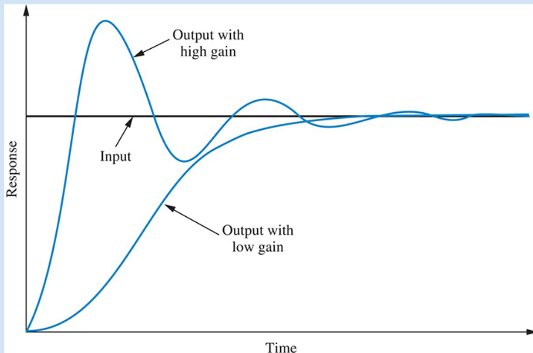
FIGURE 1.9 Response of a position control system, showing effect of high and low controller gain on the output response
