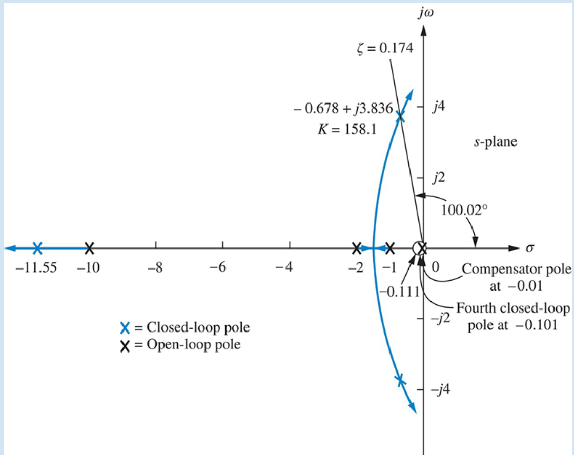
FIGURE 9.12 Root locus for compensated system of Figure 9.11
