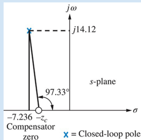
FIGURE 9.52 Finding the compensator zero in Example 9.7
