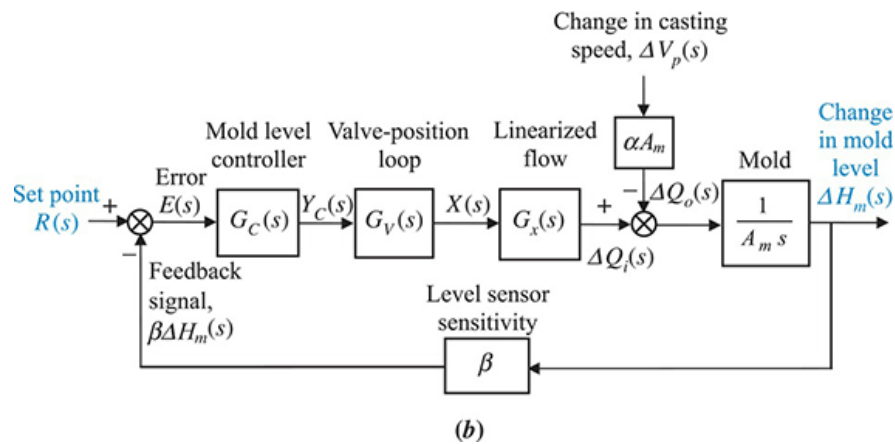
FIGURE P5.30 Steel mold process: a. process; b. block diagram
