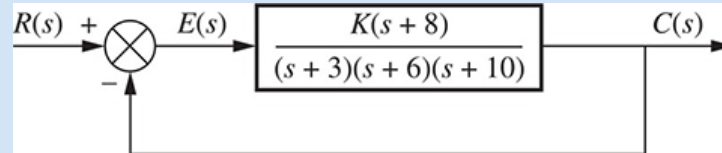
FIGURE 9.31 Uncompensated feedback control system for Example 9.5
