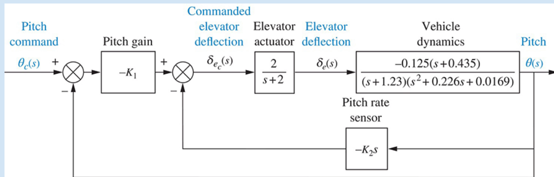
FIGURE 4.34 Pitch control loop for the UFSS vehicle
