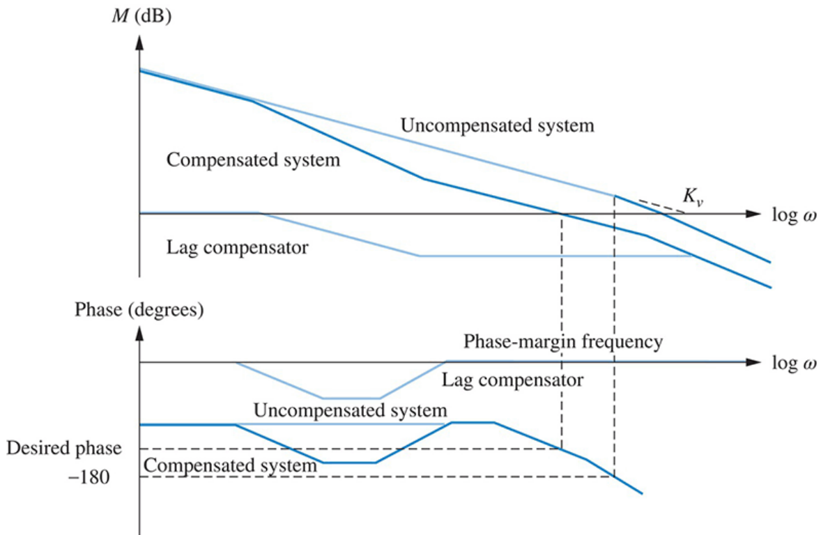
FIGURE 11.4 Visualizing lag compensation
