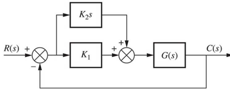
FIGURE 9.23 PD controller
