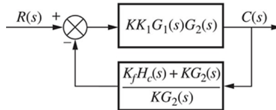
FIGURE 9.48 Equivalent block diagram of Figure 9.45
