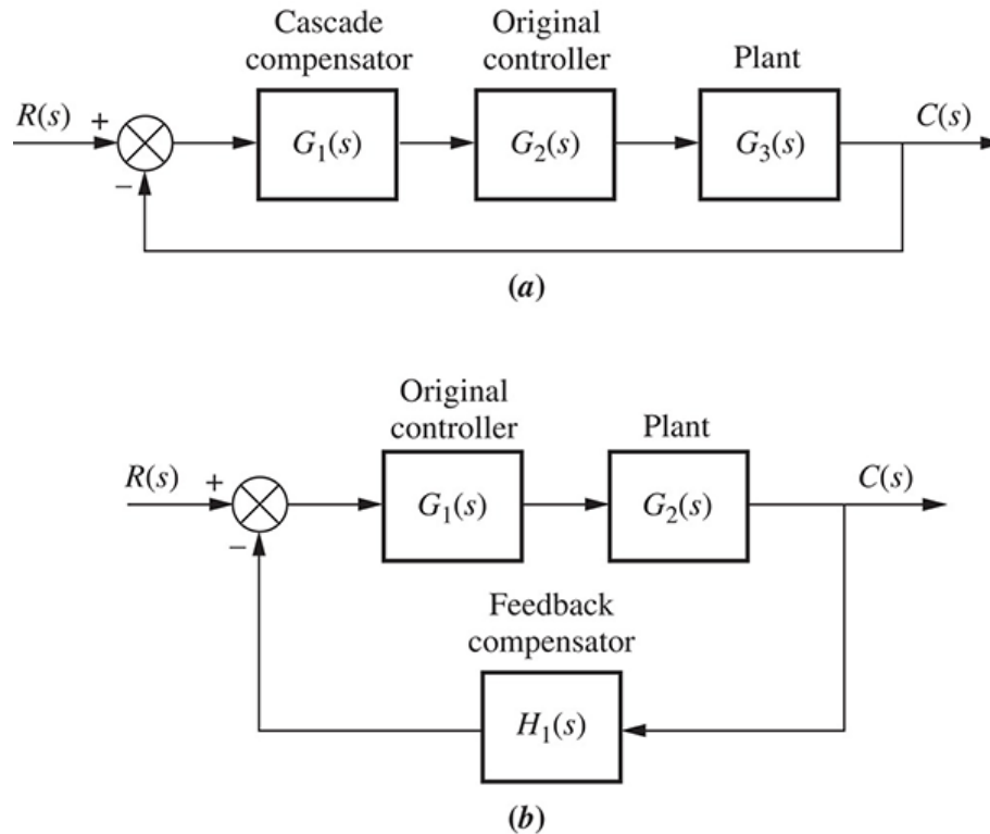
FIGURE 9.2 Compensation techniques: a. cascade; b. feedback
