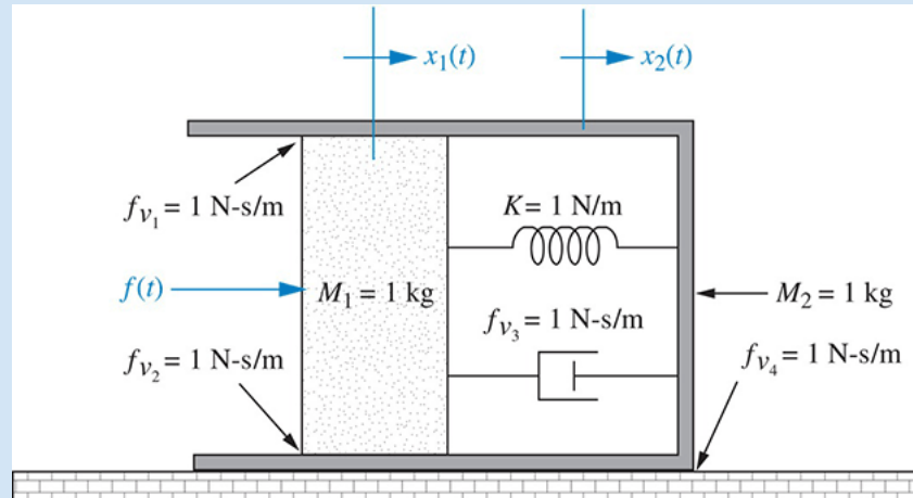
FIGURE 2.21 Translational mechanical system for Skill-Assessment Exercise 2.8
