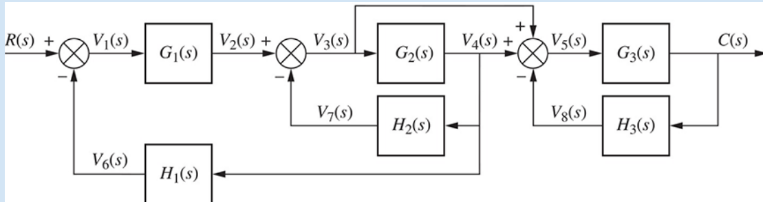
FIGURE 5.11 Block diagram for Example 5.2
