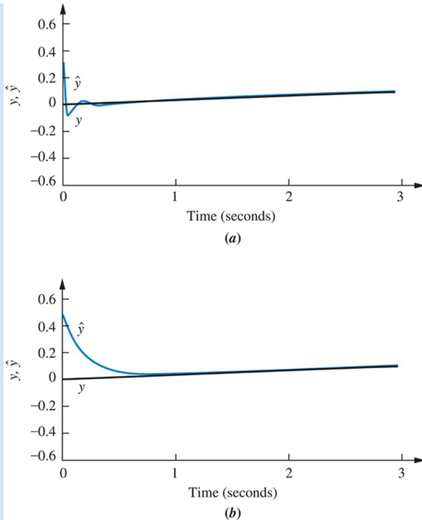
FIGURE 12.19 Observer design step response simulation: a. closed-loop observer; b. open-loop observer with observer gains disconnected
