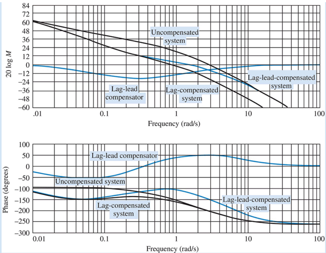
FIGURE 11.12 Bode plots for lag-lead compensation in Example 11.4
