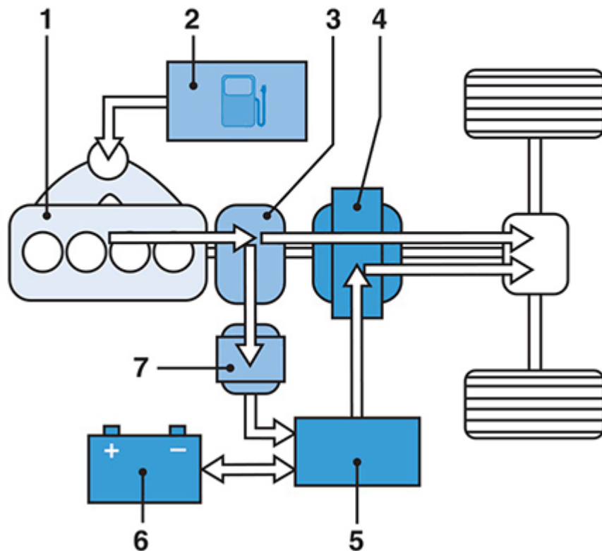
FIGURE P1.9 Split-power hybrid electric vehicle 7
