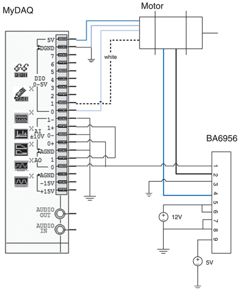
FIGURE 4.39 Wiring diagram 10
