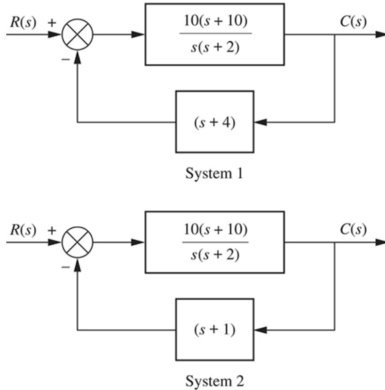
FIGURE P7.12 Closed-loop systems with nonunity feedback
