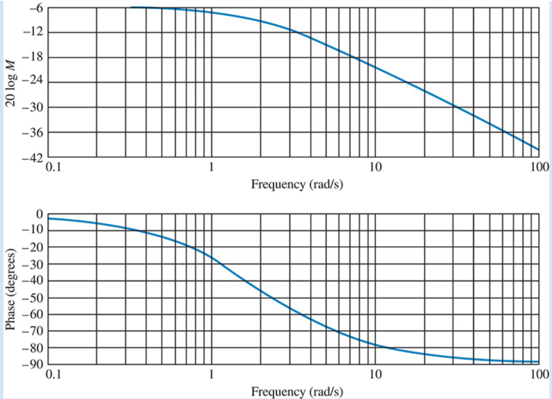
FIGURE 10.4 Frequency response plots for G(s) = 1/(s + 2) : separate magnitude and phase diagrams
