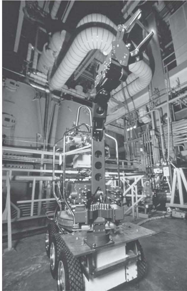
FIGURE 1.4 Rover was built to work in contaminated areas at Three Mile Island in Middleton, Pennsylvania, where a nuclear accident occurred in 1979. The remote-controlled robot's long arm can be seen at the front of the vehicle.
