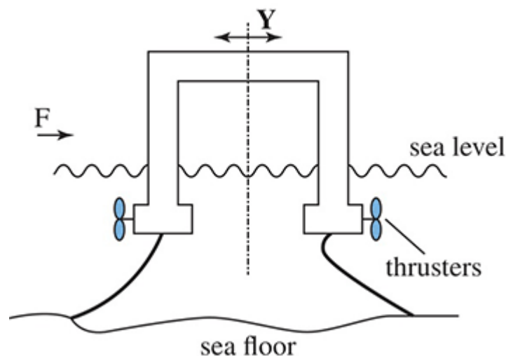
FIGURE P1.3 Tethered platform using side thrusters for positioning 2
