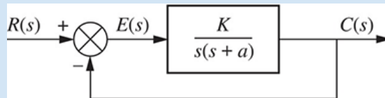
FIGURE 7.19 Feedback control system for Examples 7.10 and 7.11
