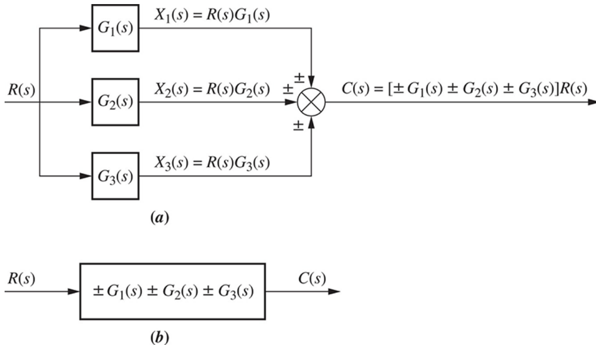
FIGURE 5.5 a. Parallel subsystems; b. equivalent transfer function
