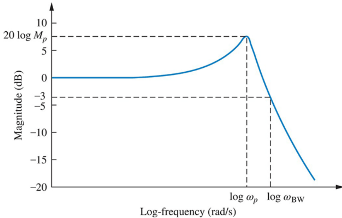
FIGURE 10.39 Representative log-magnitude plot of Eq. (10.51) .
