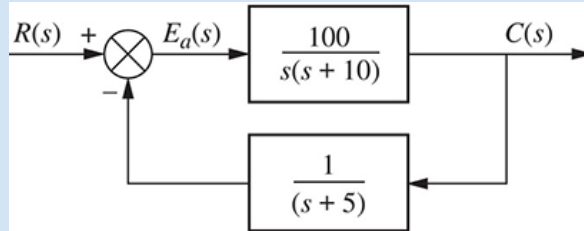
FIGURE 7.16 Nonunity-feedback control system for Example 7.8
