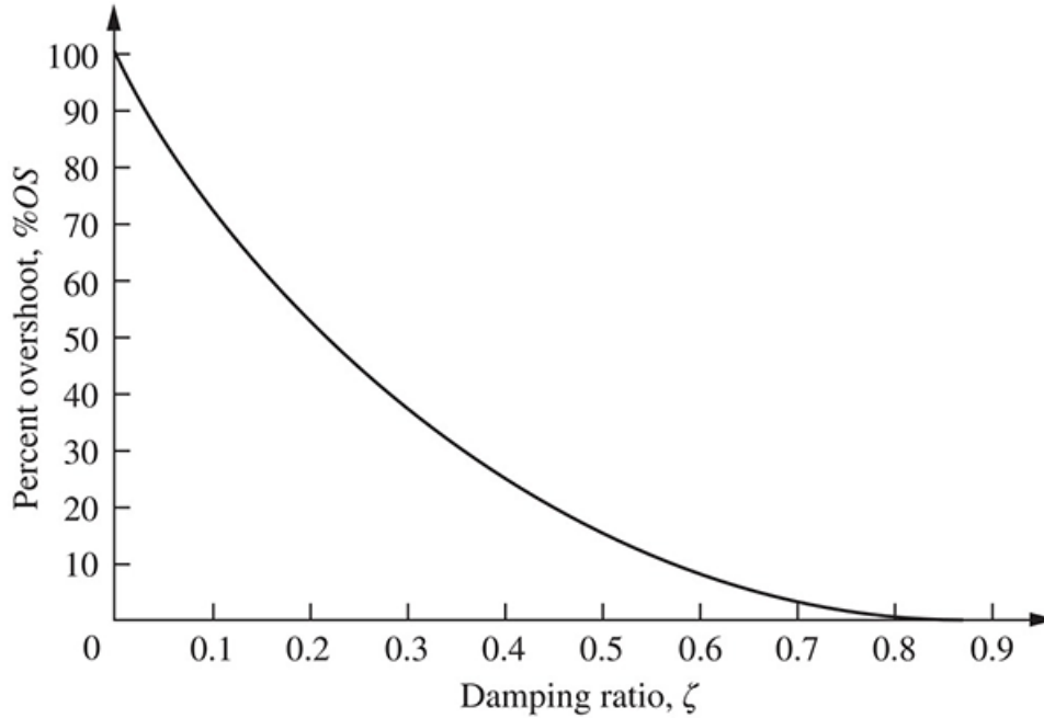
FIGURE 4.15 Percent overshoot versus damping ratio
