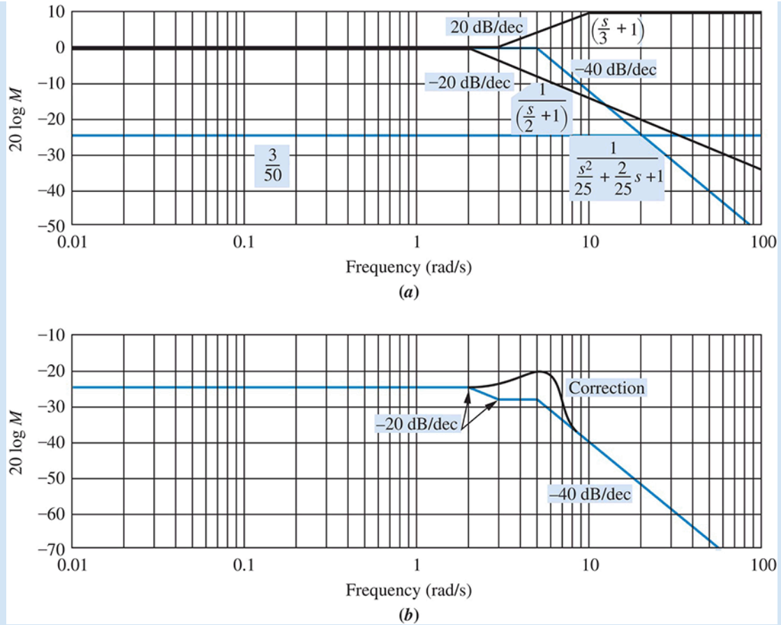
FIGURE 10.18 Bode magnitude plot for G(s) = \frac{(s + 3)}{[(s + 2)(s^2 + 2s + 25)]} :
