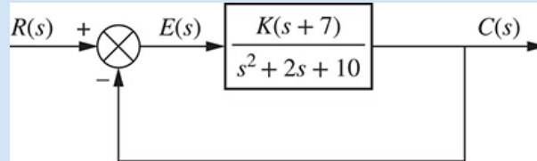
FIGURE 7.21 System for Skill-Assessment Exercise 7.6
