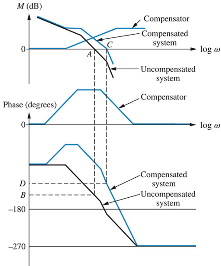
FIGURE 11.7 Visualizing lead compensation
