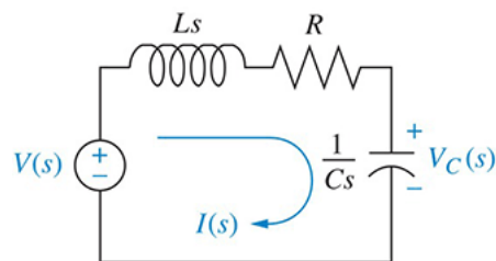
FIGURE 2.5 Laplace-transformed network
