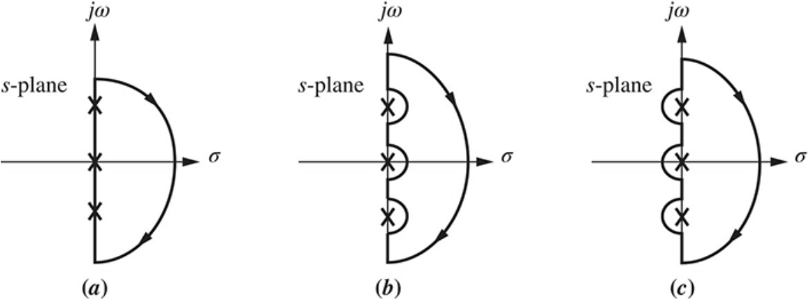
FIGURE 10.28 Detouring around open-loop poles: a. poles on contour; b. detour right; c. detour left
