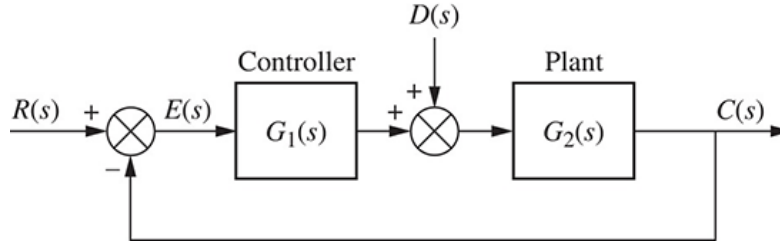
FIGURE 7.11 Feedback control system showing disturbance
