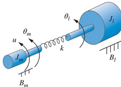
FIGURE P8.16 Idealized model representing joint flexibility 4
