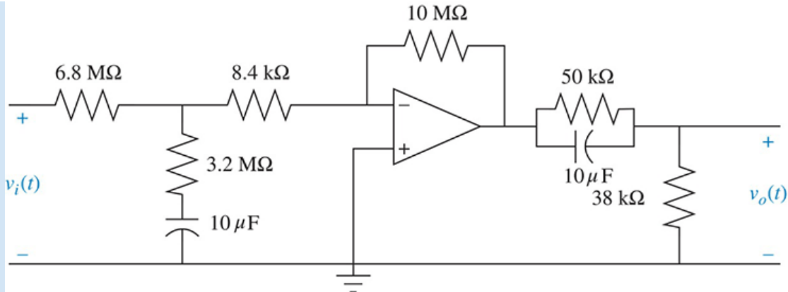
FIGURE 9.65 Realization of lag–lead compensator
