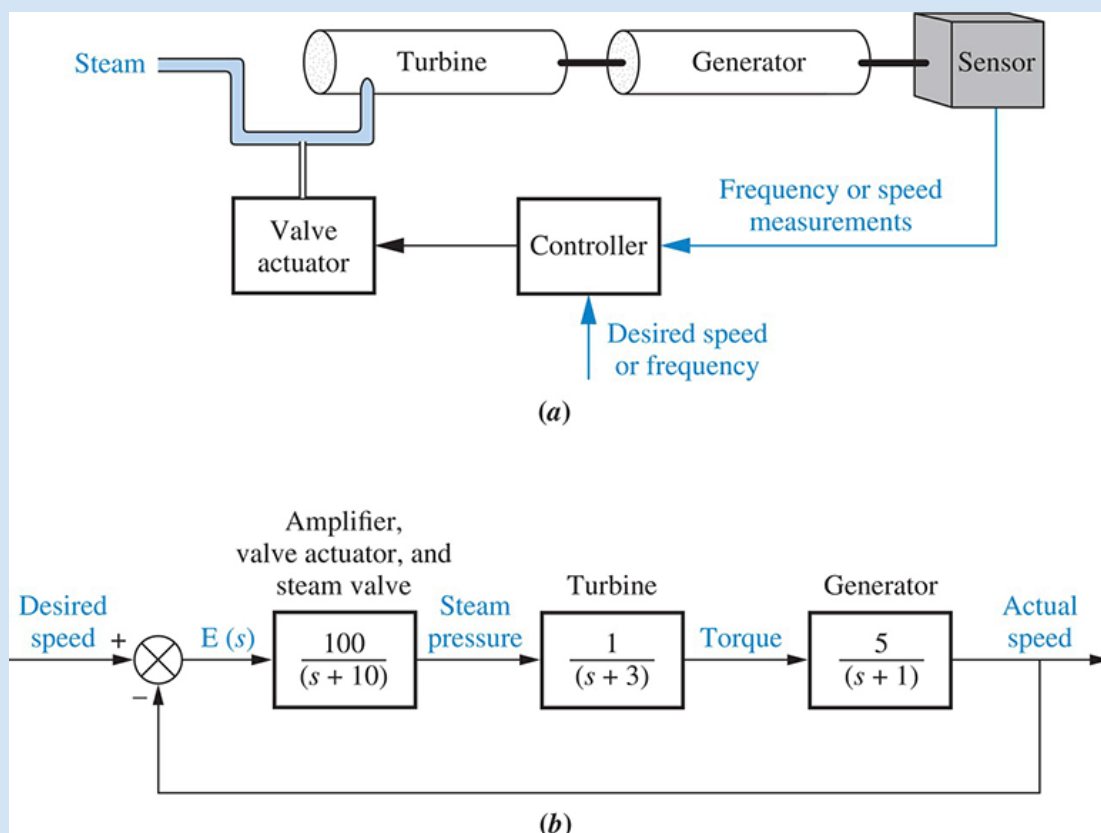
FIGURE 10.26 a. Turbine and generator; b. block diagram of speed control system for Example 10.4 .
