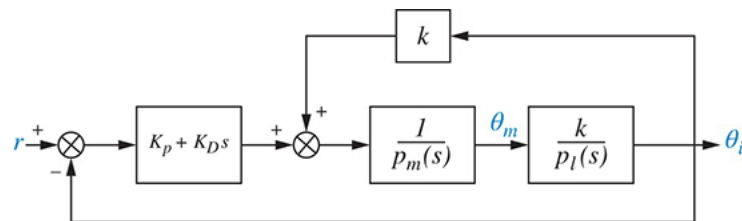
FIGURE P8.17 Joint flexibility model inserted in feedback loop 5
