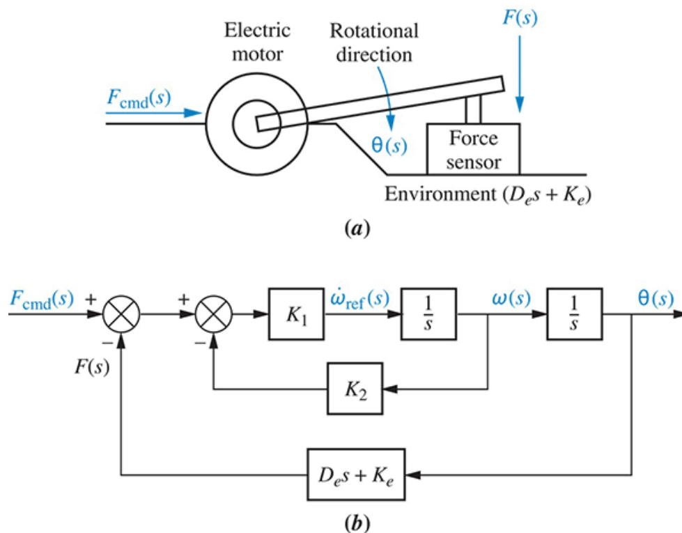
FIGURE P7.24 a. Force control mechanical loop under contact motion; 4 b. block diagram 4
