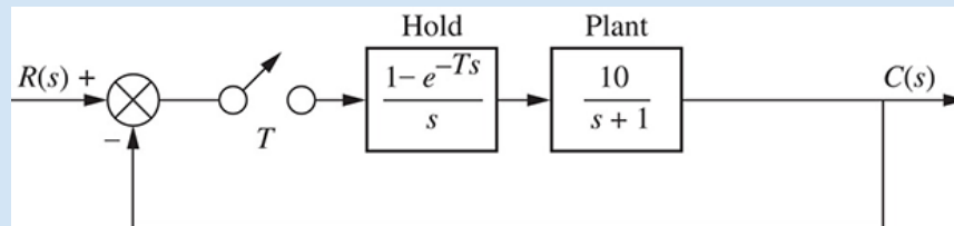
FIGURE 13.15 Digital system for Example 13.7
