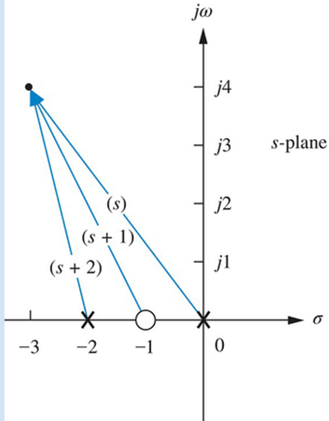
FIGURE 8.3 Vector representation of Eq.(8.7) .
