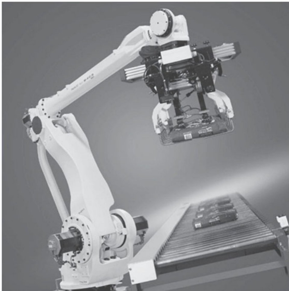
FIGURE 6.11 A FANUC M-410iB™ has 4 axes of motion. It is seen here performing bag palletizing
