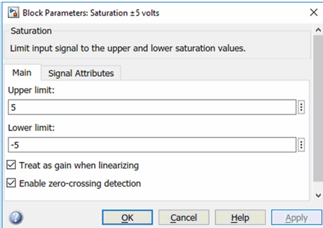
FIGURE C.11 a. Simulink library for nonlinearities; b. parameter settings for saturation
