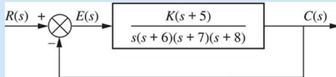
FIGURE 7.10 Feedback control system for Example 7.6
