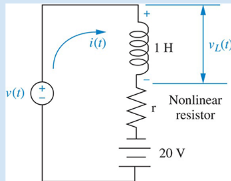
FIGURE 2.49 Nonlinear electrical network
