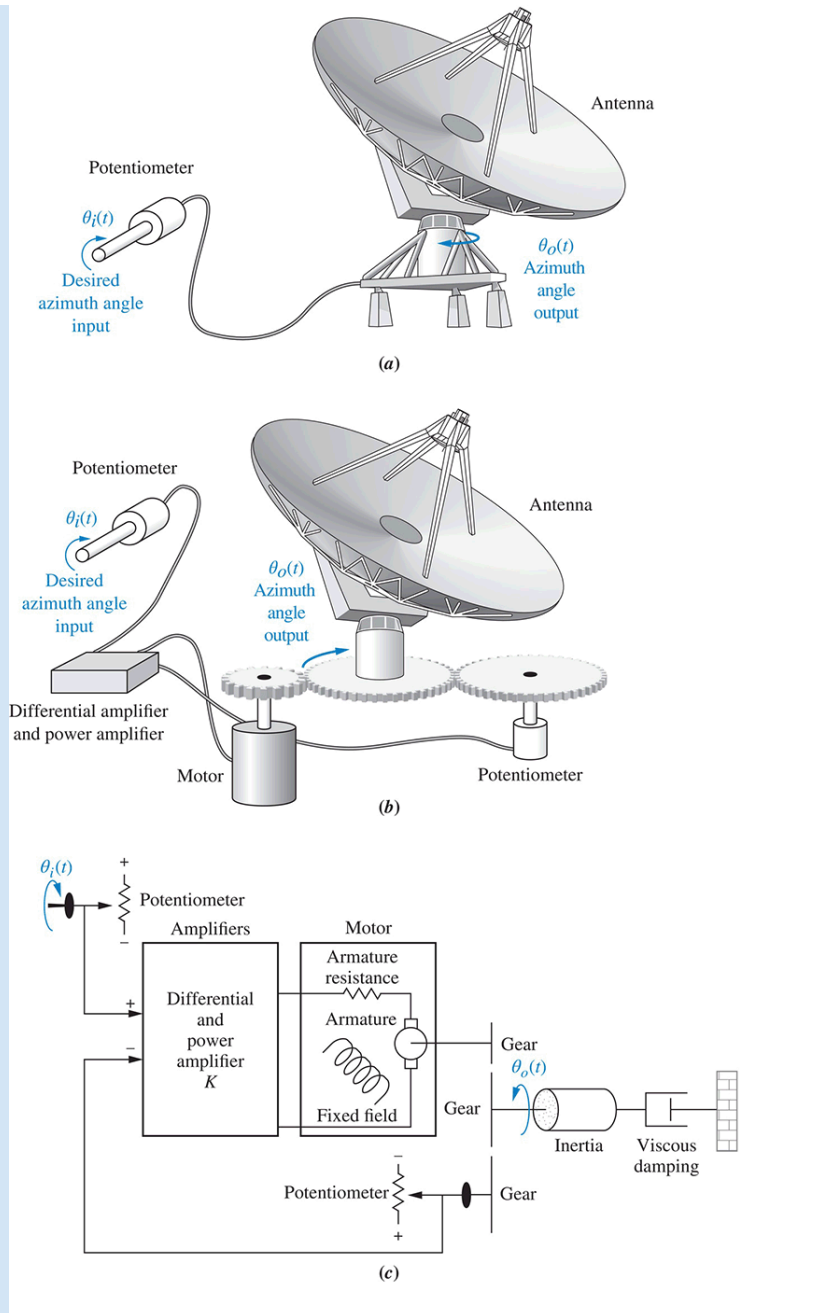
FIGURE 1.8 Antenna azimuth position control system: a. system concept; b. detailed layout; c. schematic d. functional block diagram
