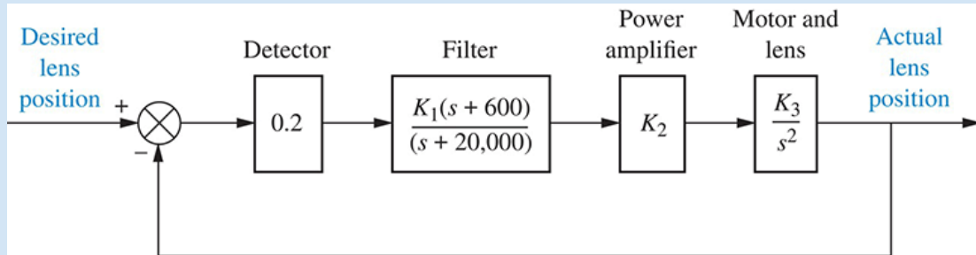
FIGURE 7.24 Video laser disc recording focusing system
