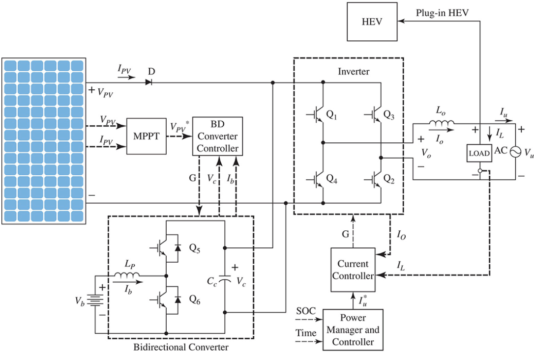
FIGURE P1.4 Proposed solar powered residential home with plug-in hybrid electric vehicle (PHEV) loads 4
