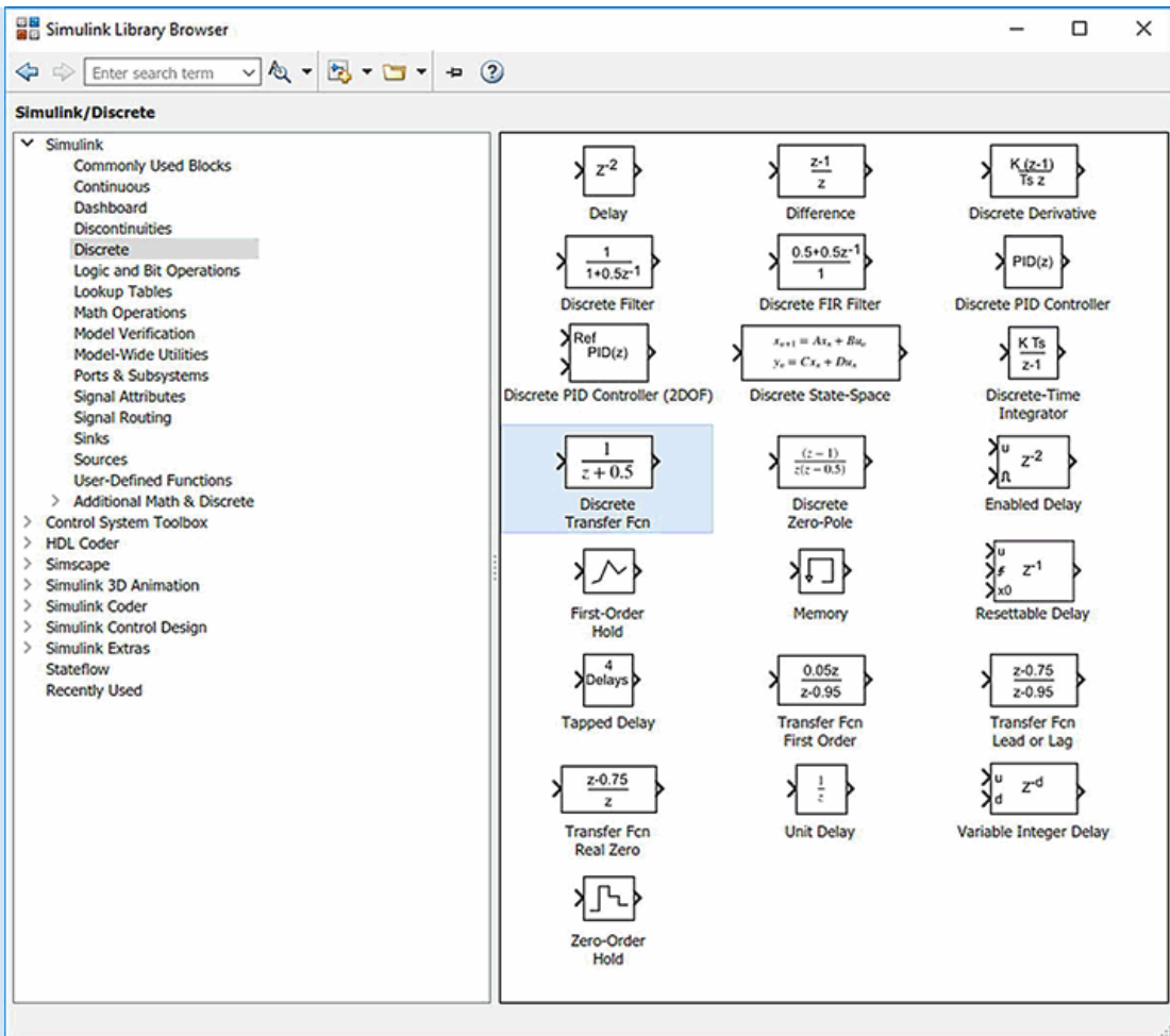
FIGURE C.16 Simulink library of discrete blocks
