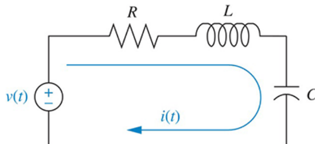
FIGURE 3.2 RLC network
