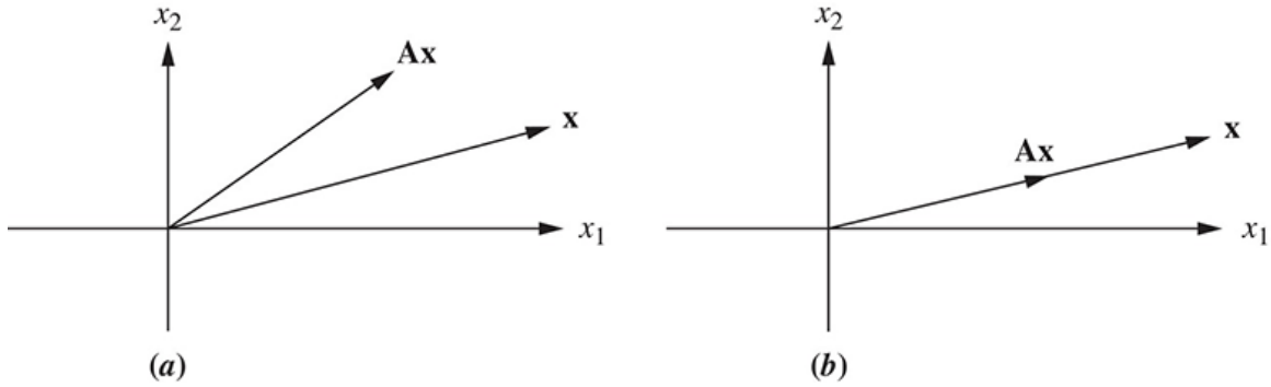
FIGURE 5.32 To be an eigenvector, the transformation Ax must be collinear with x ; thus, in (a), x is not an eigenvector; in (b), it is.
