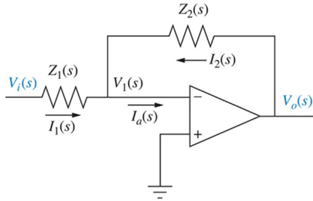
FIGURE 9.60 Operational amplifier configured for transfer function realization
