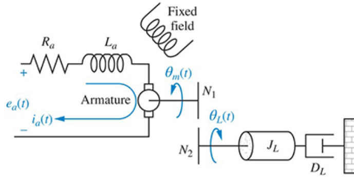
FIGURE P3.10 Motor and load
