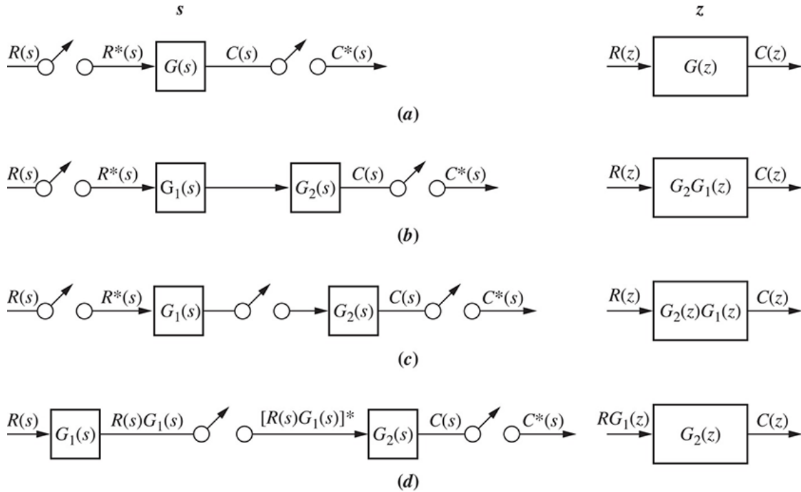
FIGURE 13.9. Sampled-data systems and their z-transforms
