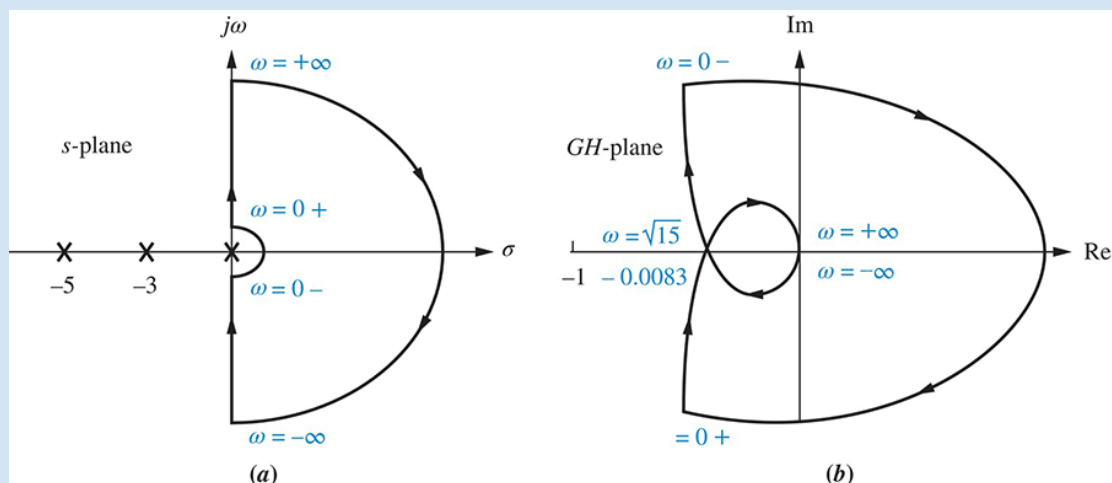
FIGURE 10.31 a. Contour for Example 10.6 ; b. Nyquist diagram
