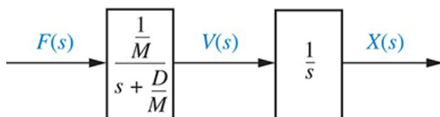
FIGURE 3.4 Block diagram of a mass and damper
