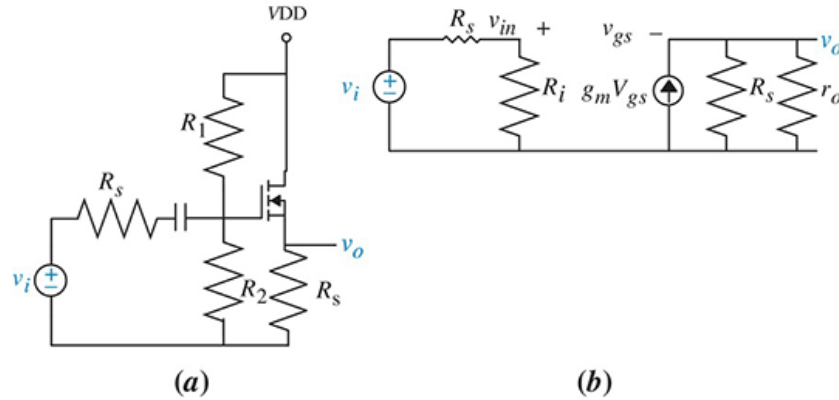
FIGURE P5.25 a. An n -channel enhancement-mode MOSFET source follower circuit; b. small-signal equivalent
