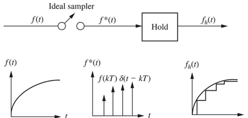
FIGURE 13.7 Ideal sampling and the zero-order hold
