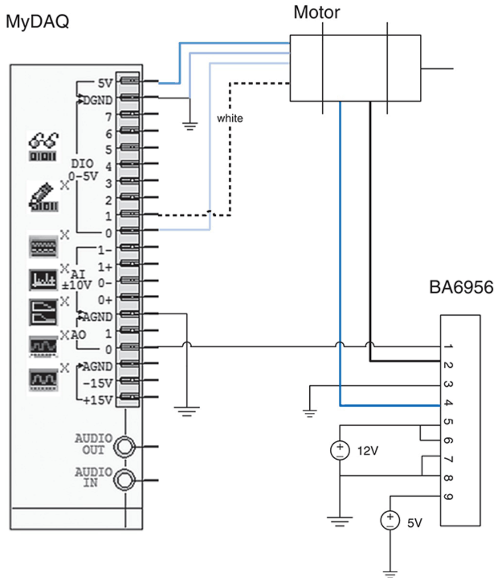
FIGURE 4.38 Wiring diagram 9
