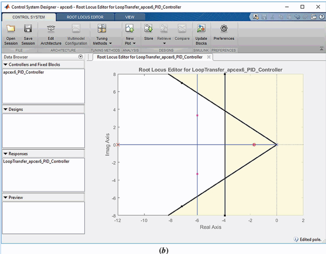
FIGURE C.27 Root locus plots with design boundaries: a. Original ; b. After moving compensator pole
