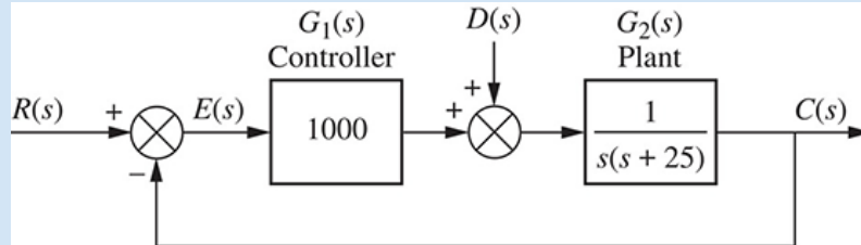
FIGURE 7.13 Feedback control system for Example 7.7 .
