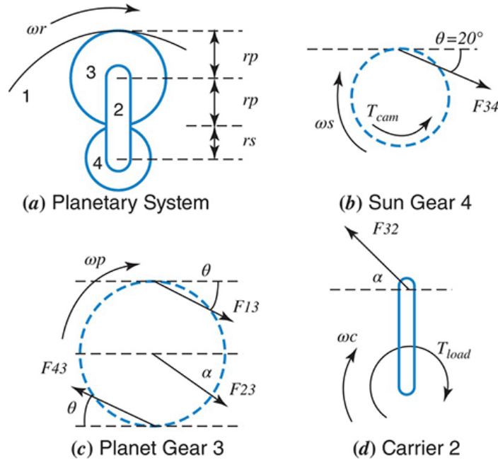
FIGURE P4.12 Free-body diagrams of planetary gear system components 2
