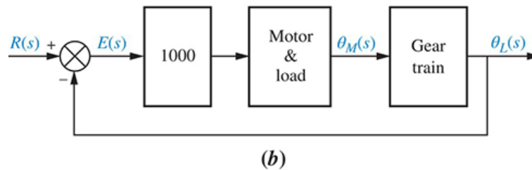
FIGURE P5.34 Position control: a. motor and load; b. block diagram
