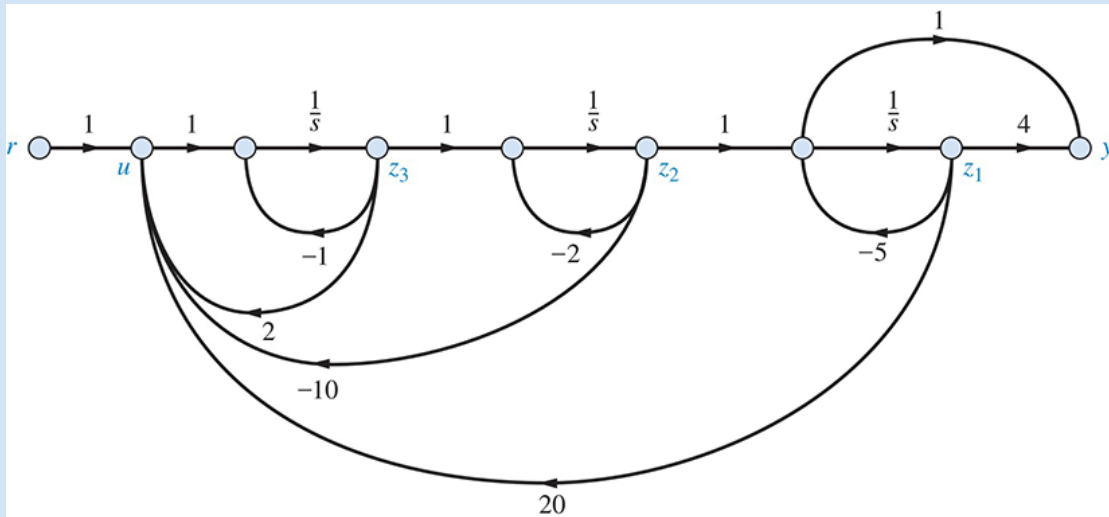
FIGURE 12.10 Designed system with state-variable feedback for Example 12.4
