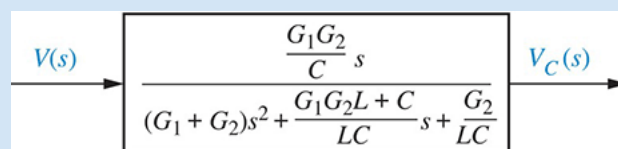
FIGURE 2.7 Block diagram of the network of Figure 2.6
