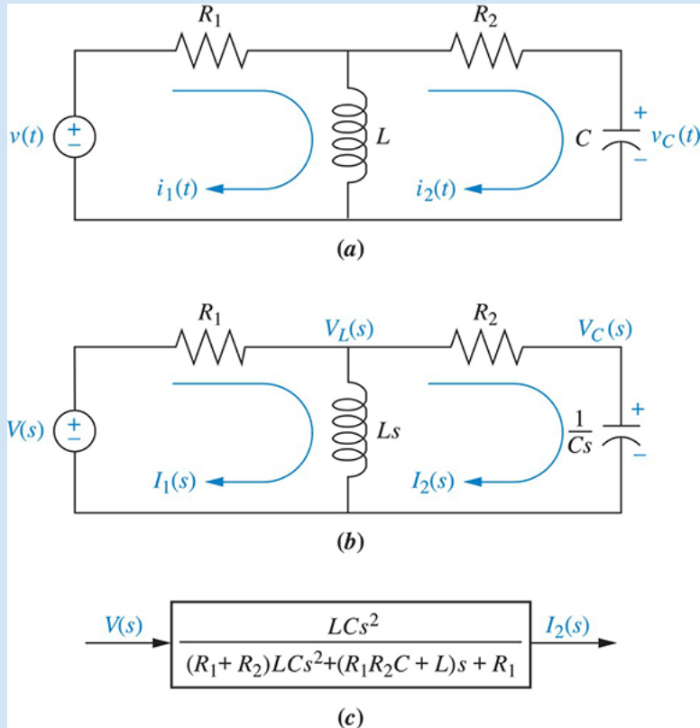
FIGURE 2.6 a. Two-loop electrical network; b. transformed two-loop electrical network; c. block diagram
