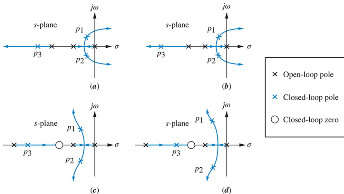
FIGURE 8.20 Making second-order approximations
