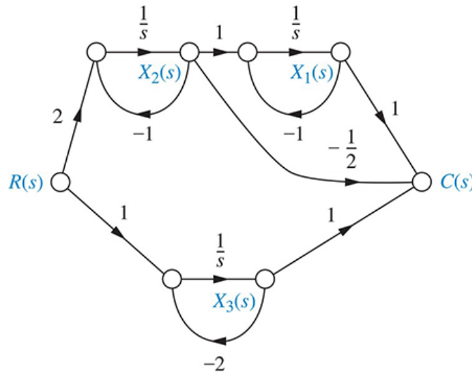
FIGURE 5.26 Signal-flow representation of Eq. (5.52) .
