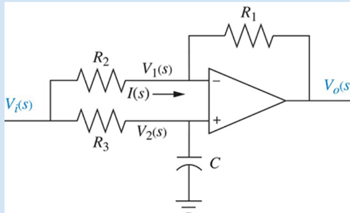
FIGURE 4.27 Nonminimum-phase electric circuit 6
