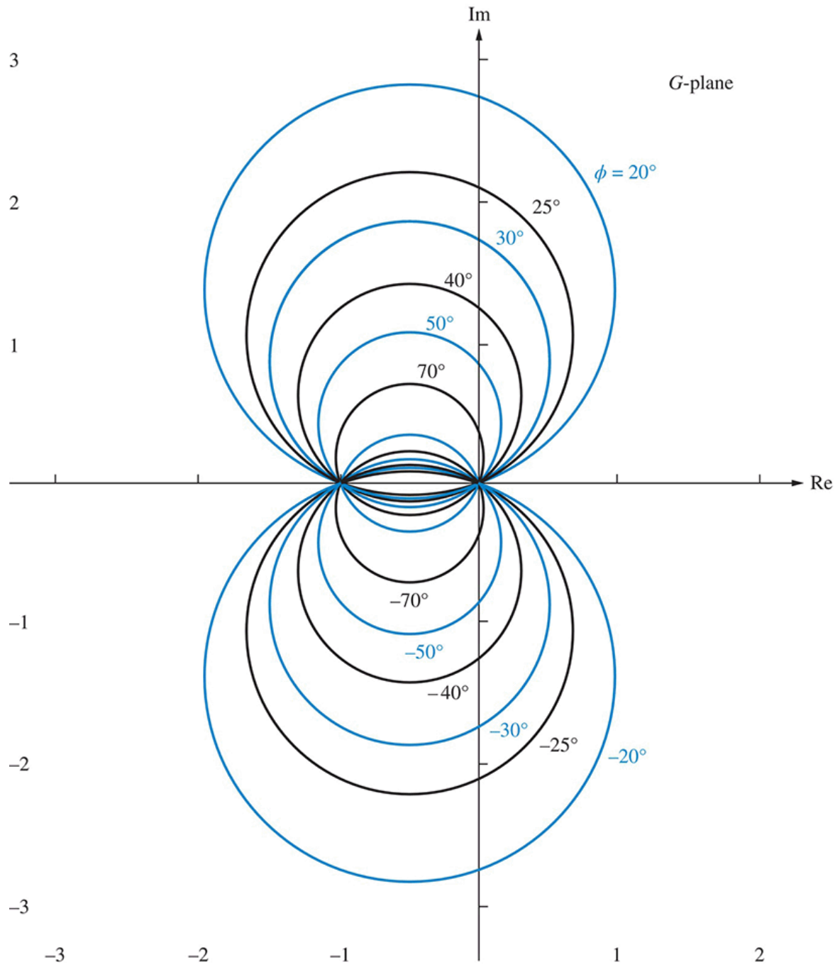
FIGURE 10.43 Constant N circles
