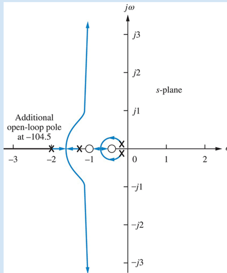
FIGURE 9.68 Root locus for lead-compensated system
