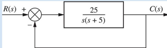
FIGURE 5.15 Feedback system for Example 5.3
