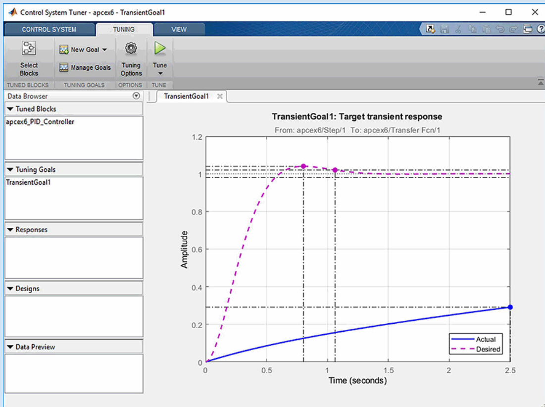
FIGURE C.24 Control System Tuner window with Target transient response plots with Control System tab selected
