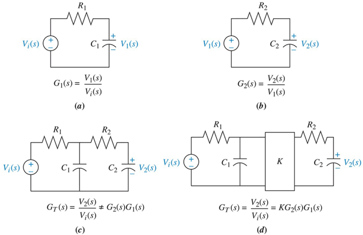
FIGURE 5.4 Loading in cascaded systems
