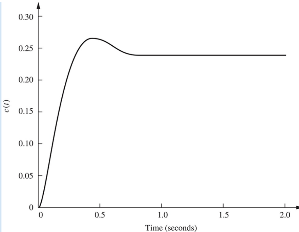
FIGURE 12.5 Simulation of closed-loop system of Example 12.1
