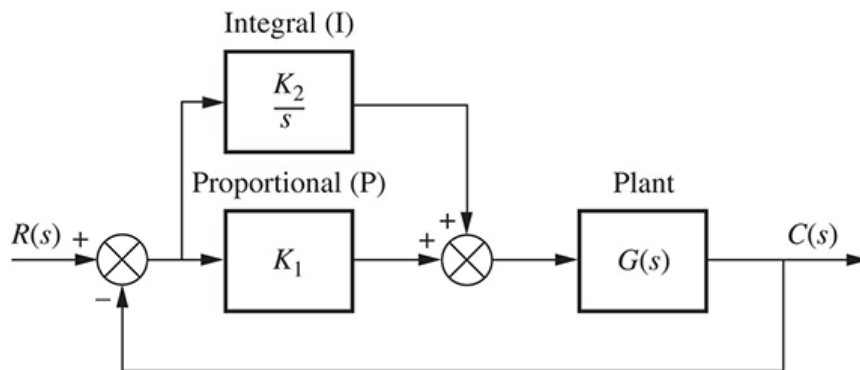
FIGURE 9.8 PI controller
