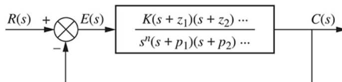
FIGURE 7.8 Feedback control system for defining system type
