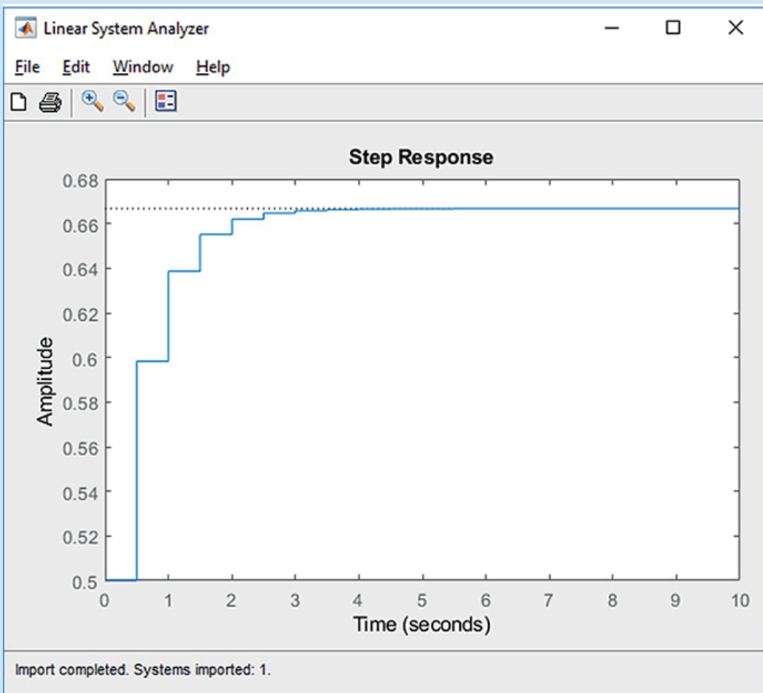
FIGURE E.6 Linear System Analyzer used for digital step response: a. M-file; b. Linear System Analyzer
