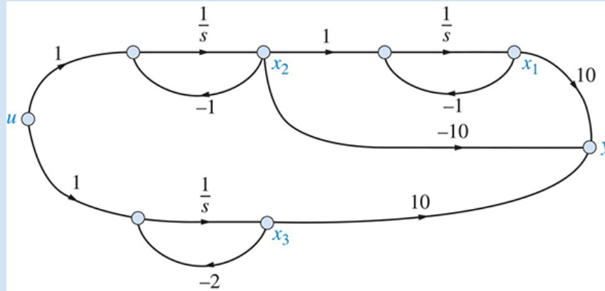
FIGURE 12.7 System for Example 12.2
