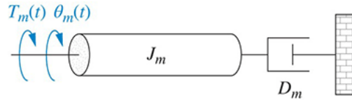
FIGURE 2.36 Typical equivalent mechanical loading on a motor
