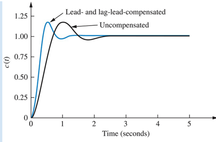
FIGURE 9.42 Improvement in step response for lag-lead-compensated system of Example 9.6
