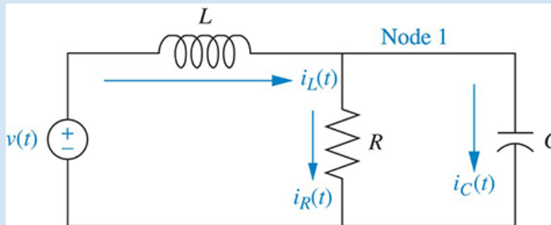
FIGURE 3.5 Electrical network for representation in state space
