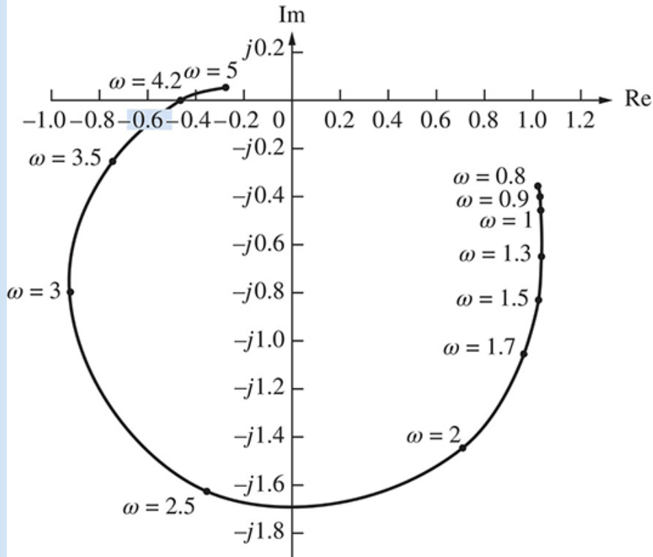
FIGURE 10.45 Closed-loop frequency response for Example 10.11
