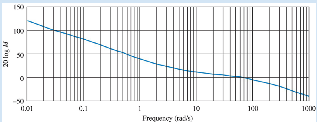
FIGURE 10.53 Bode log-magnitude plot for Skill-Assessment Exercise 10.10
