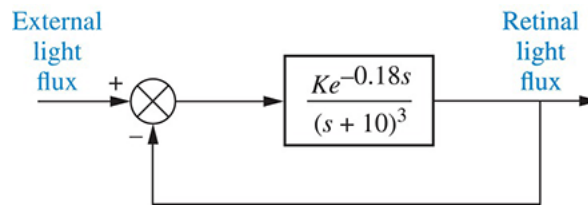
FIGURE P8.14 Simplified block diagram of pupil servomechanism
