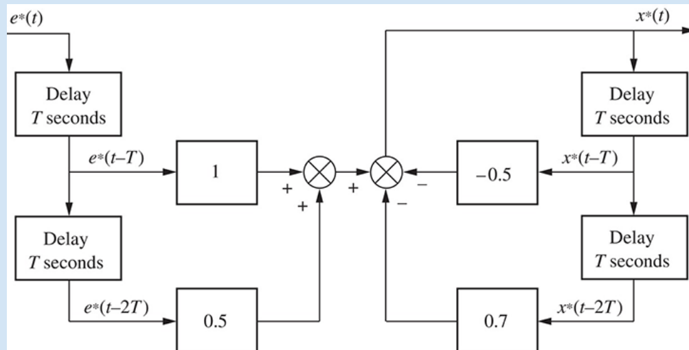
FIGURE 13.29 Flowchart to implement G_c(z) = \frac{z+0.5}{z^2-0.5z+0.7}
