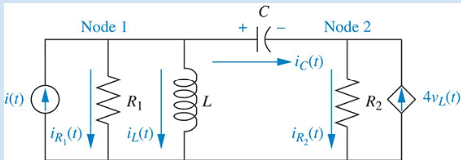
FIGURE 3.6 Electrical network for Example 3.2
