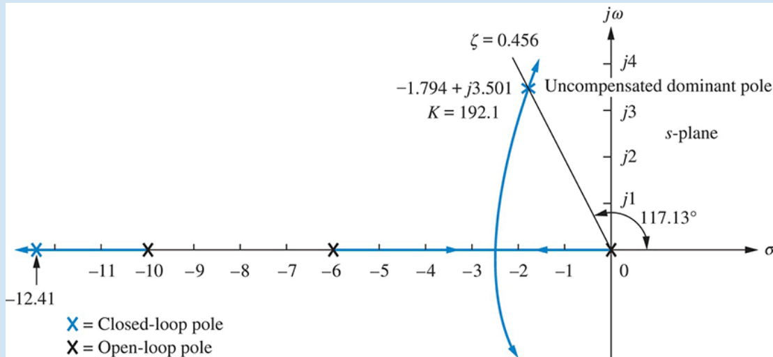
FIGURE 9.38 Root locus for uncompensated system of Example 9.6
