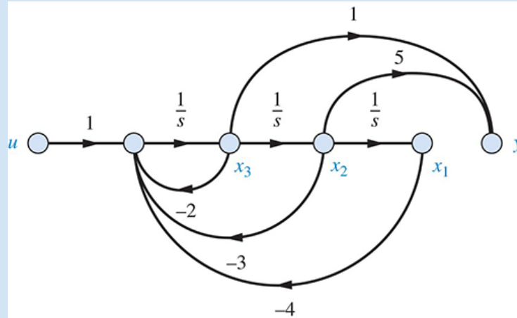
FIGURE 12.16 System of Example 12.6
