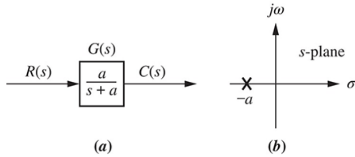
FIGURE 4.4 a. First-order system; b. Pole plot
