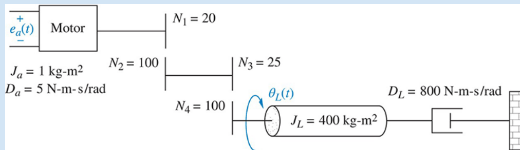
FIGURE 2.40 Electromechanical system for Skill-Assessment Exercise 2.11
