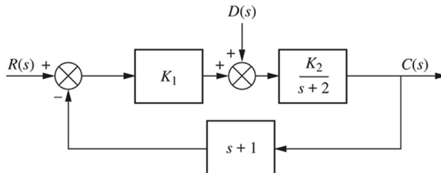
FIGURE P7.19 System with input and disturbance
