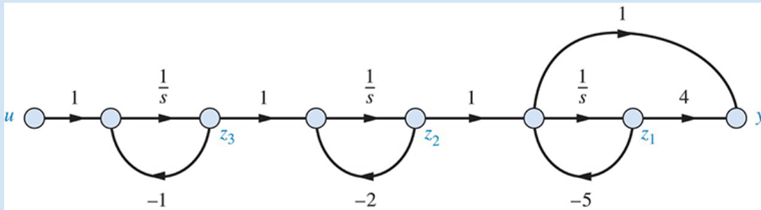
FIGURE 12.9 Signal-flow graph for plant of Example 12.4.
