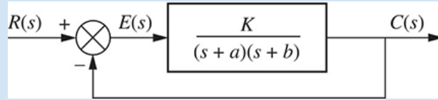
FIGURE 7.20 Feedback control system for Example 7.12
