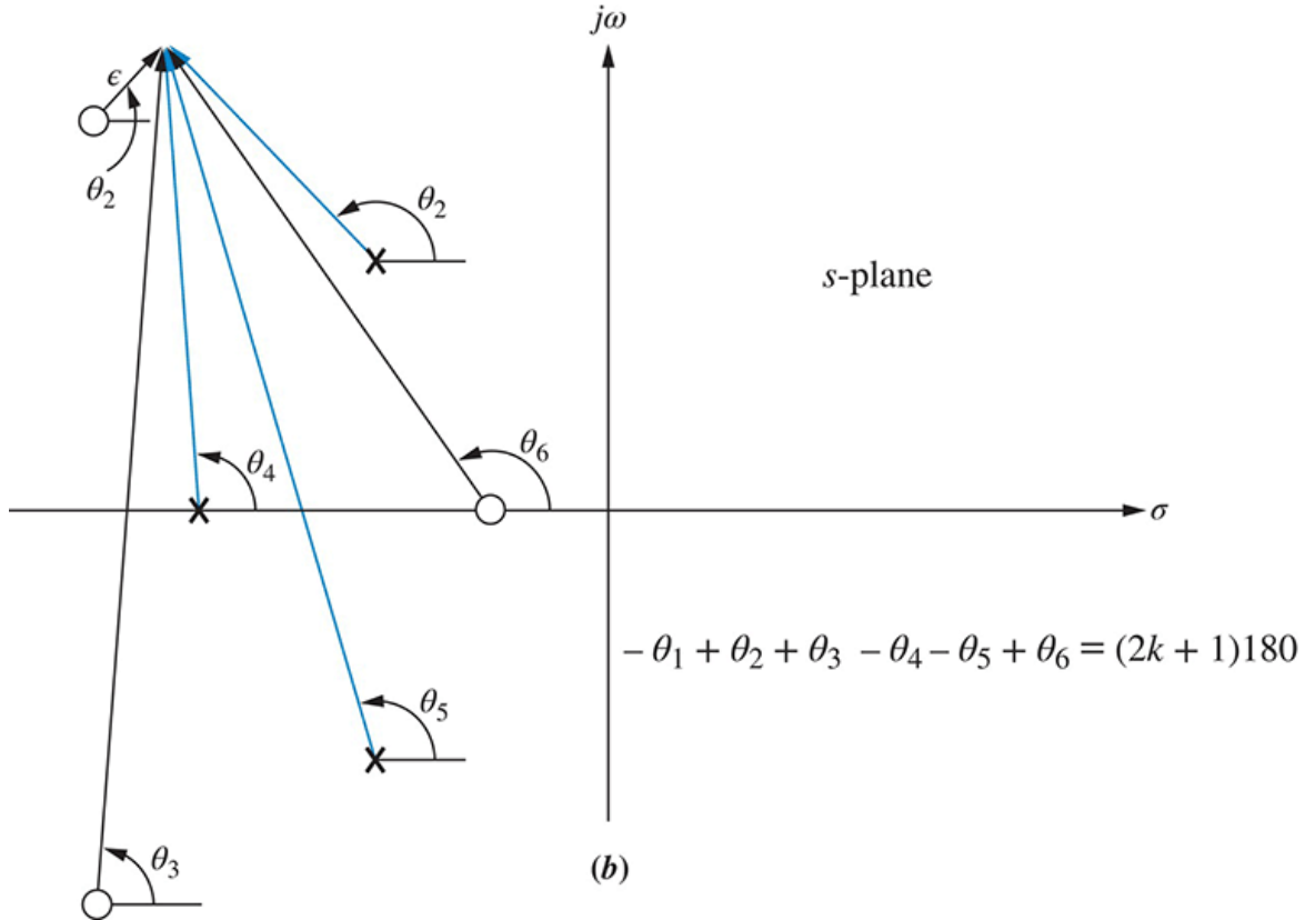
FIGURE 8.15 Open-loop poles and zeros and calculation of a. angle of departure; b. angle of arrival
