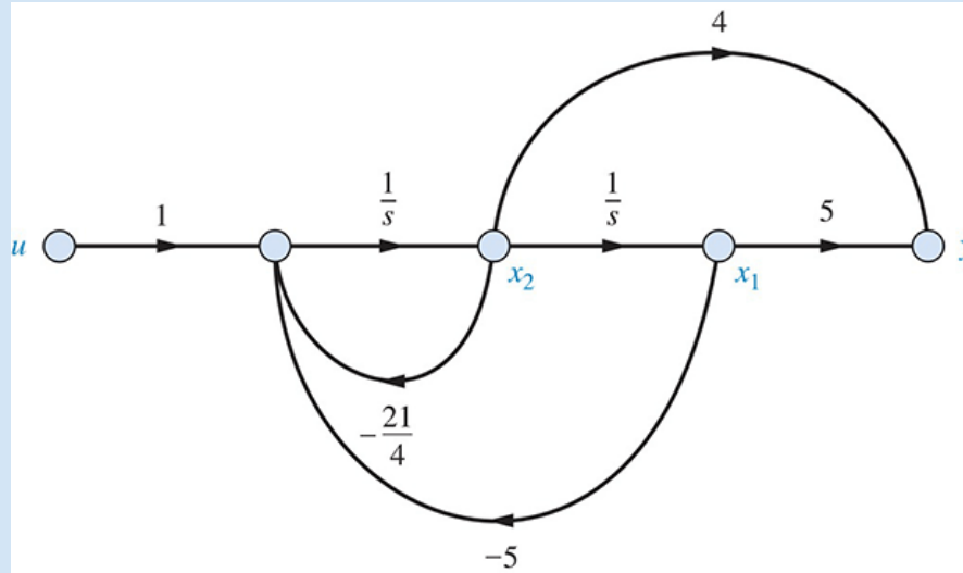
FIGURE 12.17 System of Example 12.7 .
