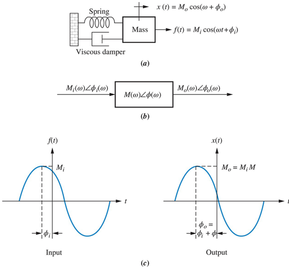
FIGURE 10.2 Sinusoidal frequency response: a. system; b. transfer function; c. input and output waveforms
