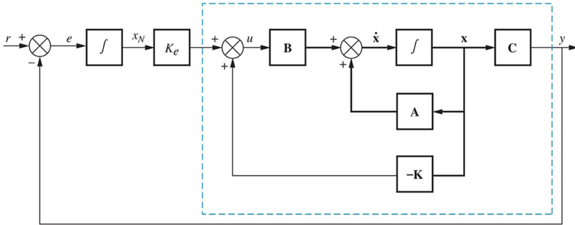
FIGURE 12.21 Integral control for steady-state error design
