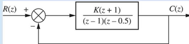
FIGURE 13.21 Digital feedback control for Example 13.10
