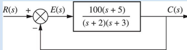
FIGURE 5.29 Feedback control system for Example 5.8
