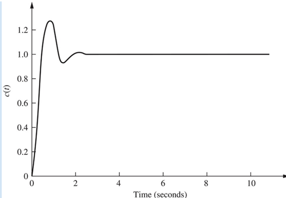
FIGURE 9.66 Step response of lag–lead-compensated antenna control
