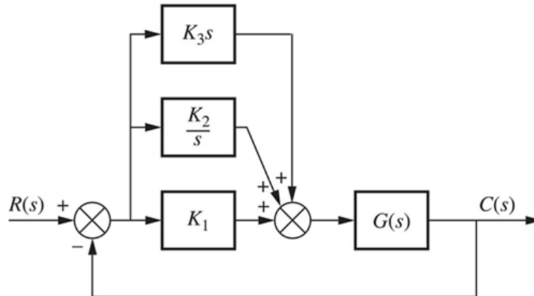
FIGURE 9.30 PID controller
