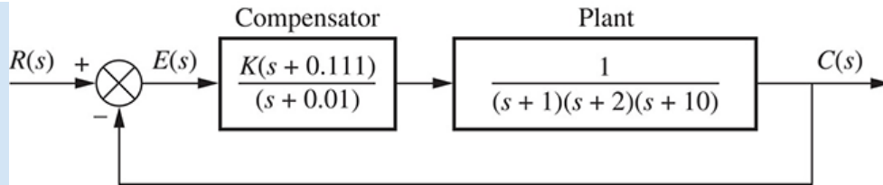
FIGURE 9.11 Compensated system for Example 9.2
