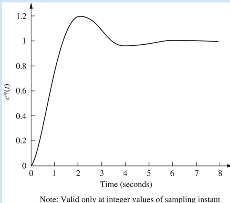
FIGURE 13.33 Sampled step response of the antenna azimuth position control system
