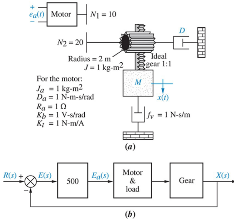
FIGURE P5.36 a. Motor and load; b. motor and load in feedback system
