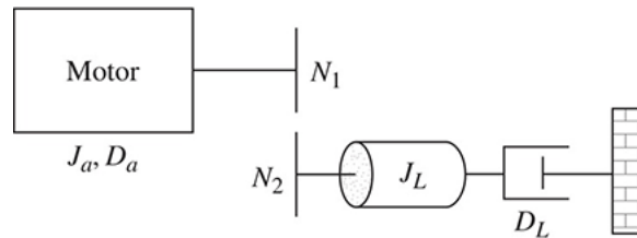
FIGURE 2.37 DC motor driving a rotational mechanical load
