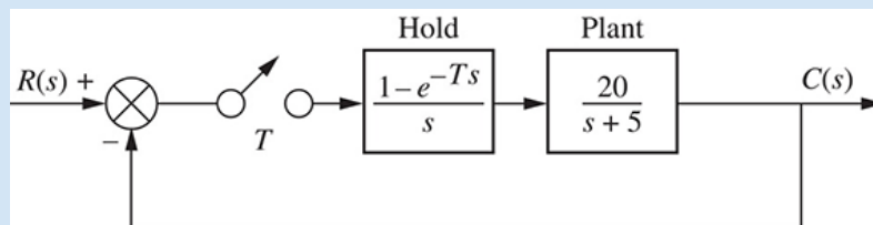
FIGURE 13.16 Digital system for Skill-Assessment Exercise 13.5
