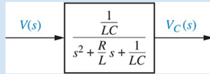
FIGURE 2.4 Block diagram of series RLC electrical network
