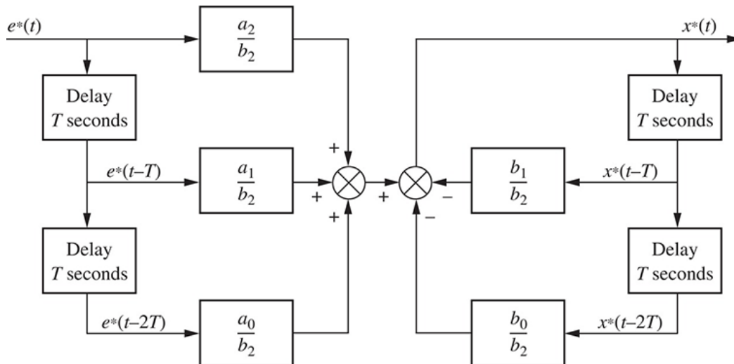
FIGURE 13.28 Flowchart for a second-order digital compensator 6
