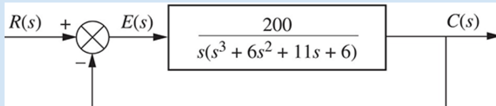
FIGURE 6.6 Feedback control system for Example 6.6
