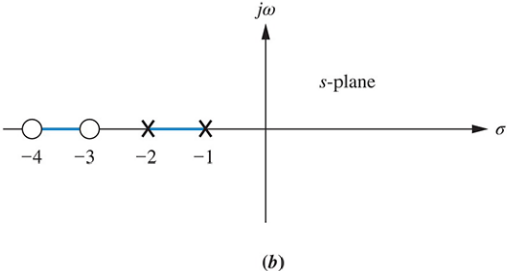
FIGURE 8.6 a. Example system; b. pole-zero plot of G(s)
