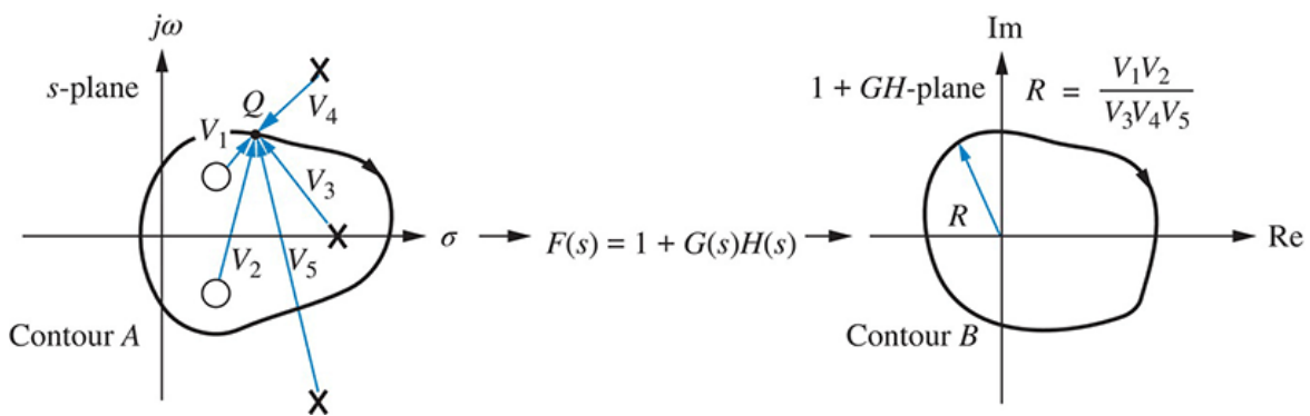
FIGURE 10.23 Vector representation of mapping
