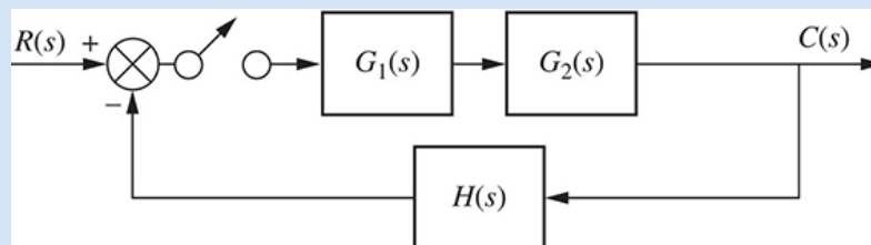
FIGURE 13.11 Digital system for Skill-Assessment Exercise 13.4 .
