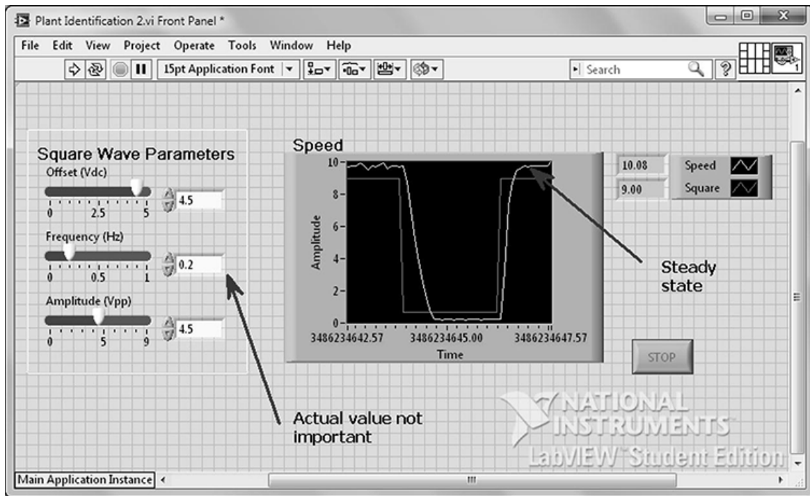
FIGURE 4.41 Plant Identification 2.vi Front Panel
