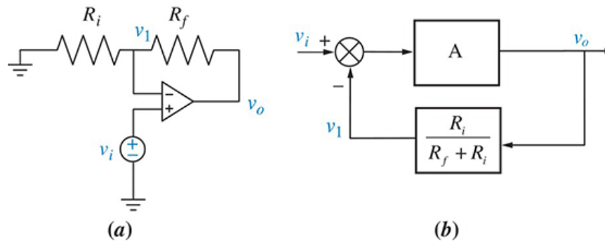
FIGURE P5.24 a. Noninverting amplifier; b. block diagram
