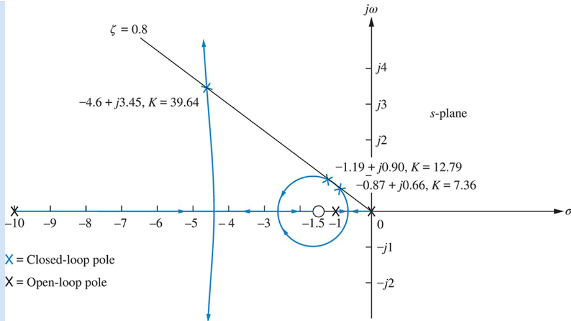
FIGURE 8.22 Root locus for Example 8.8
