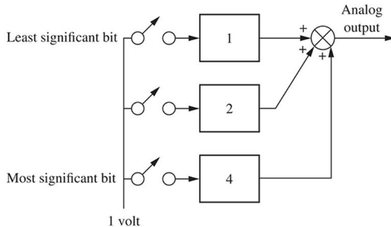
FIGURE 13.3 Digital-to-analog converter
