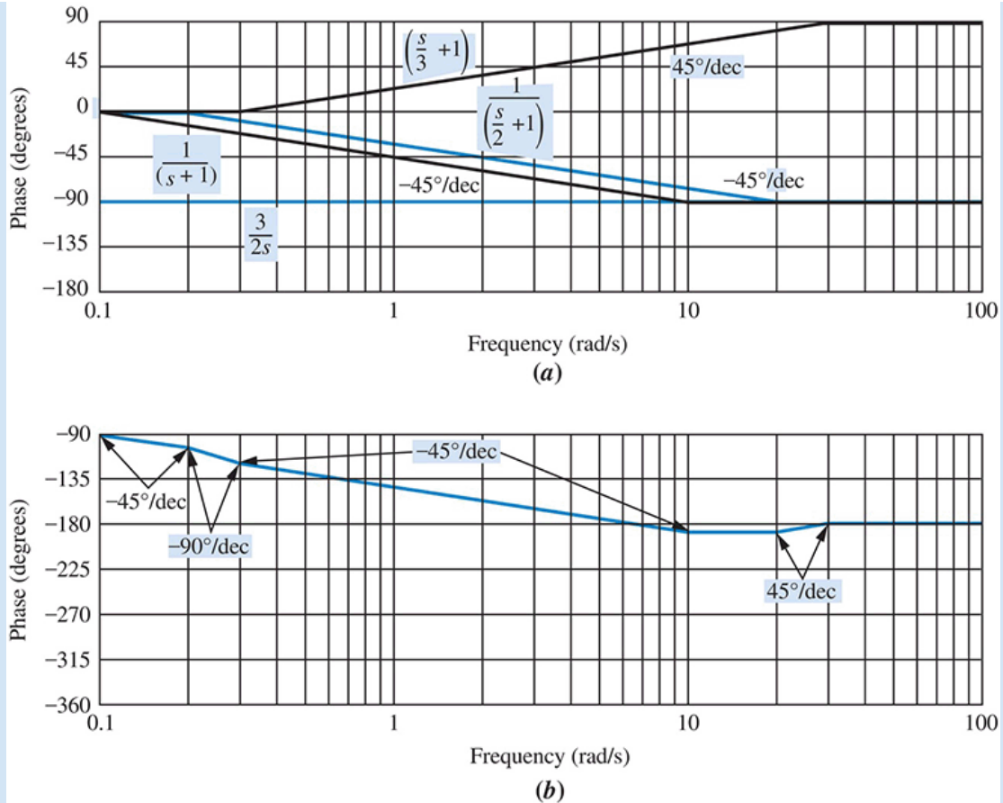
FIGURE 10.12 Bode phase plot for Example 10.2 :
