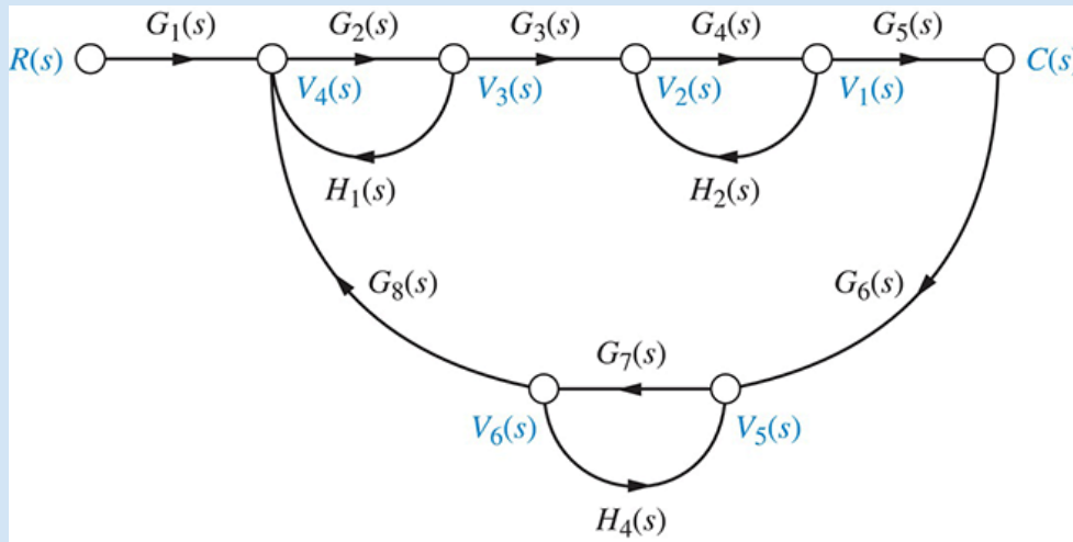
FIGURE 5.21 Signal-flow graph for Example 5.7 .
