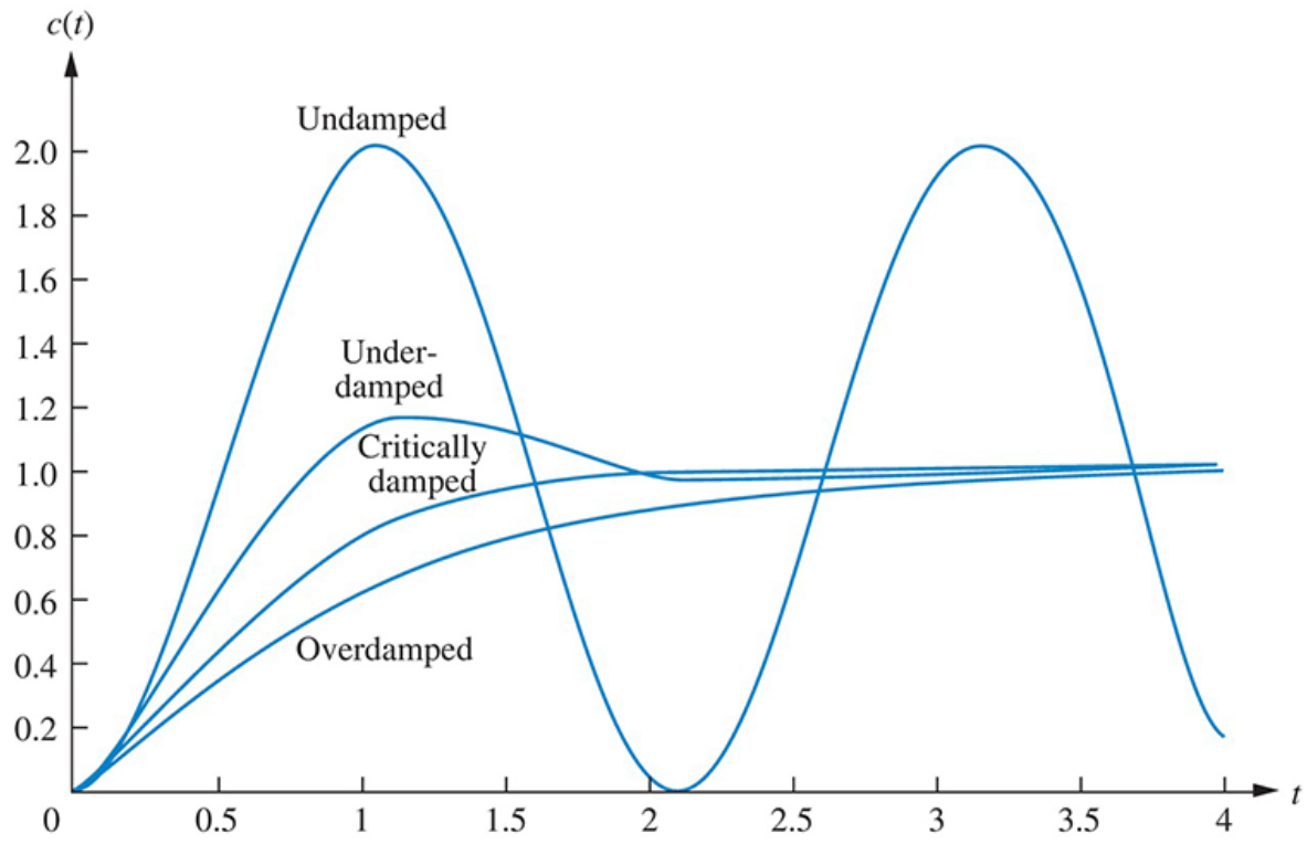
FIGURE 4.10 Step responses for second-order system damping cases
