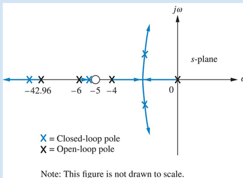
FIGURE 9.28 Compensated system root locus
