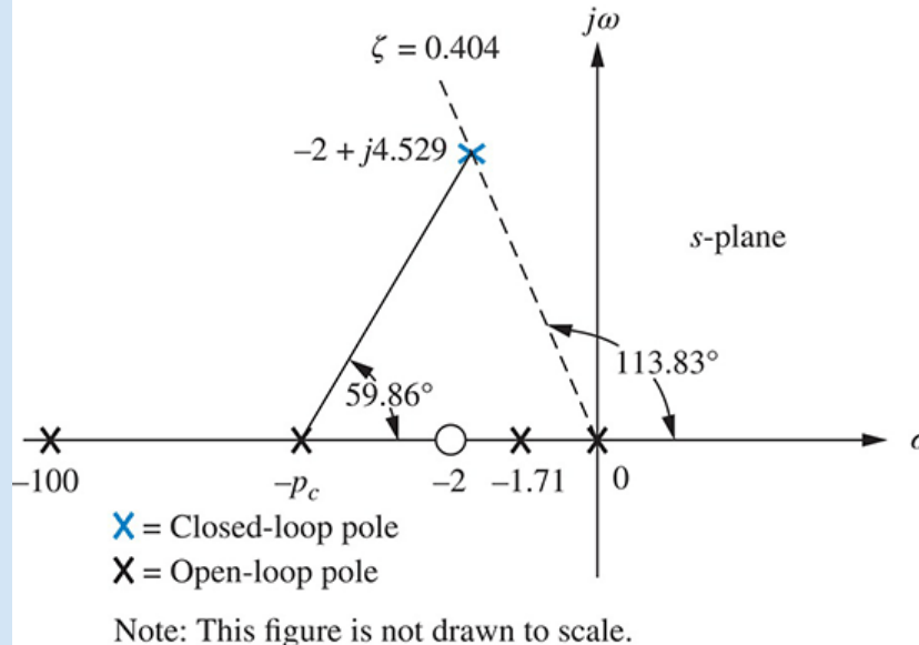
FIGURE 9.64 Locating compensator pole
