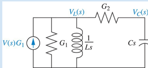
FIGURE 2.8 Transformed network ready for nodal analysis
