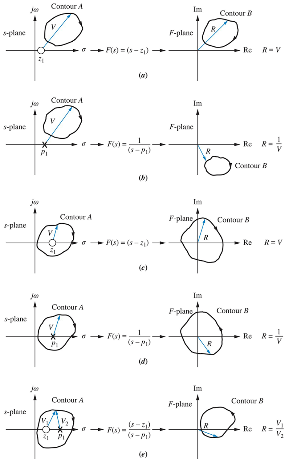
FIGURE 10.22 Examples of contour mapping
