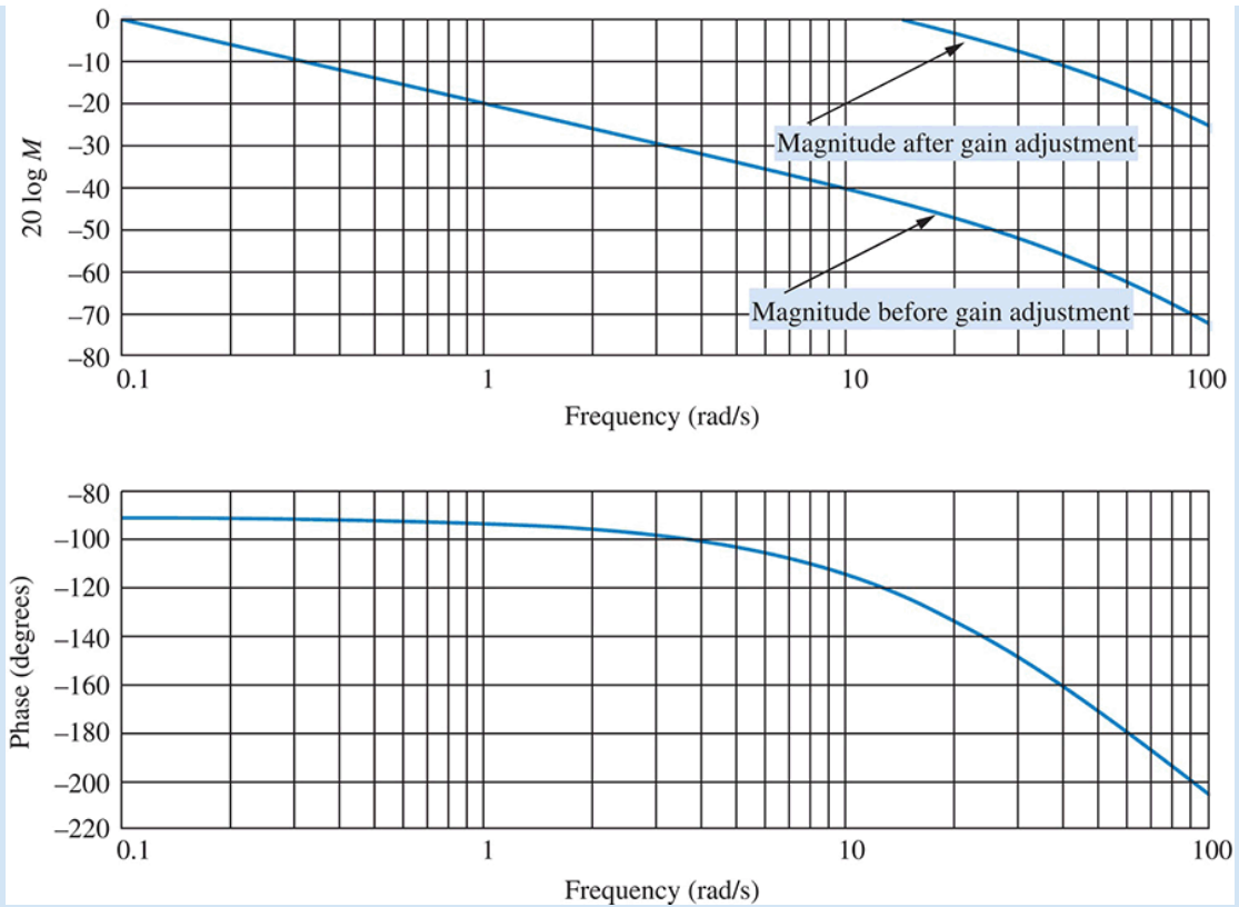
FIGURE 11.3 Bode magnitude and phase plots for Example 11.1
