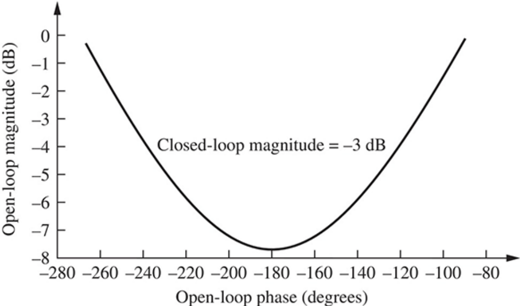
FIGURE 10.49 Open-loop gain vs. open-loop phase angle for -3 dB closed-loop gain
