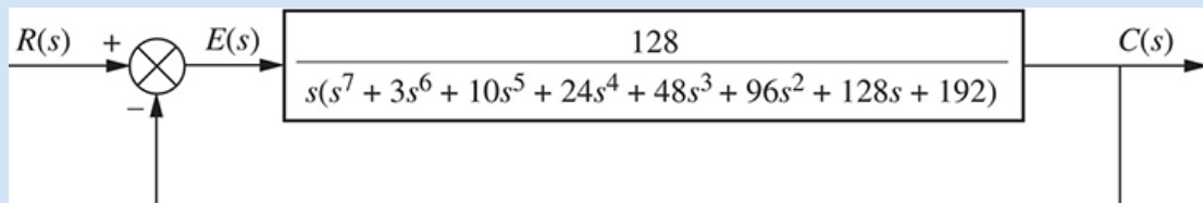
FIGURE 6.8 Feedback control system for Example 6.8
