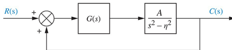
FIGURE P8.11 Linearized magnetic levitation system block diagram
