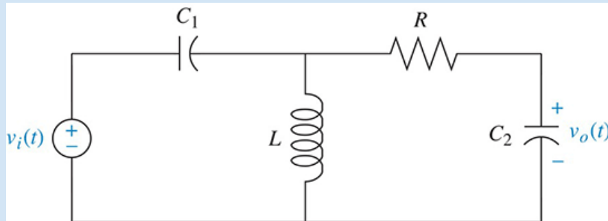
FIGURE 3.8 Electric circuit for Skill-Assessment Exercise 3.1
