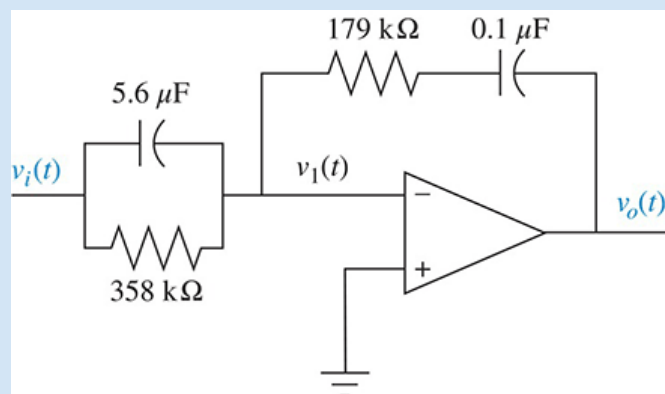
FIGURE 9.62 PID controller
