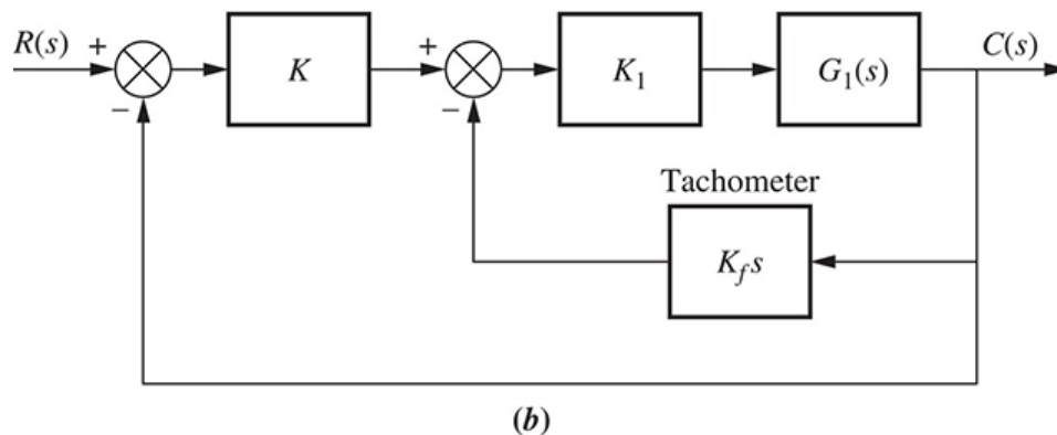
FIGURE 9.47 a. Transfer function of a tachometer; b. tachometer feedback compensation
