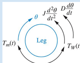
FIGURE 2.52 Free-body diagram of leg model
