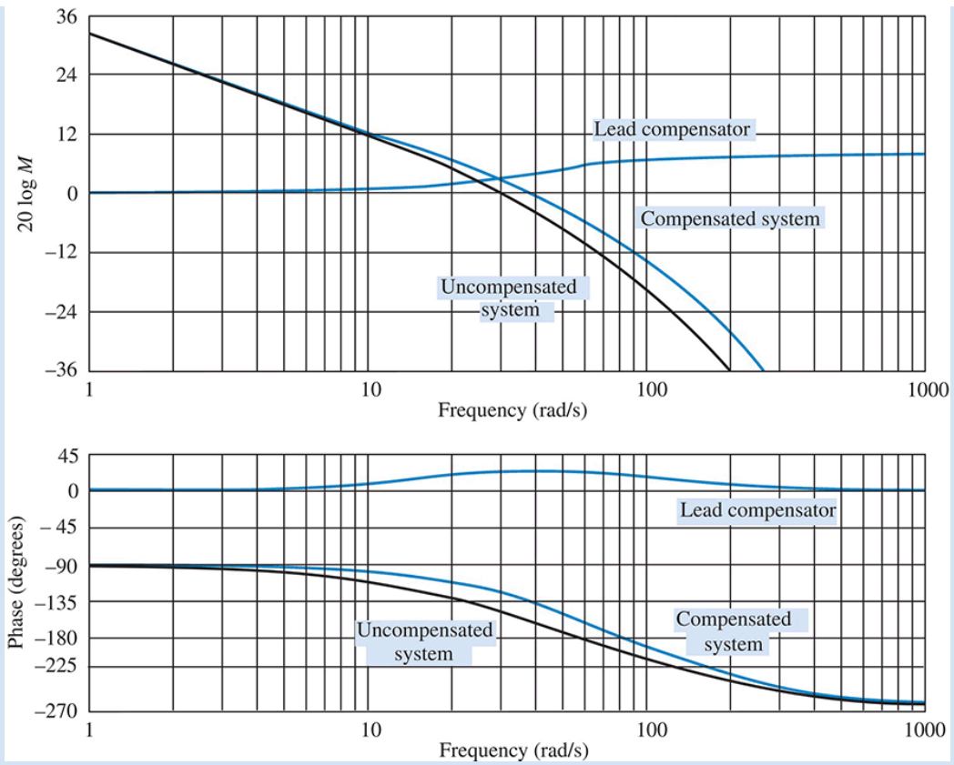
FIGURE 11.9 Bode plots for lead compensation in Example 11.3
