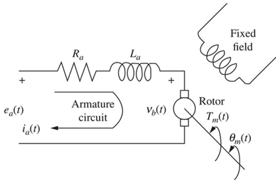
FIGURE I.4 DC motor circuit diagram
