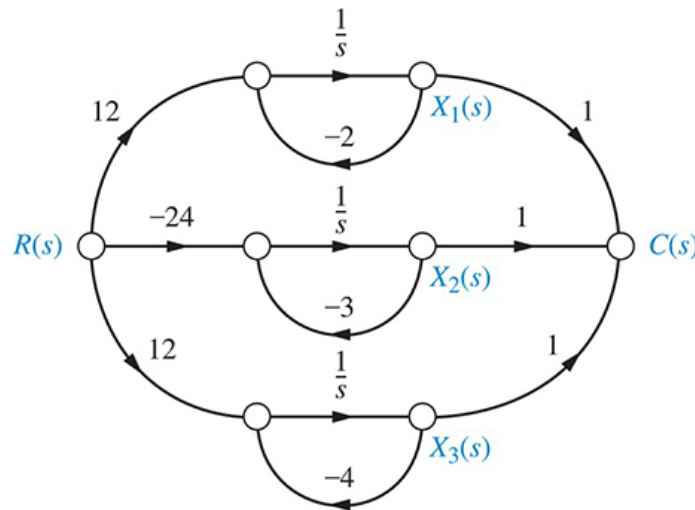
FIGURE 5.25 Signal-flow representation of Eq.(5.45) .
