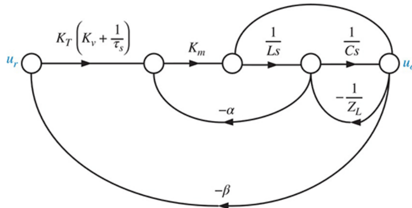
FIGURE P7.16 DVR Model
