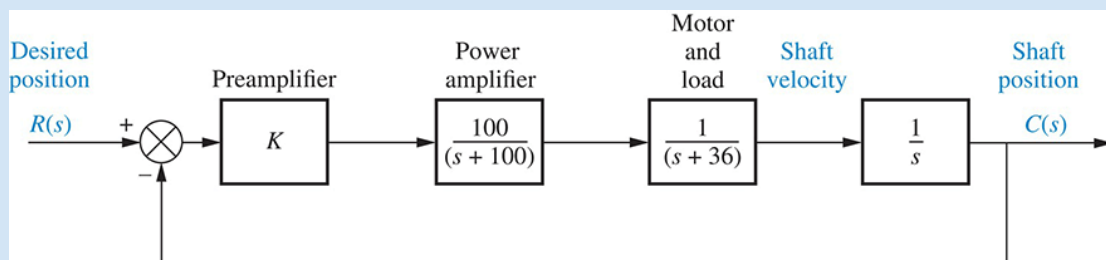
FIGURE 11.2 System for Example 11.1
