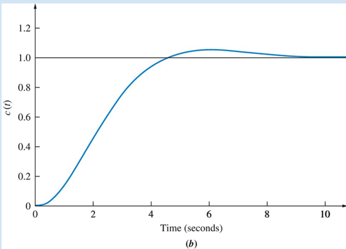
FIGURE 10.56 Step response for closed-loop system with G(s) = 5/[s(s + 1)(s + 10)] : a. with a 1-second delay; b. without delay
