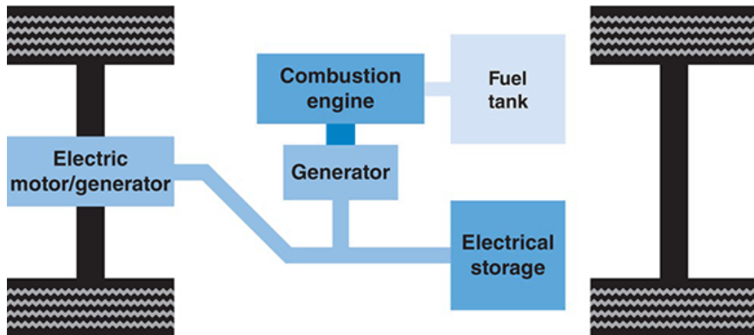
FIGURE P1.7 Serial hybrid-electric vehicle 5
