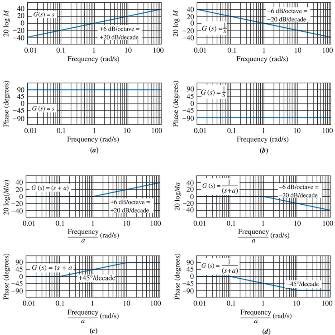
FIGURE 10.9 Normalized and scaled Bode plots for
