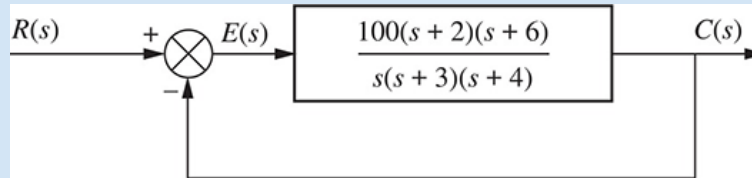
FIGURE 7.6 Feedback control system for Example 7.3
