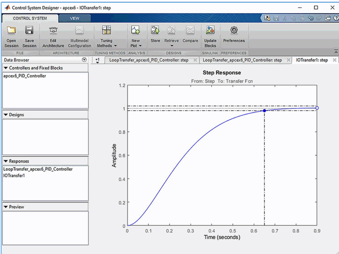
FIGURE C.29 Final designed response showing settling time
