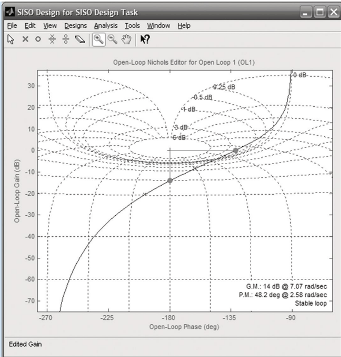
FIGURE 11.13 Nichols chart after gain adjustment
