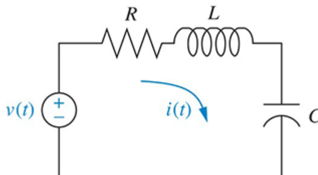
FIGURE P1.6 RLC network
