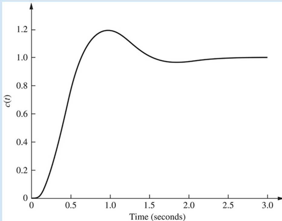
FIGURE 9.51 Step response for uncompensated system of Example 9.7
