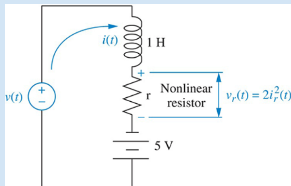
FIGURE 2.53 Nonlinear electric circuit
