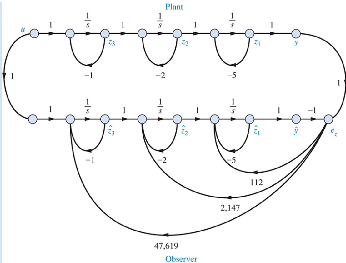
FIGURE 12.18 Observer design
