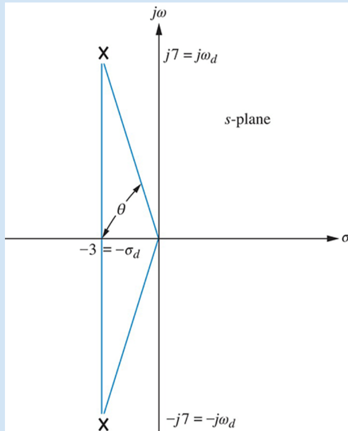
FIGURE 4.20 Pole plot for Example 4.8
