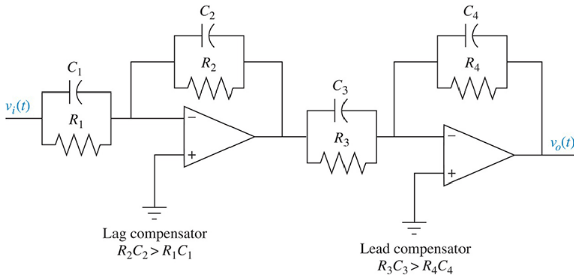
FIGURE 9.61 Lag-lead compensator implemented with operational amplifiers
