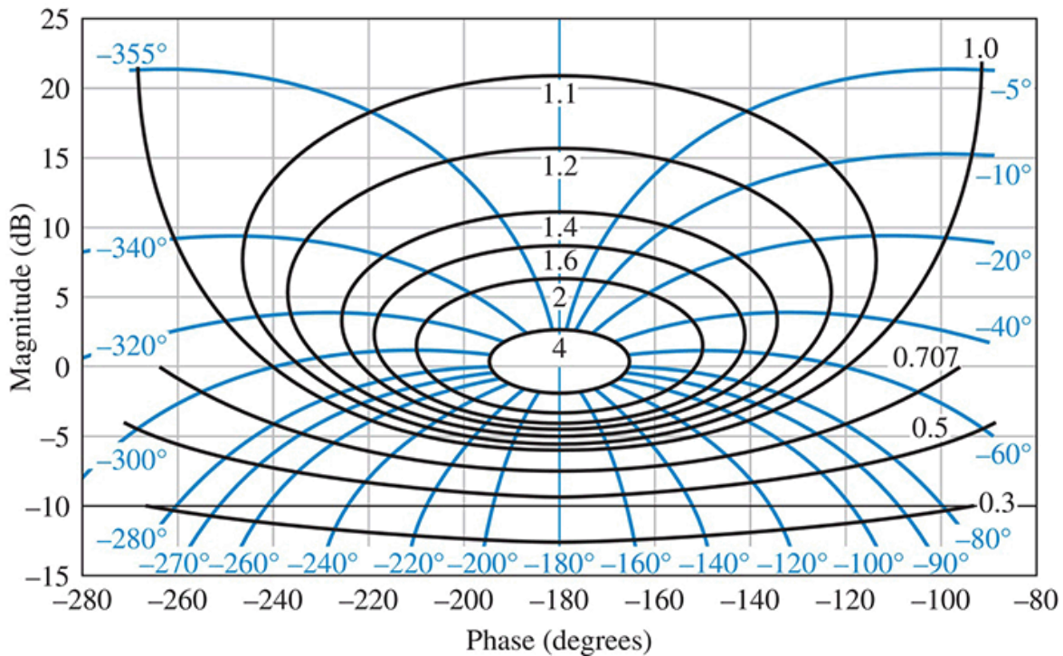
FIGURE 10.46 Nichols chart
