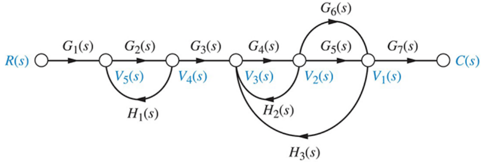
FIGURE 5.20 Signal-flow graph for demonstrating Mason's rule
