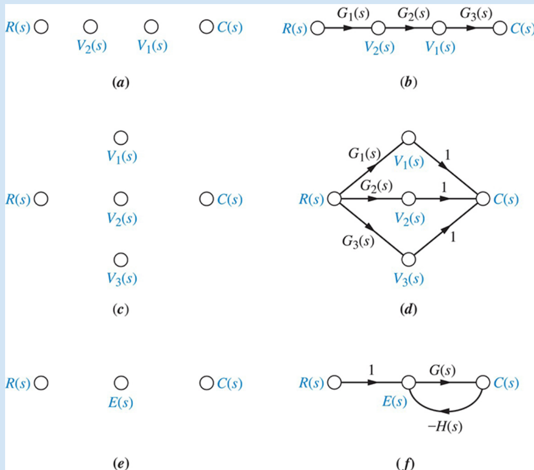
FIGURE 5.18 Building signal-flow graphs: a. cascaded system nodes (from Figure 5.3(a) ); b. cascaded system signal-flow graph; c. parallel system nodes (from Figure 5.5(a) ); d. parallel system signal-flow graph; e. feedback system nodes (from Figure 5.6(b) ); f. feedback system signal-flow graph
