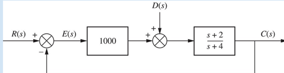
FIGURE 7.14 System for Skill-Assessment Exercise 7.4
