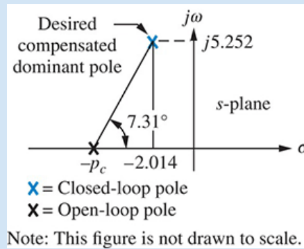
FIGURE 9.27 s -plane picture used to calculate the location of the compensator pole for Example 9.4 .
