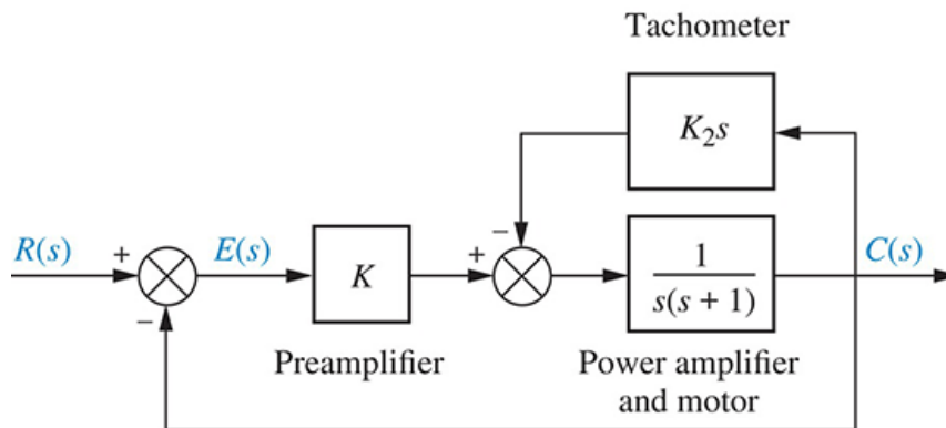
FIGURE P5.35 Position control
