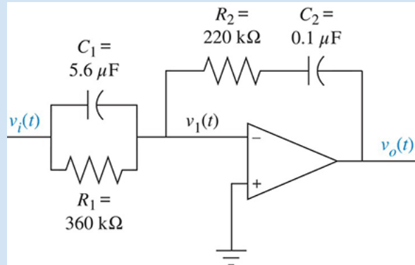
FIGURE 2.11 Inverting operational amplifier circuit for Example 2.14 .
