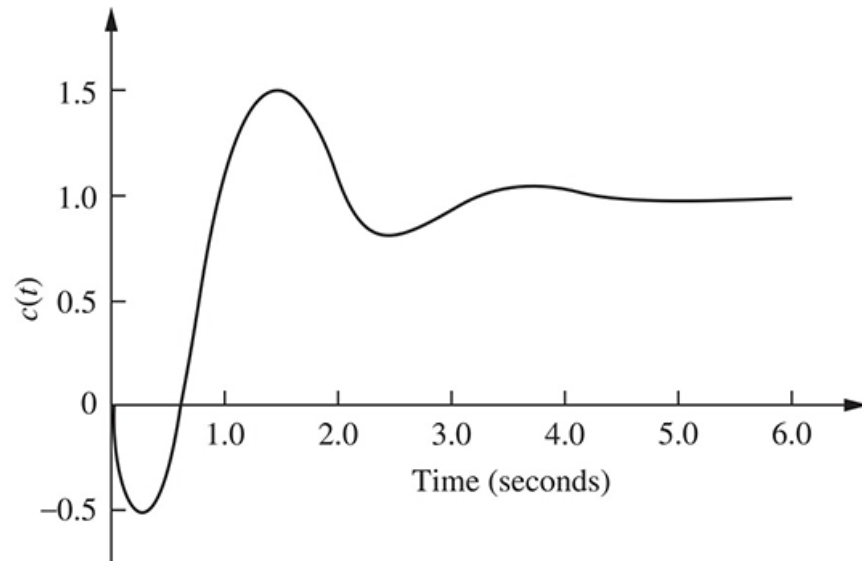
FIGURE 4.26 Step response of a nonminimum-phase system
