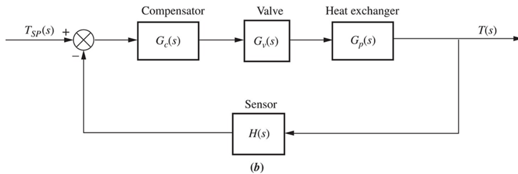
FIGURE P9.4 a. Heat-exchanger process; b. block diagram
