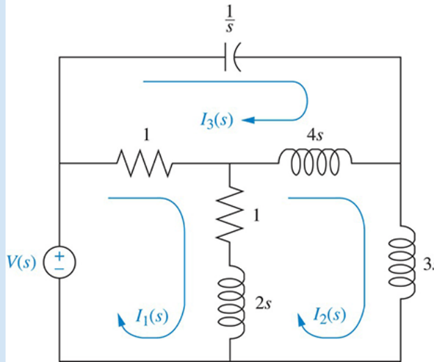
FIGURE 2.9 Three-loop electrical network
