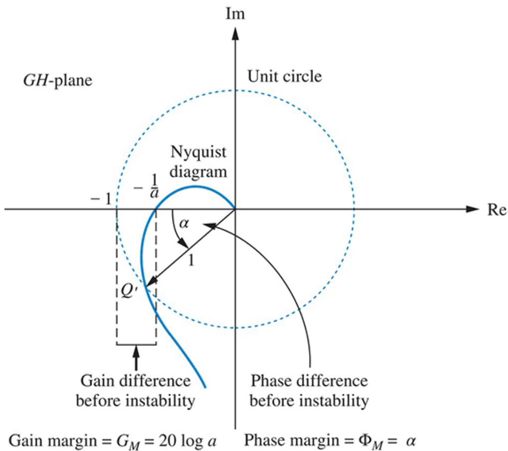
FIGURE 10.35 Nyquist diagram showing gain and phase margins
