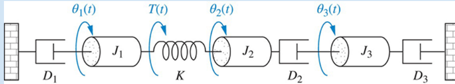
FIGURE 2.25 Three-degrees-of-freedom rotational system
