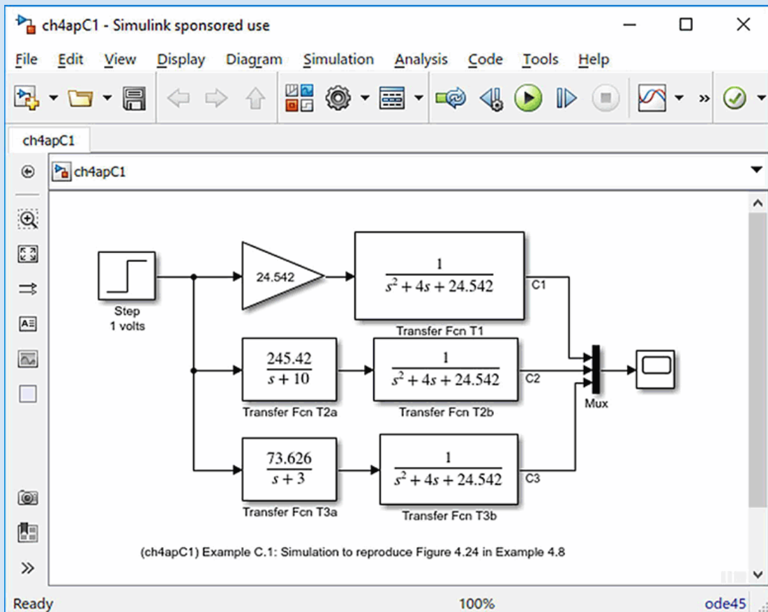
FIGURE C.5 Simulink block diagram for Example C.1
