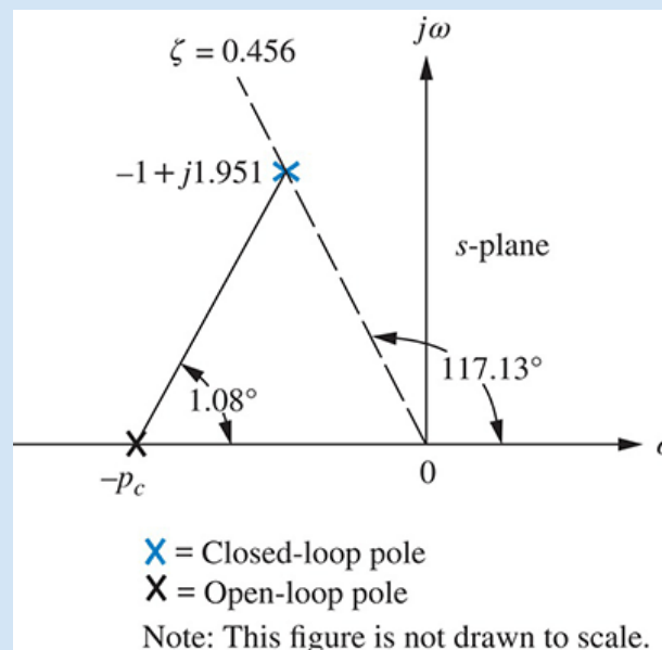
FIGURE 9.67 Locating compensator pole
