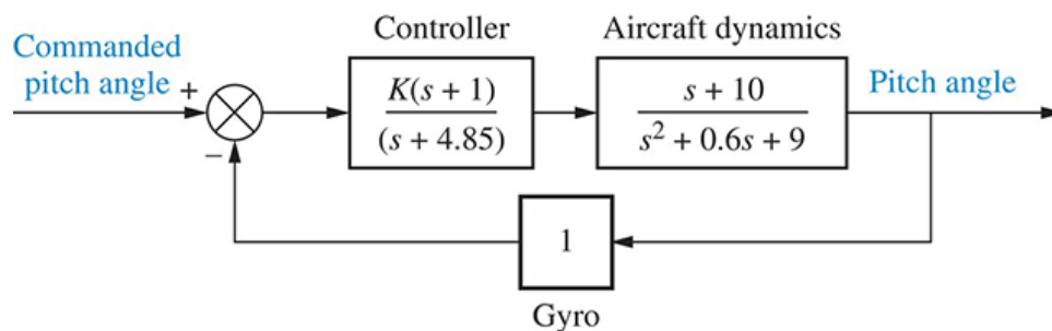
FIGURE P6.10 Aircraft pitch loop model
