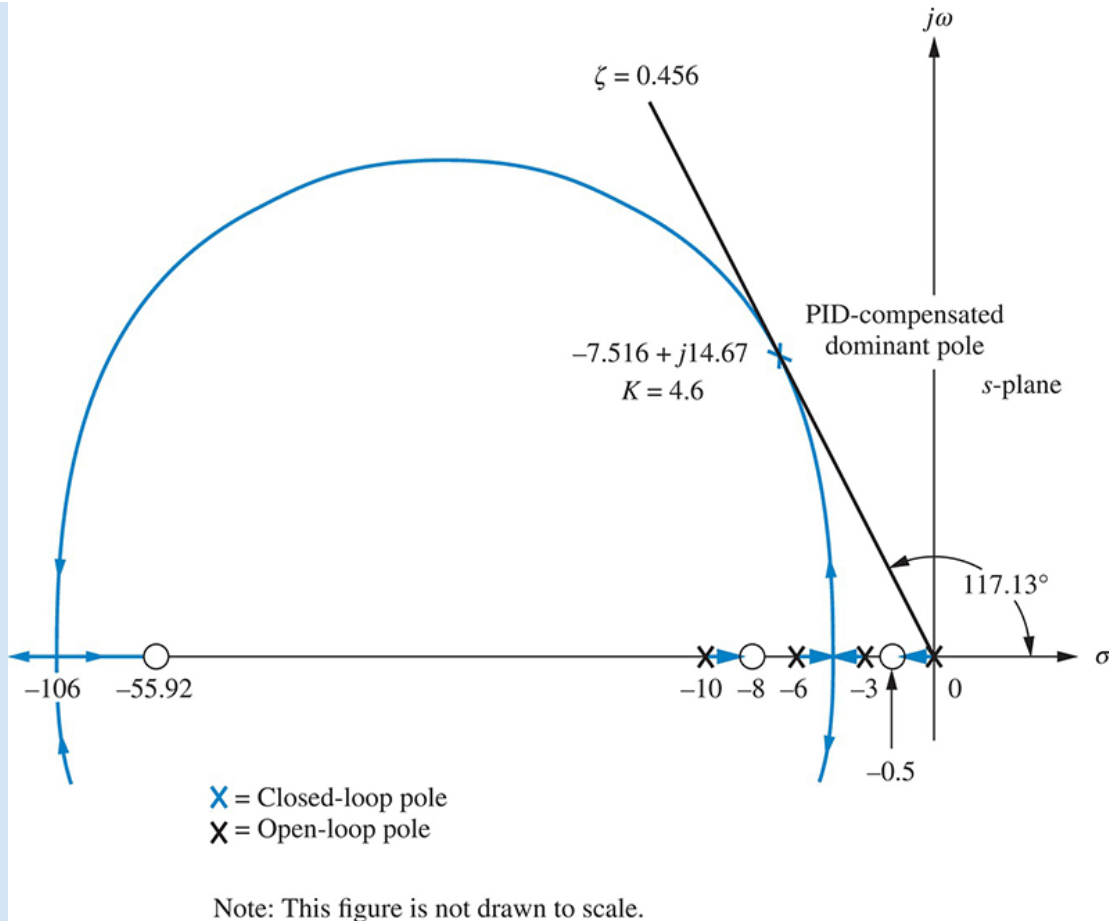
FIGURE 9.36 Root locus for PID-compensated system of Example 9.5
