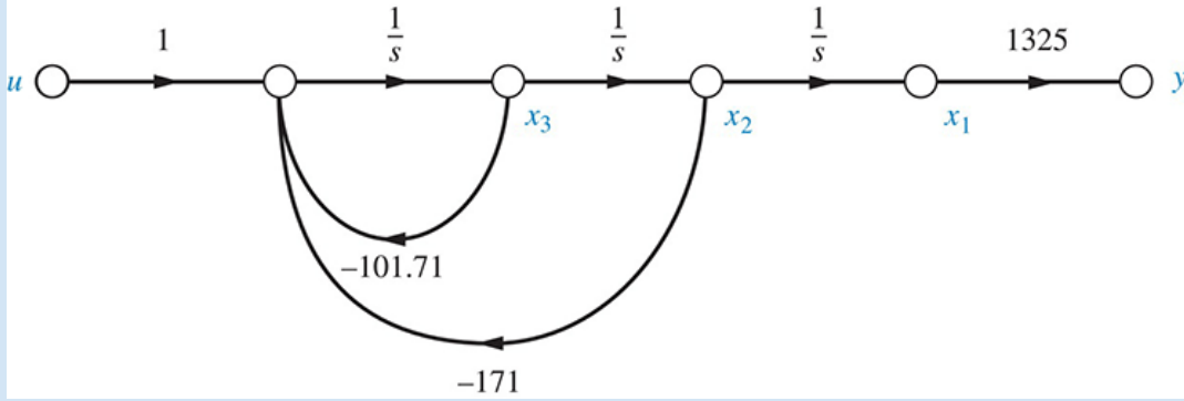
FIGURE 12.24 Signal-flow graph for G(s) = 1325 / [s(s^2 + 101.71s + 171)]
