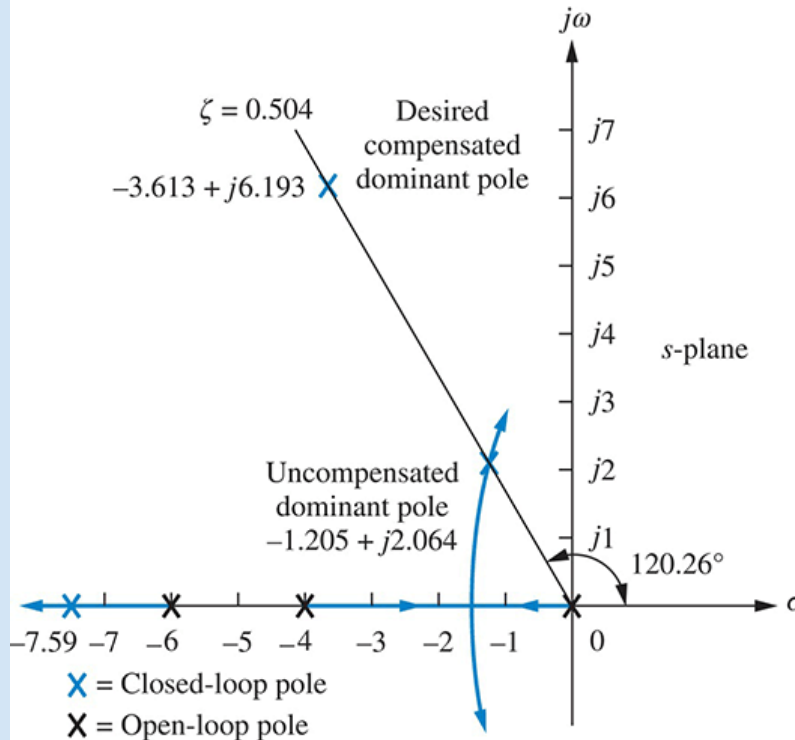
FIGURE 9.19 Compensated dominant pole superimposed over the uncompensated root locus for Example 9.3
