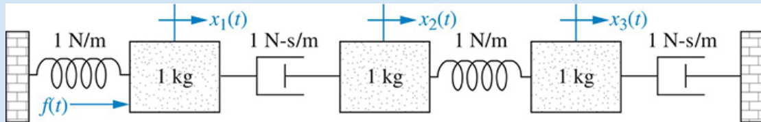
FIGURE 3.9 Translational mechanical system for Skill-Assessment Exercise 3.2
