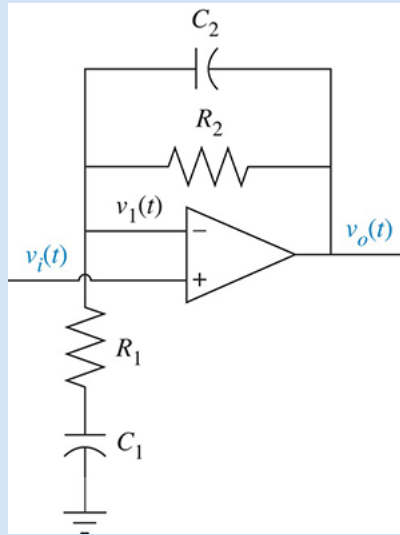
FIGURE 2.13 Noninverting operational amplifier circuit for Example 2.15
