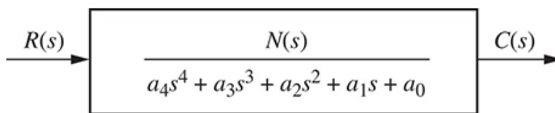
FIGURE 6.3 Equivalent closed-loop transfer function
