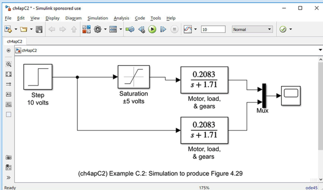
FIGURE C.10 Simulink block diagram for Example C.2
