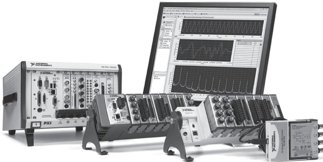
FIGURE 10.1 National Instruments PXI, Compact RIO, Compact DAQ, and USB hardware platforms (shown from left to right) coupled with NI LabVIEW software to provide stimulus and acquire signals from physical systems. NI LabVIEW can then be used to analyze data, determine the mathematical model, and prototype and deploy a controller for the physical system
