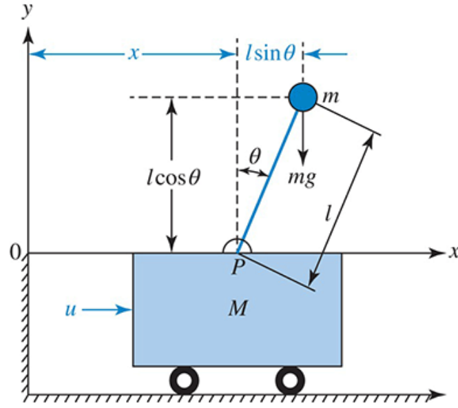
FIGURE P3.15 Motor-driven inverted pendulum cart system 6
