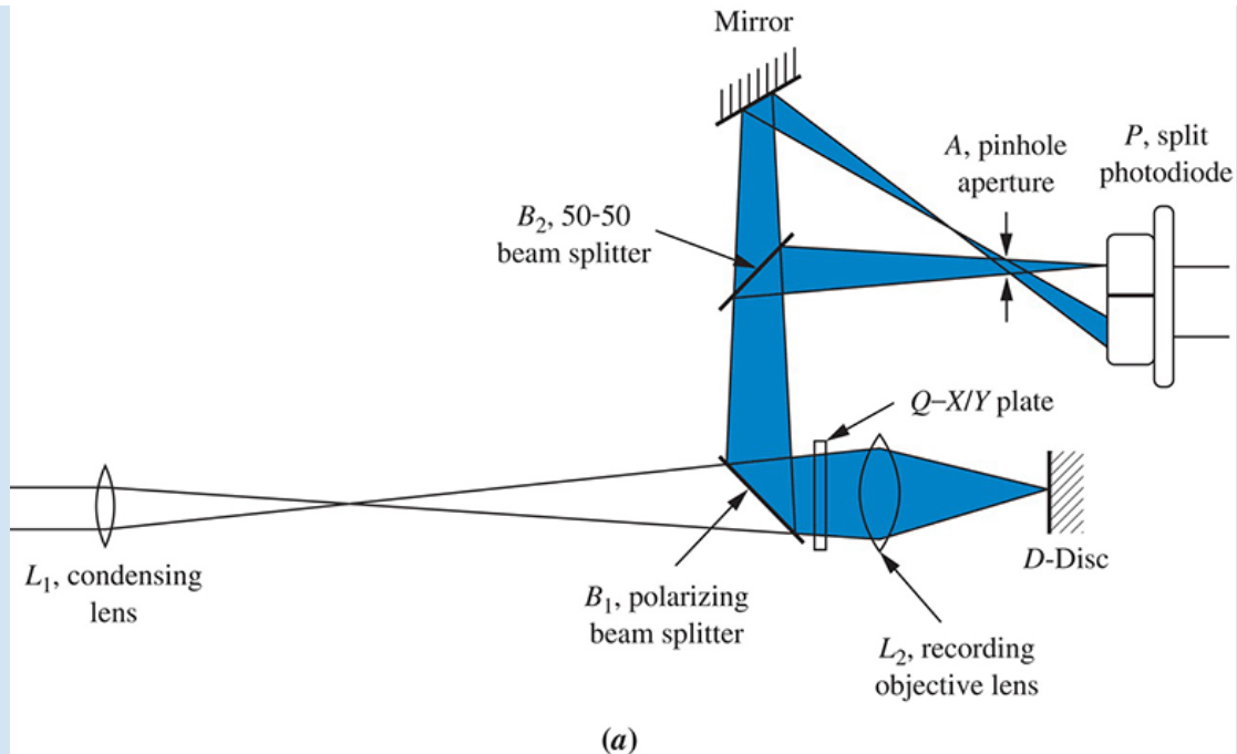
FIGURE 7.23 Video laser disc recording: a. focus detector optics 6 ; b. linearized transfer function for focus detector 6
