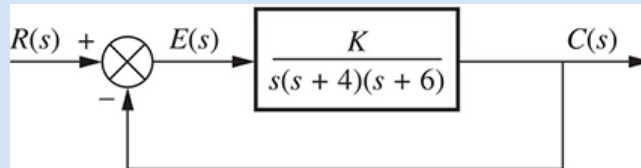
FIGURE 9.17 Feedback control system for Example 9.3
