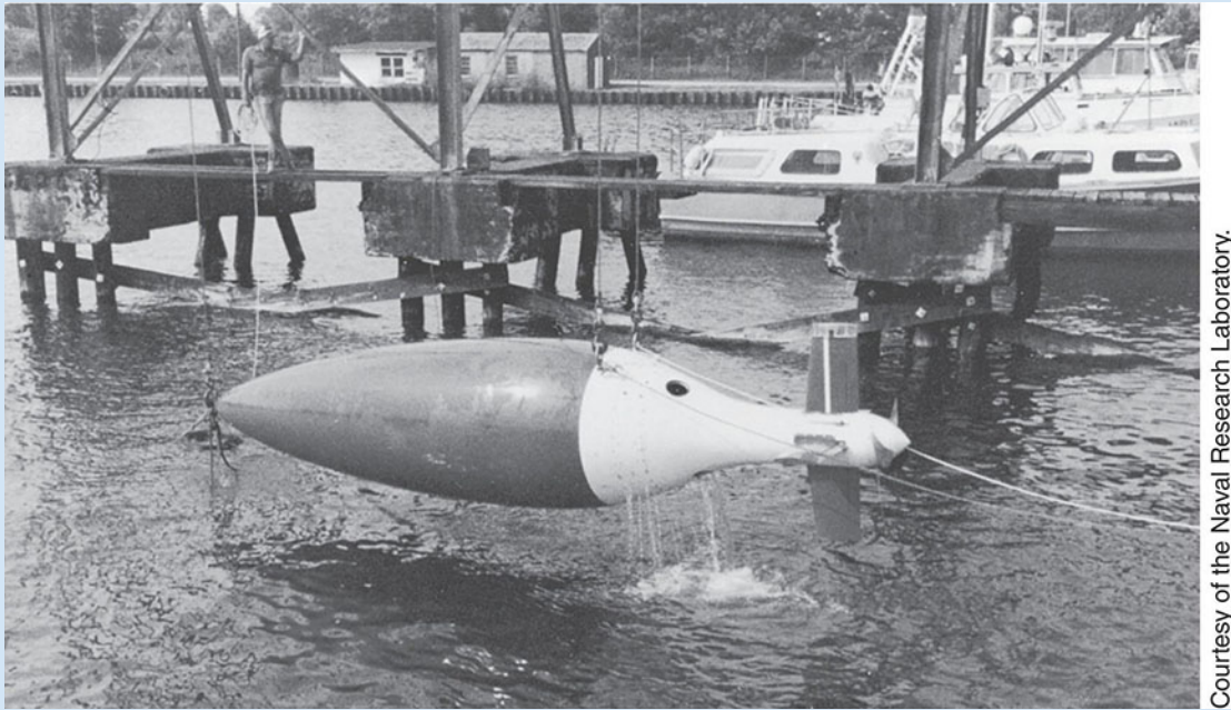
FIGURE 4.33 Unmanned Free-Swimming Submersible (UFSS) vehicle
