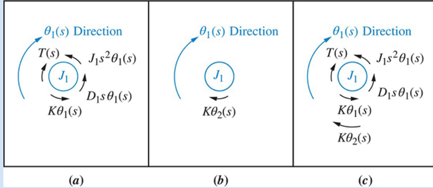
FIGURE 2.23 a. Torques on J_1 due only to the motion of J_1 ; b. torques on J_1 due only to the motion of J_2 ; c. final free-body diagram for J_1
