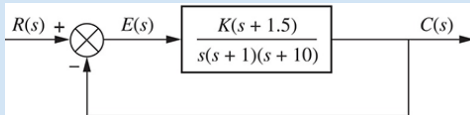
FIGURE 8.21 System for Example 8.8
