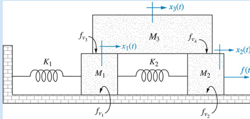
FIGURE 2.20 Three-degrees-of-freedom translational mechanical system
