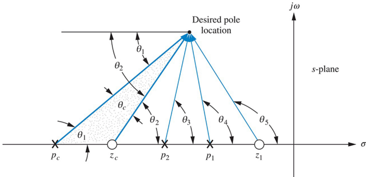
FIGURE 9.24 Geometry of lead compensation
