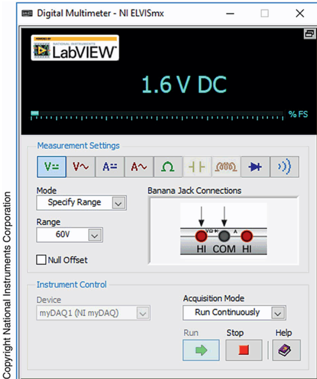
FIGURE D.28 Battery voltage measurement: a. Connections to myDAQ; b. DMM reading
