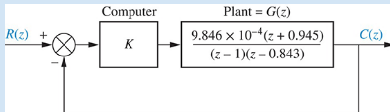
FIGURE 13.31 Analog antenna azimuth position control system is converted to a digital system.
