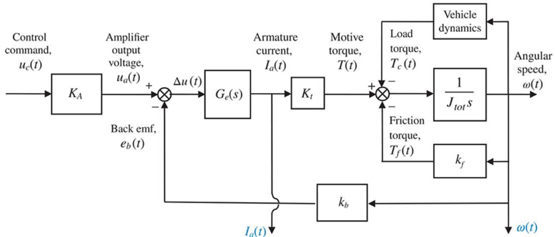
FIGURE P3.16 Block diagram representation of an HEV forward path 8
