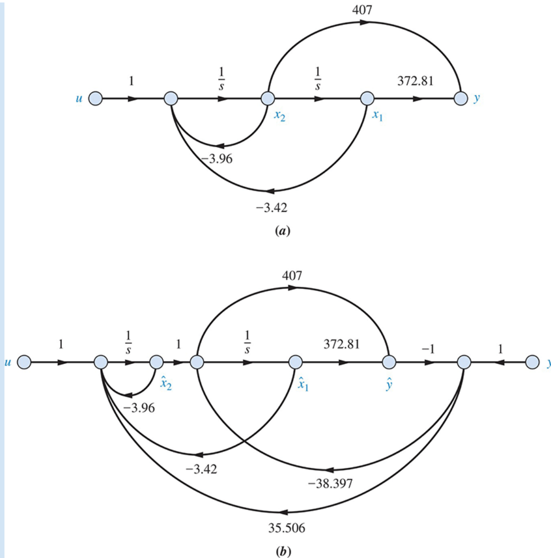
FIGURE 12.20 a. Plant; b. designed observer for Example 12.9 .
