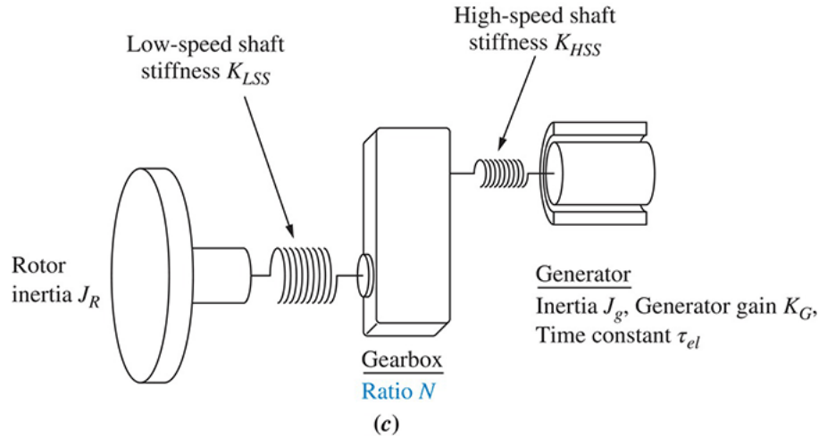
FIGURE P8.15 a. Wind turbines generating electricity near Palm Springs, California; b. control loop for a constant-speed pitch-controlled wind turbine; 3 c. drivetrain 3
