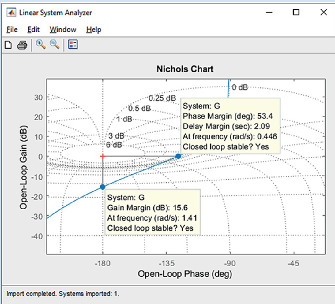
FIGURE E.5 Linear System Analyzer used for Nichols chart: a. M-file; b. Linear System Analyzer
