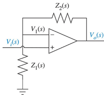
FIGURE 2.12 General noninverting operational amplifier circuit
