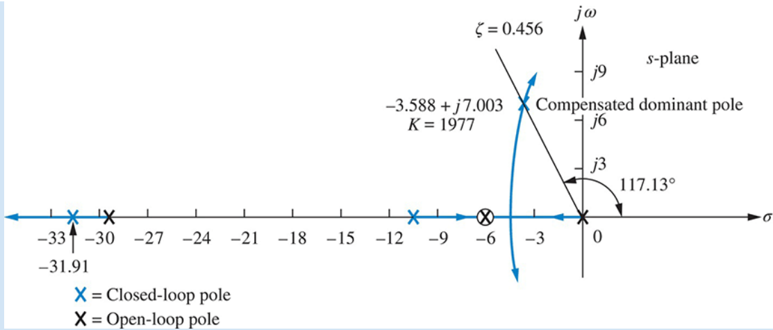
FIGURE 9.40 Root locus for lead-compensated system of Example 9.6
