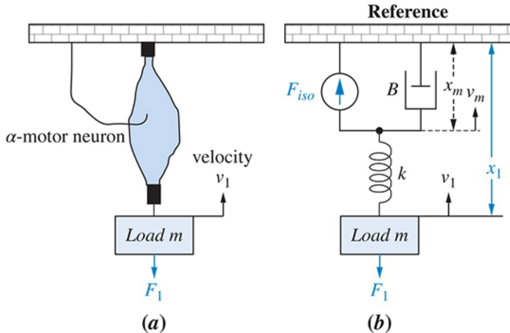
FIGURE P2.26 a. Motor neuron stimulating a muscle; 1 b. equivalent circuit 2
