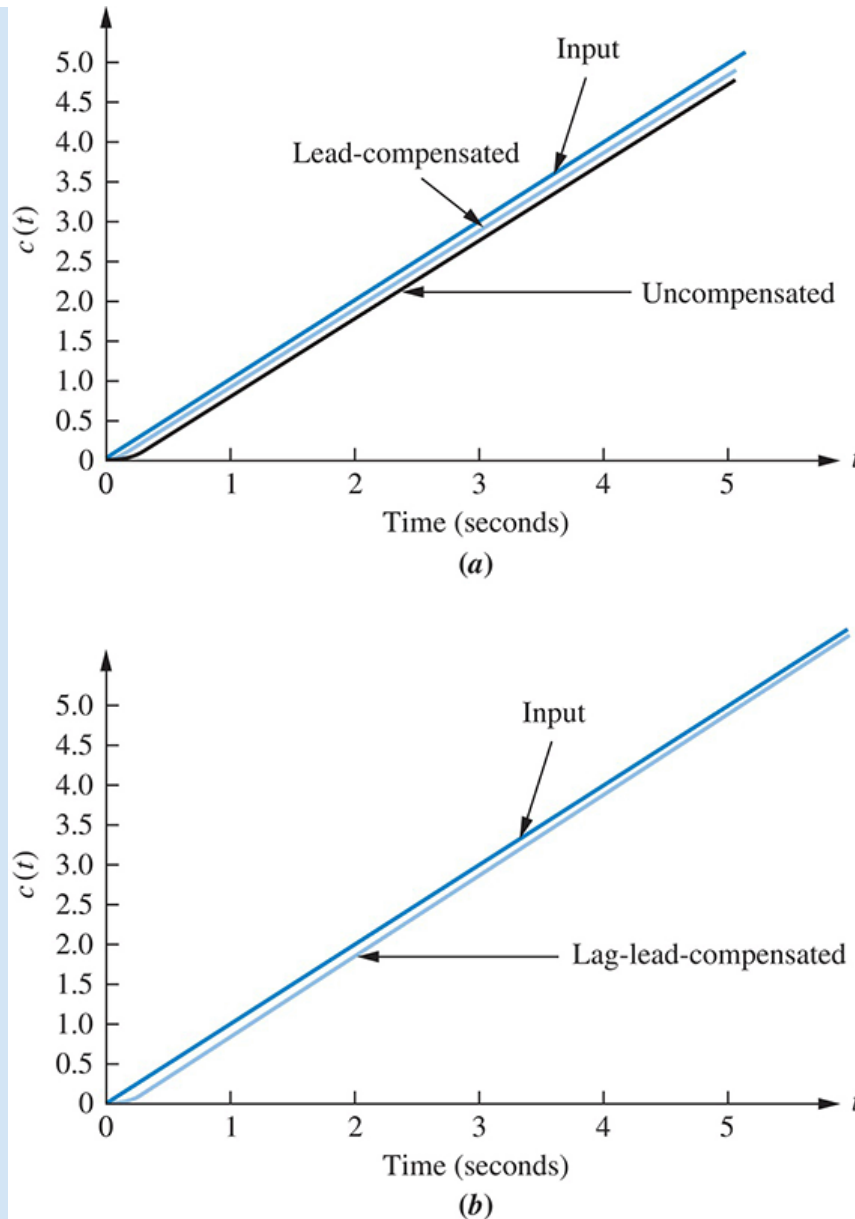
FIGURE 9.43 Improvement in ramp response error for the system of Example 9.6 : a. lead-compensated; b. lag-lead-compensated
