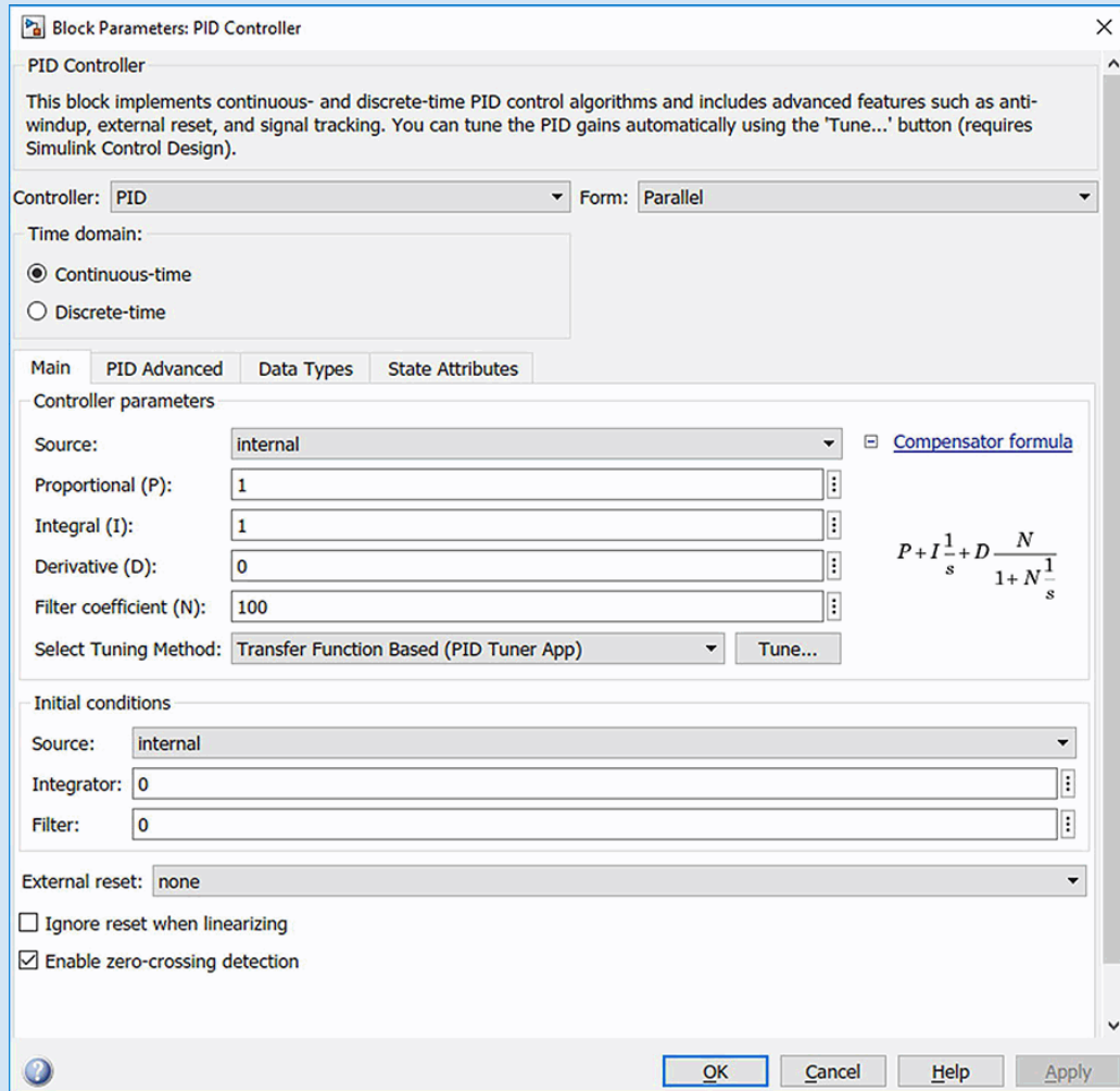
FIGURE C.20 Block Parameters window for the PID controller
