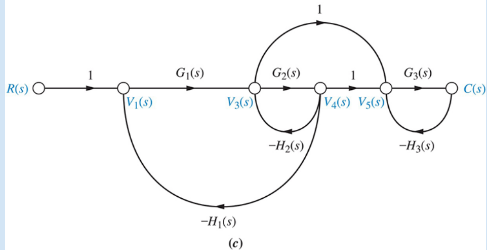
FIGURE 5.19 Signal-flow graph development: a. signal nodes; b. signal-flow graph; c. simplified signal-flow graph
