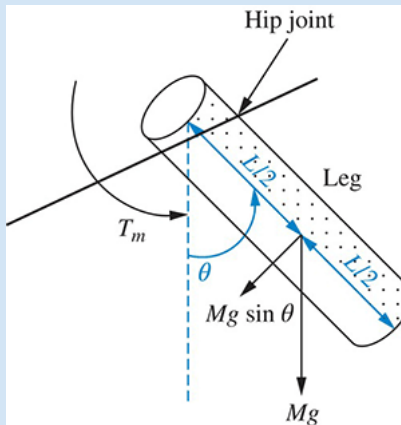
FIGURE 2.51 Cylinder model of a human leg
