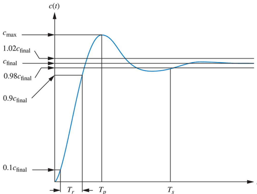
FIGURE 4.14 Second-order underdamped response specifications
