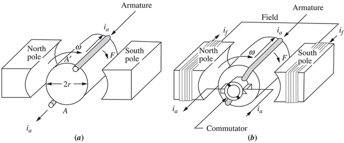
FIGURE I.2 a. Current-carrying wire on a rotor; b. current-carrying wire on a rotor with commutation and coils added to the permanent magnets to increase magnetic field strength
