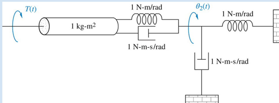
FIGURE 2.26 Rotational mechanical system for Skill-Assessment Exercise 2.9 .
