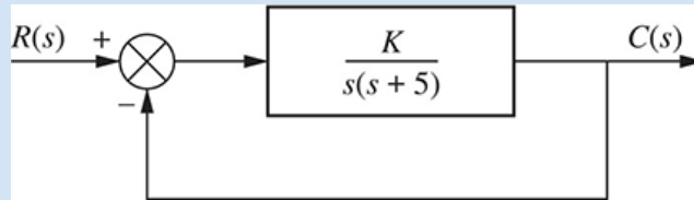
FIGURE 5.16 Feedback system for Example 5.4 .
