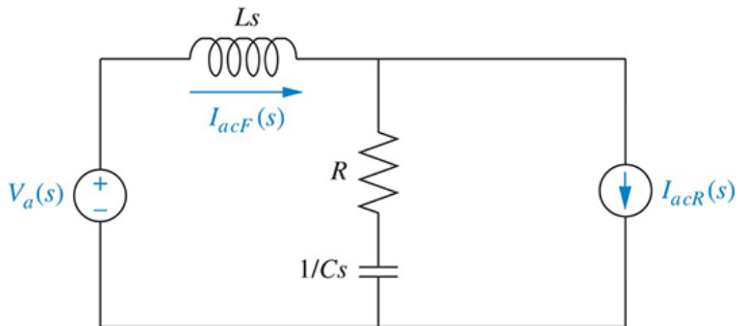
FIGURE P2.27 AC filter equivalent circuit for a three-phase ac/dc converter
