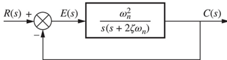
FIGURE 10.38 Second-order closed-loop system
