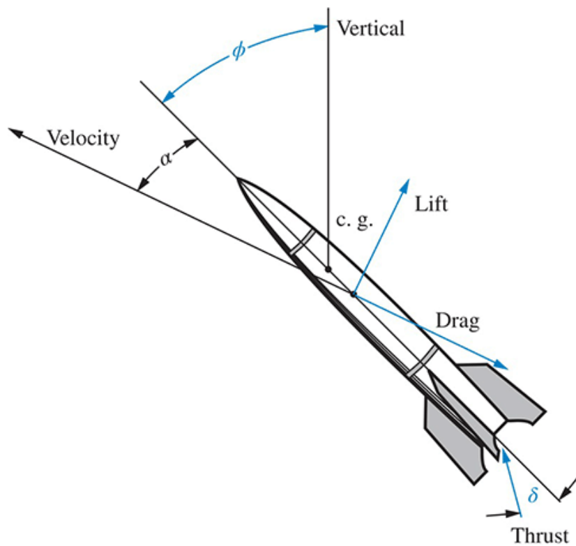
FIGURE P3.9 Missile
