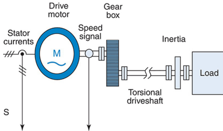
FIGURE P4.13 Partial topology of a typical motor drive system 3
