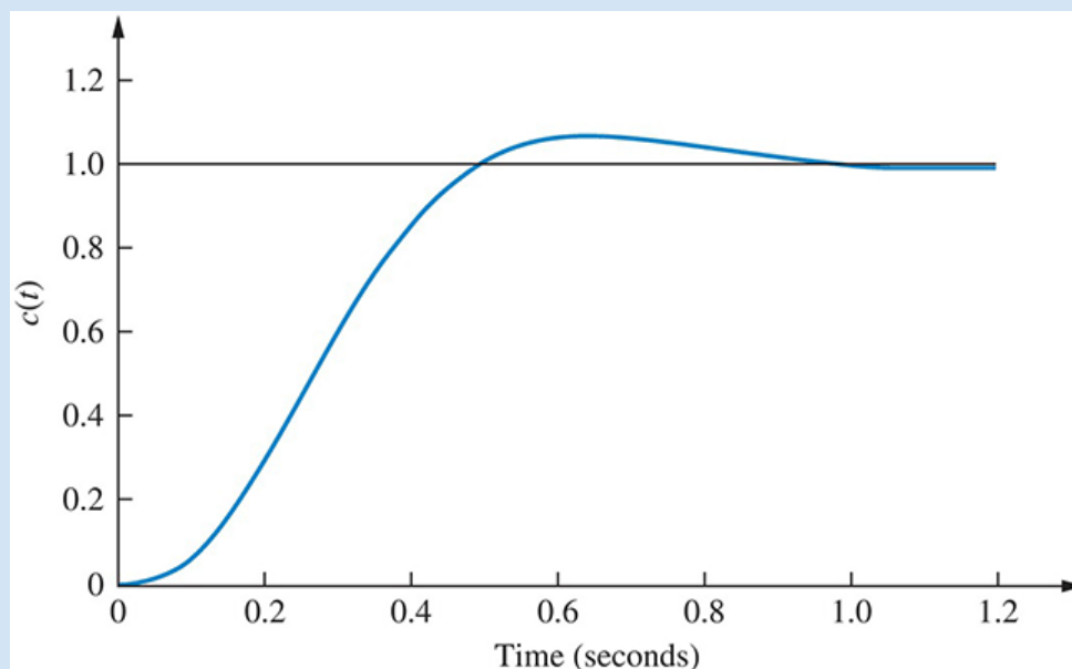
FIGURE 9.58 Step response simulation for Example 9.8
