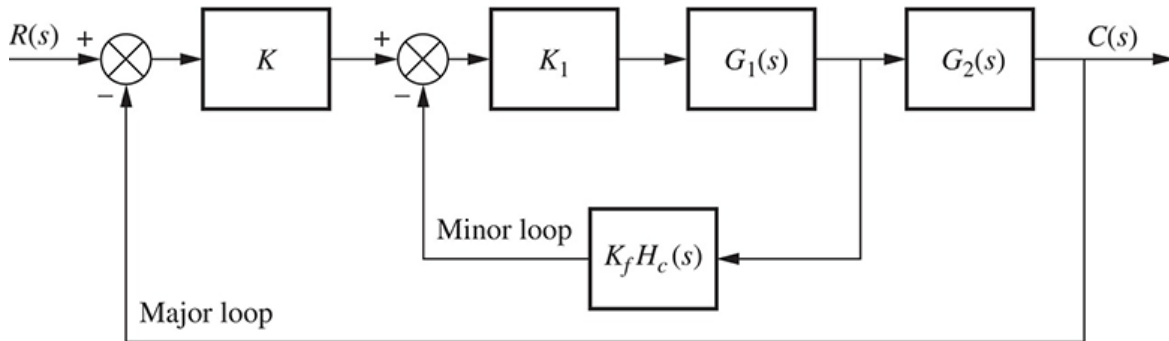
FIGURE 9.45 Generic control system with feedback compensation.
