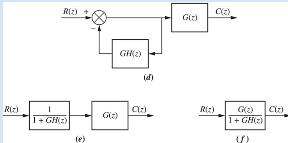
FIGURE 13.10 Steps in block diagram reduction of a sampled-data system
