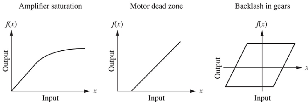
FIGURE 2.46 Some physical nonlinearities
