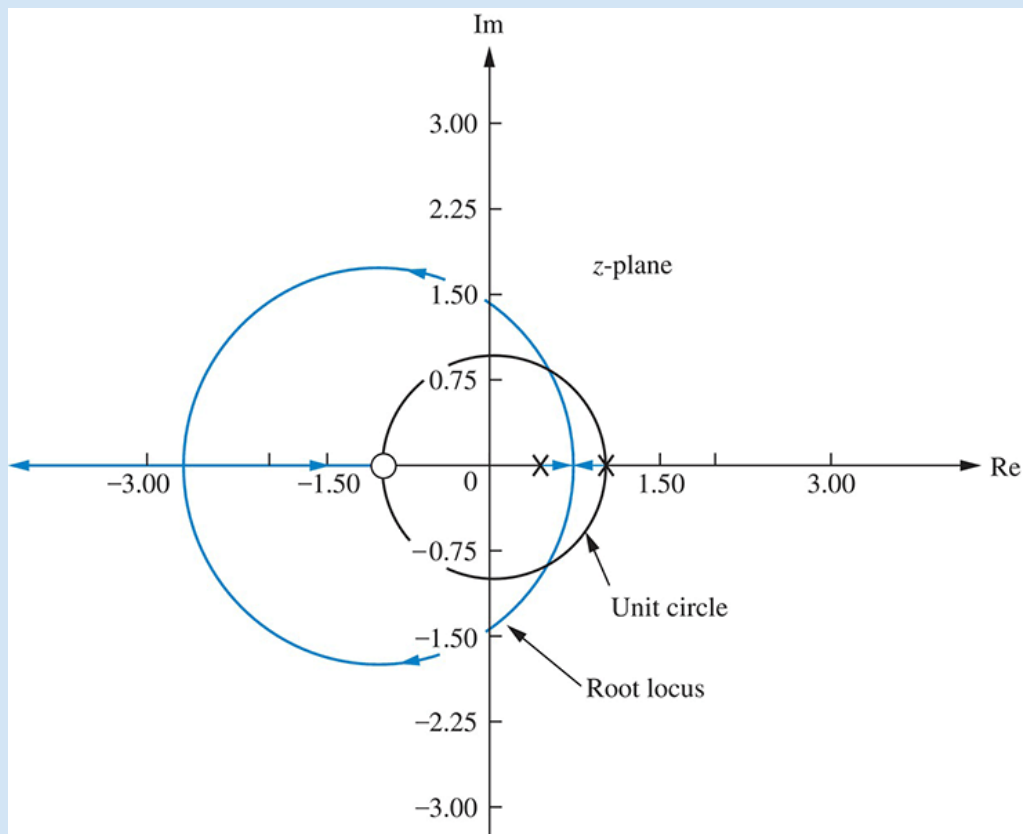
FIGURE 13.22 Root locus for the system of Figure 13.21
