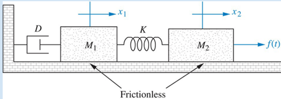
FIGURE 3.7. Translational mechanical system
