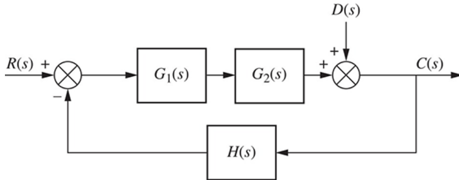
FIGURE P7.17 System with input and disturbance
