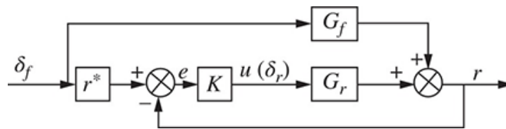
FIGURE P7.20 Steering model for a four-wheel drive vehicle 1
