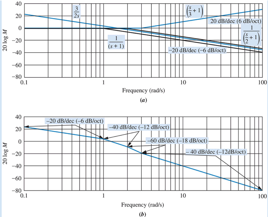
FIGURE 10.11 Bode log-magnitude plot for Example 10.2 :
