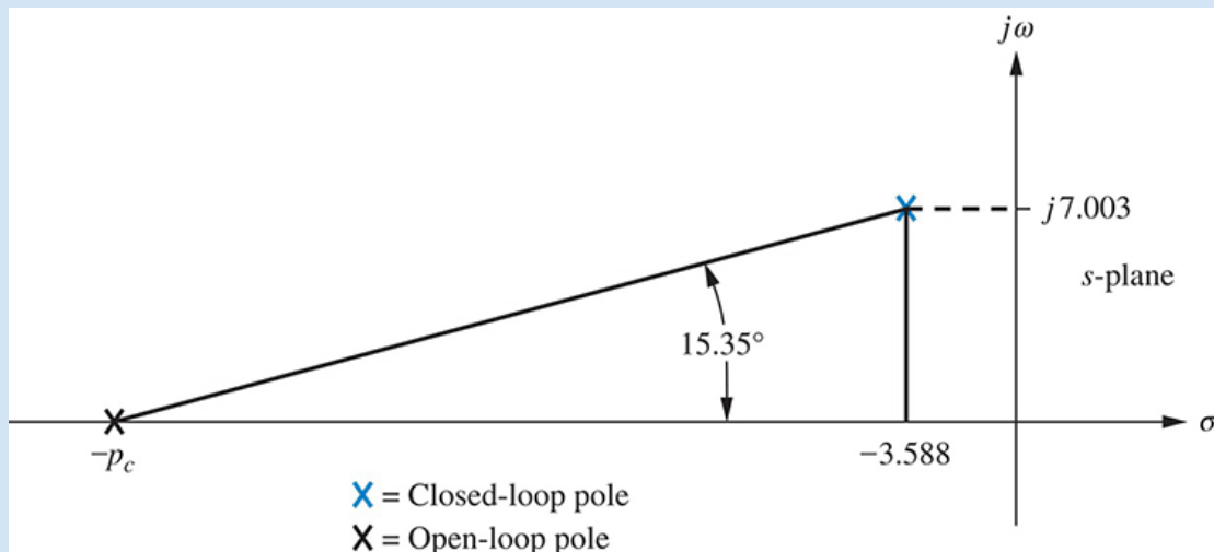
FIGURE 9.39 Evaluating the compensator pole for Example 9.6
