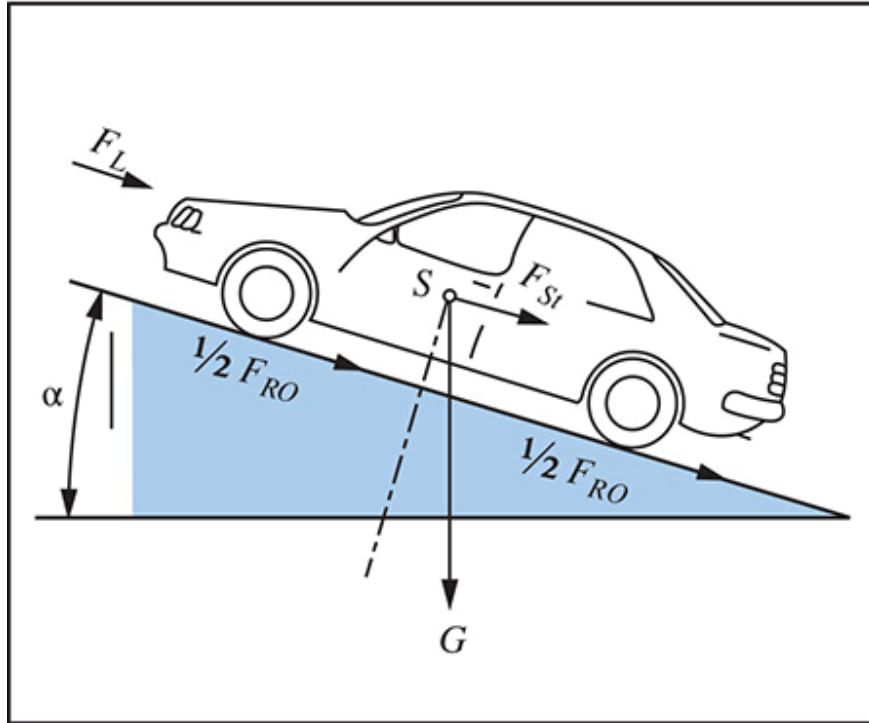
FIGURE P2.29 Running resistances 4
