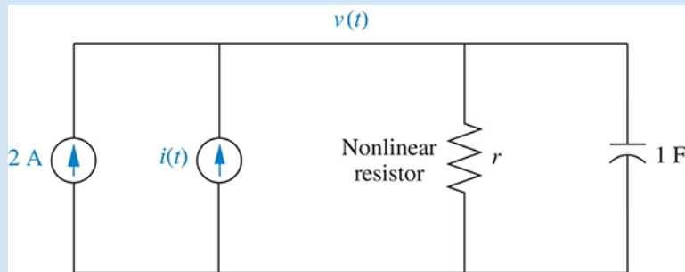
FIGURE 2.50 Nonlinear electric circuit for Skill-Assessment Exercise 2.13
