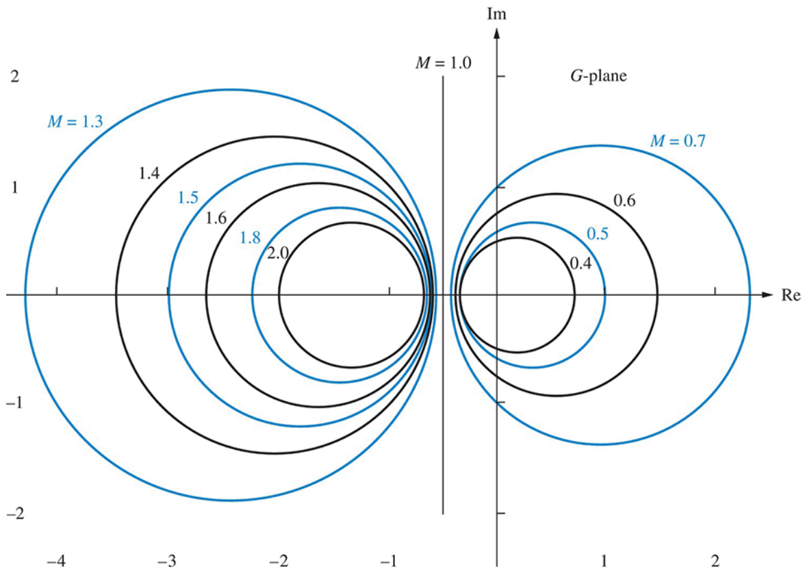
FIGURE 10.42 Constant M circles
