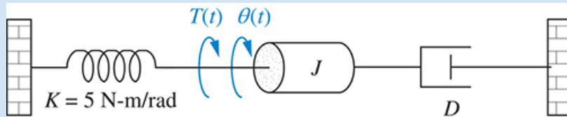
FIGURE 4.21 Rotational mechanical system for Example 4.7 .
