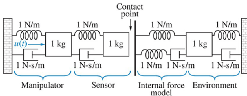
FIGURE P3.12 Robotic manipulator and target environment 2
