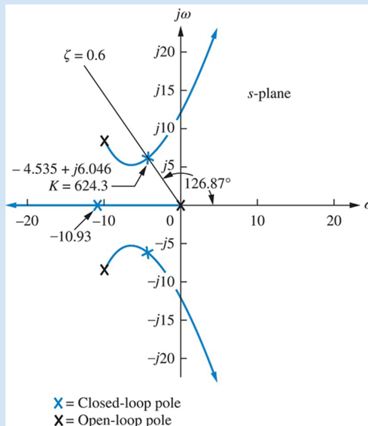
FIGURE 9.57 Root locus for closed-loop system of Example 9.8
