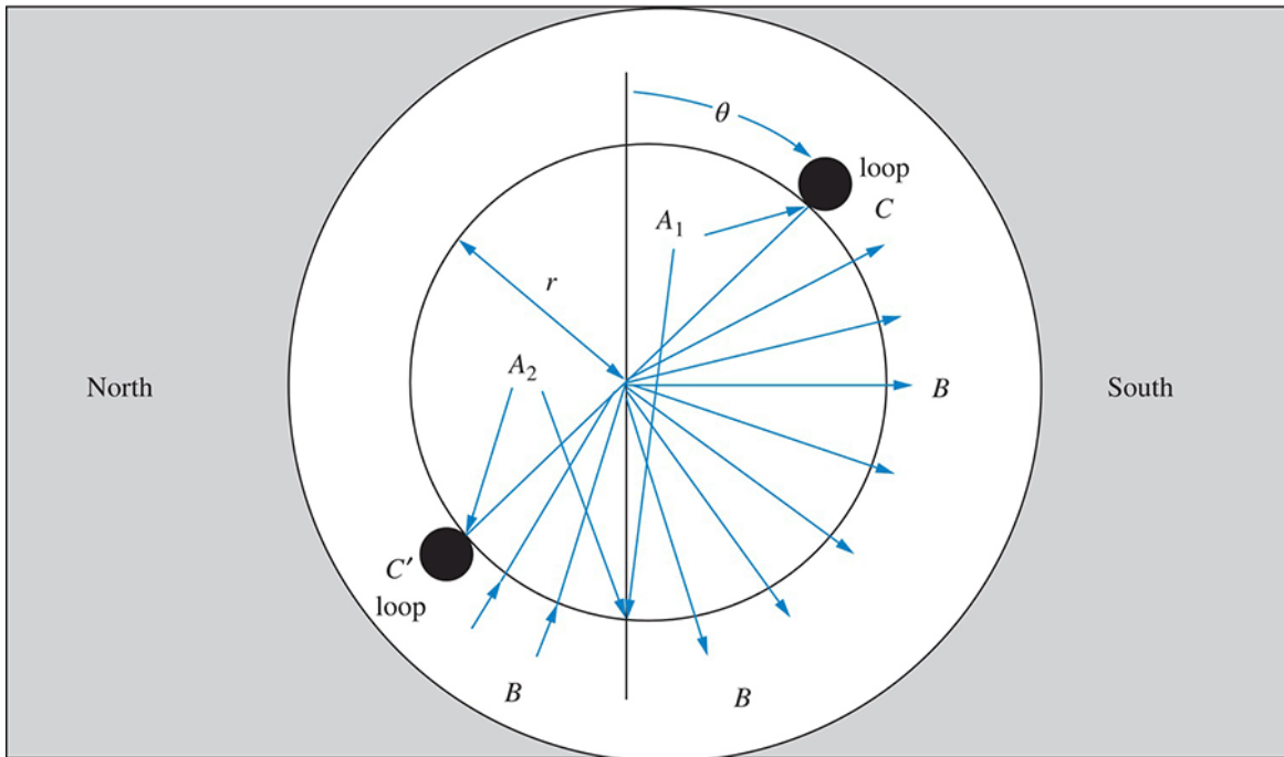
FIGURE I.3 Magnetic flux density passing through a loop of wire on an armature
