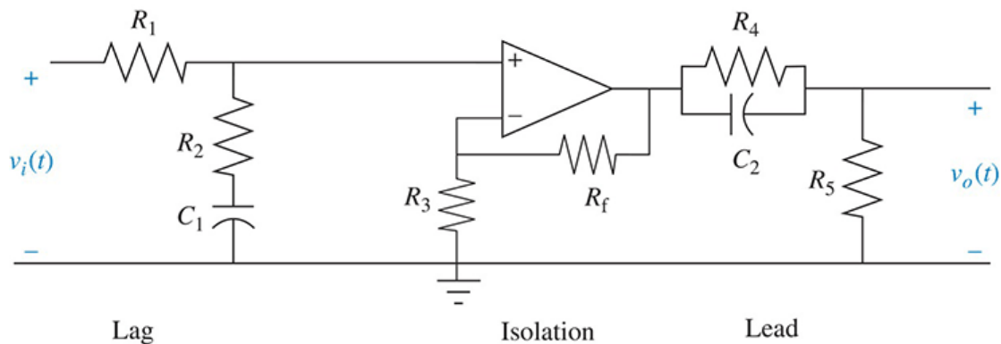
FIGURE 9.63 Lag–lead compensator implemented with cascaded lag and lead networks with isolation
