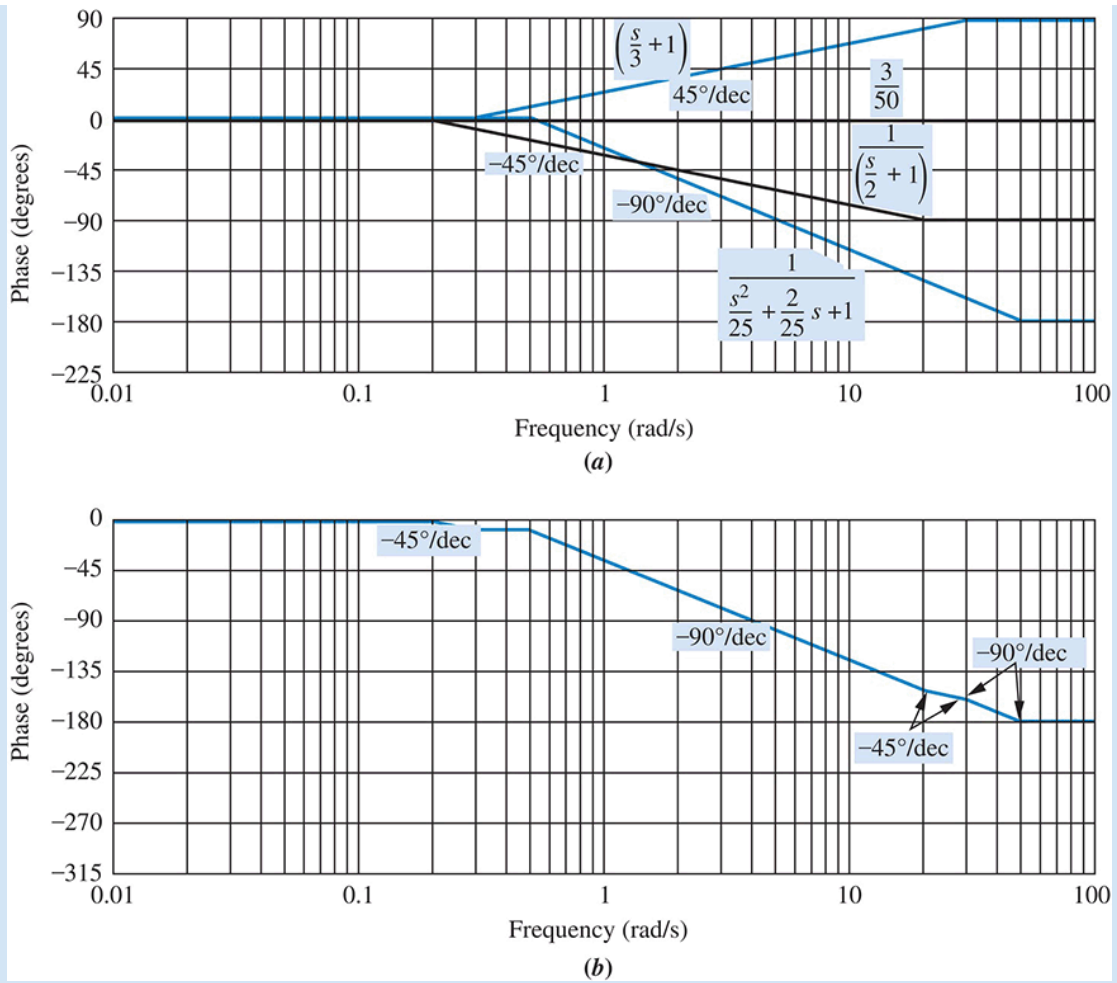
FIGURE 10.19 Bode phase plot for G(s) = (s + 3)/[(s + 2)(s^2 + 2s + 25)] :
