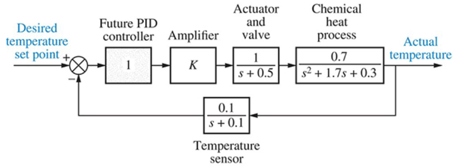
FIGURE P6.11 Block diagram of a chemical process control system
