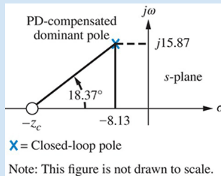
FIGURE 9.33 Calculating the PD compensator zero for Example 9.5
