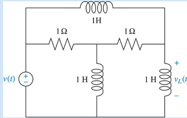
FIGURE 2.14 Electric circuit for Skill-Assessment Exercise 2.6
