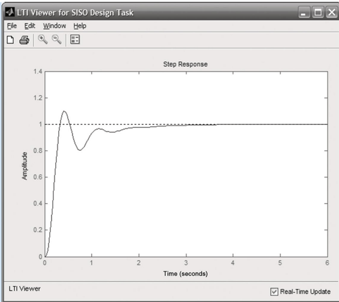
FIGURE 11.16 Lag-lead compensated closed-loop step response
