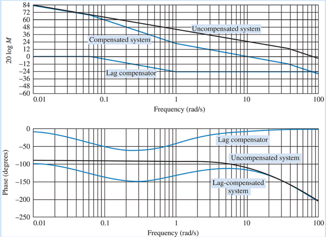
FIGURE 11.6 Bode plots for Example 11.2
