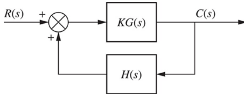
FIGURE 8.26 Positive-feedback system
