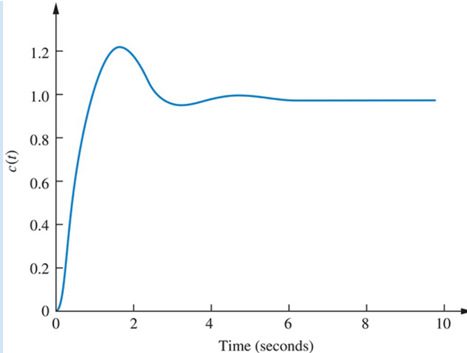
FIGURE 9.69 Step response of lead-compensated UFSS vehicle
