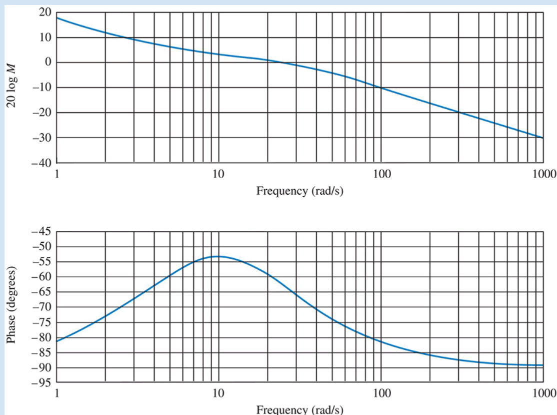
FIGURE 10.60 Bode plots for Skill-Assessment Exercise 10.12
