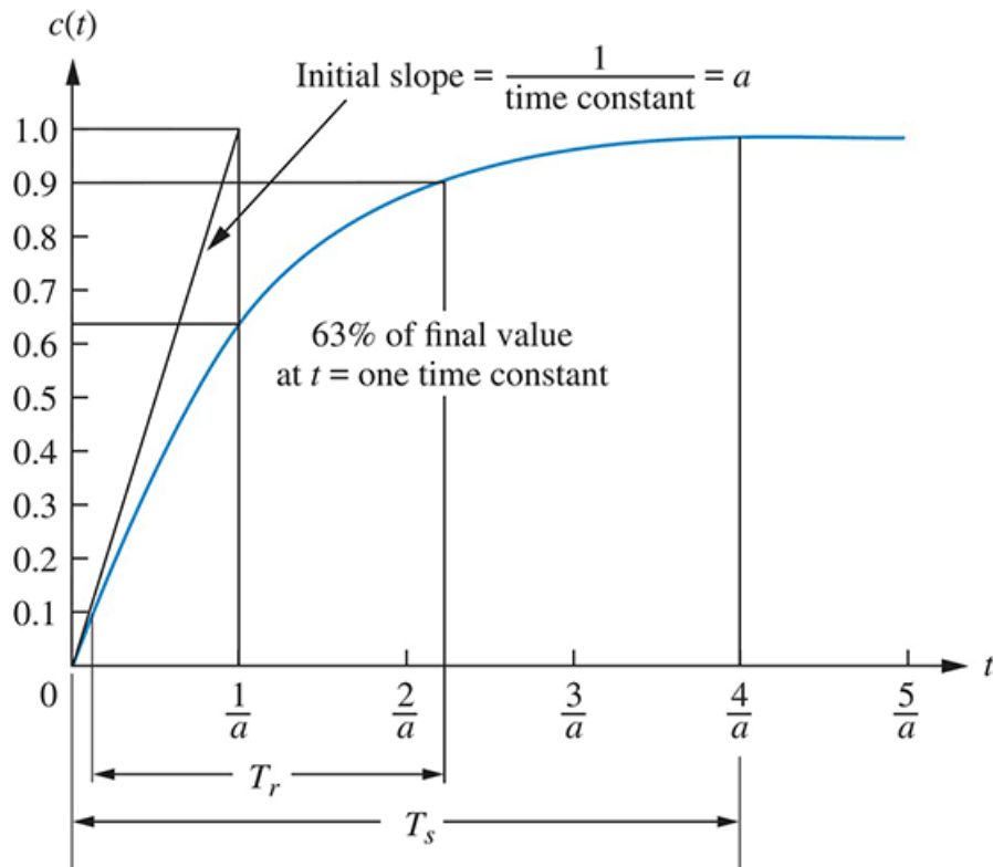
FIGURE 4.5 First-order system response to a unit step
