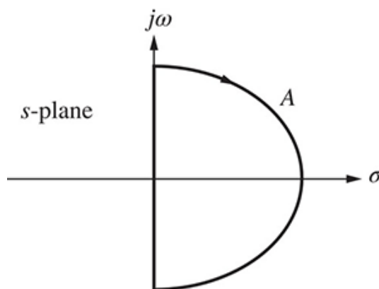
FIGURE 10.24 Contour enclosing right half-plane to determine stability
