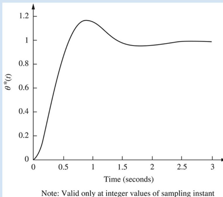
FIGURE 13.35 Closed-loop digital step response for antenna control system with a lead compensator
