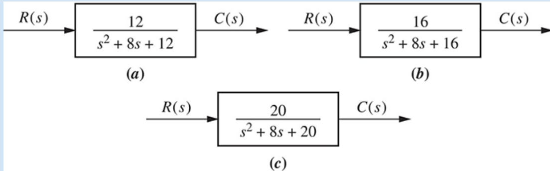
FIGURE 4.12 Systems for Example 4.4 .
