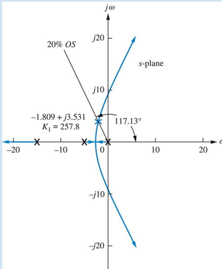
FIGURE 9.50 Root locus for uncompensated system of Example 9.7 .
