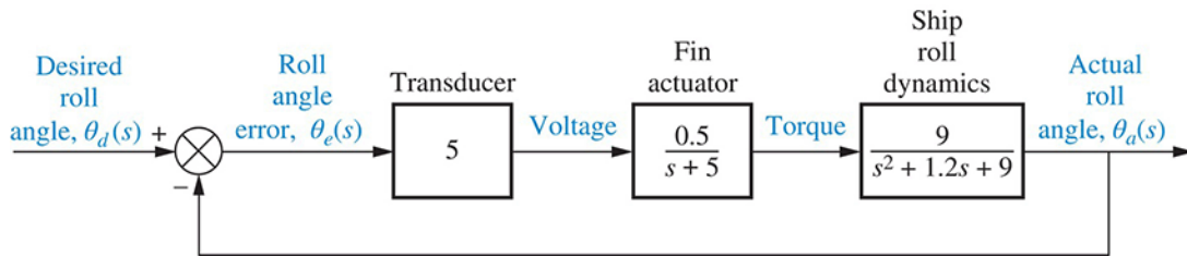
FIGURE P10.11 Block diagram of a ship's roll-stabilizing system
